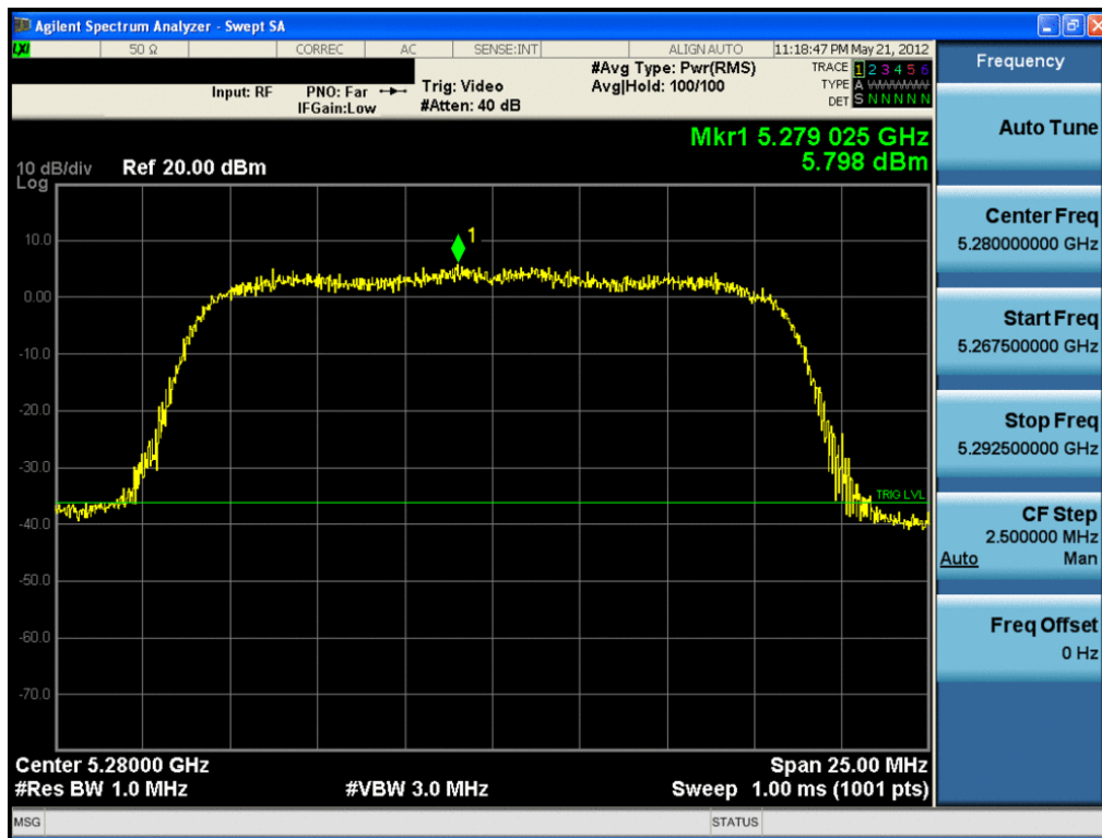
Plot 6-26. Peak Power Spectral Density Plot (802.11a (UNII Band 2) – Ch. 56)
