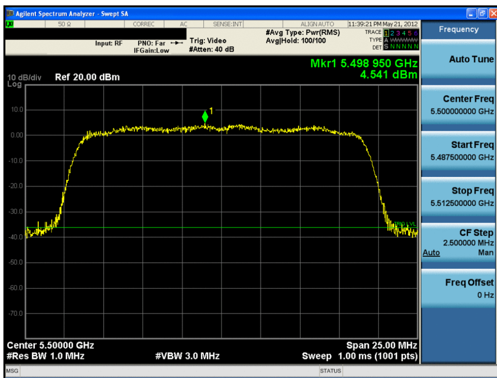
Plot 6-34. Peak Power Spectral Density Plot (802.11n (UNII Band 3) – Ch. 100)
