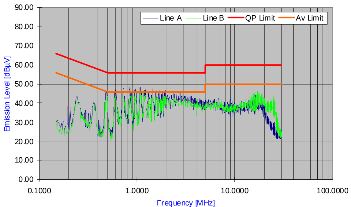
Plot 6-56. Line Conducted Plot with 802.11a (UNII Band 2)
