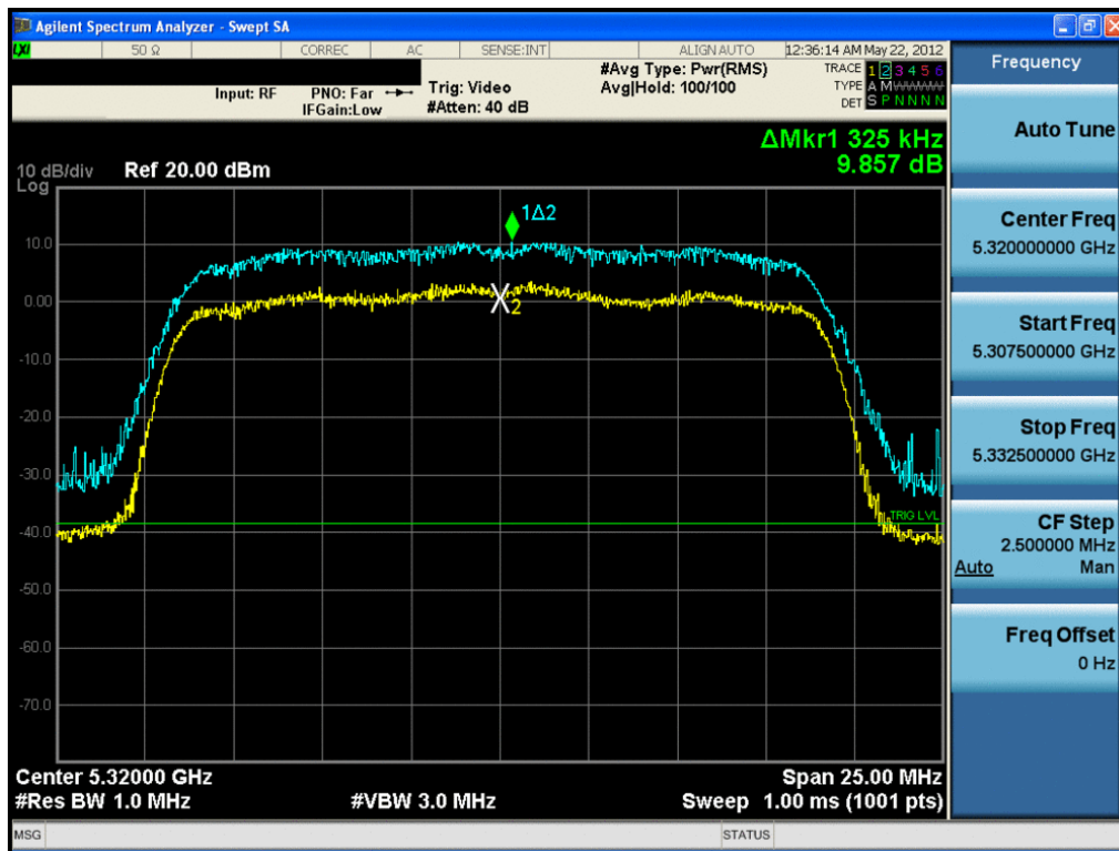
Plot 6-48. Peak Excursion Ratio Plot (802.11n (UNII Band 2) – Ch. 64)
