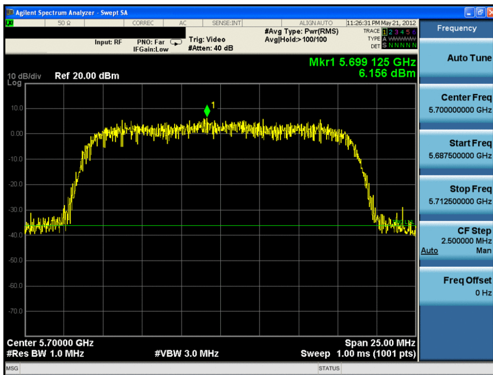
Plot 6-33. Peak Power Spectral Density Plot (802.11a (UNII Band 3) – Ch. 140)
