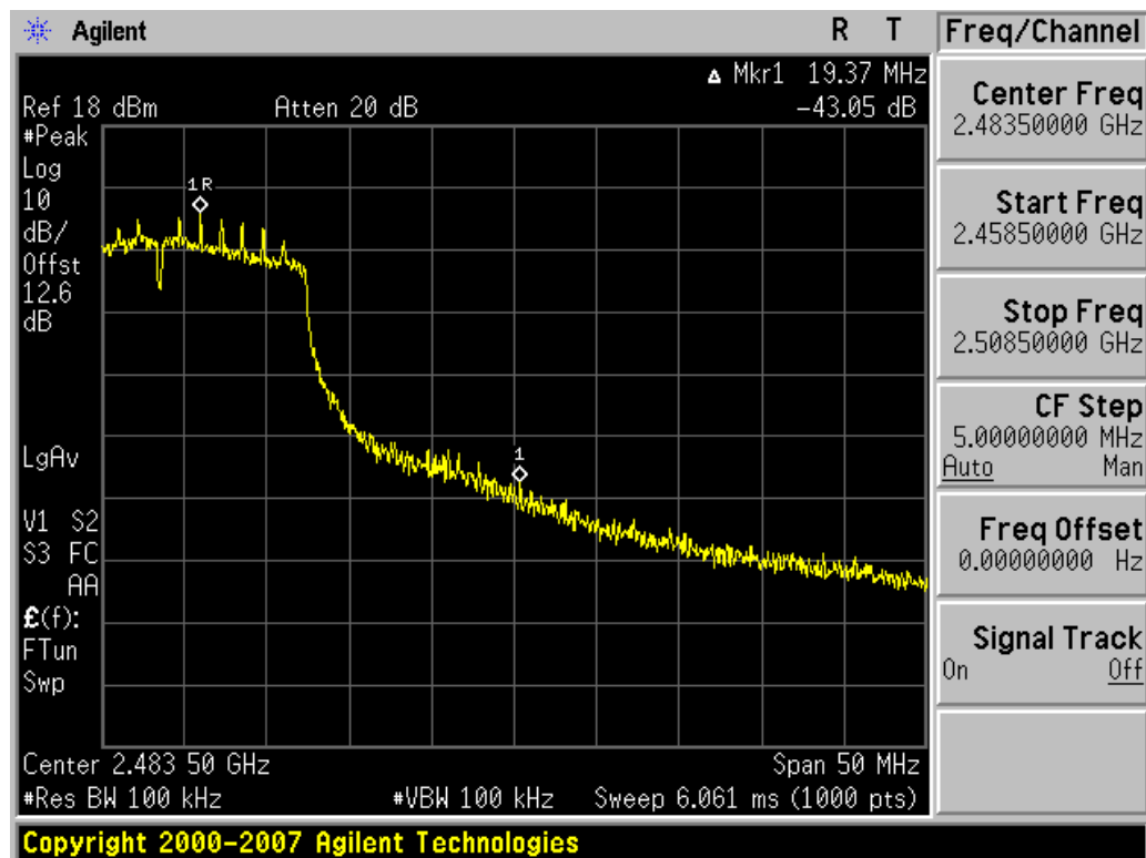
Plot 6-24. Band Edge Plot (802.11n – Ch. 11)
