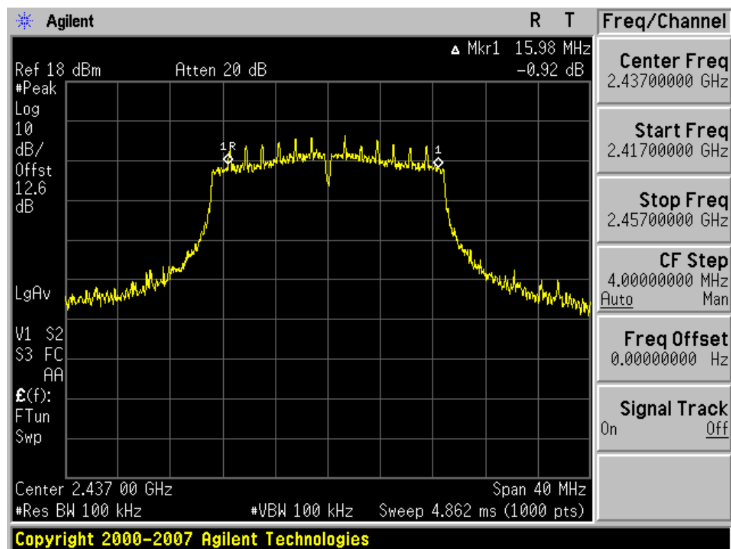
Plot 6-8. 6dB Bandwidth Plot (802.11n – Ch. 6)
