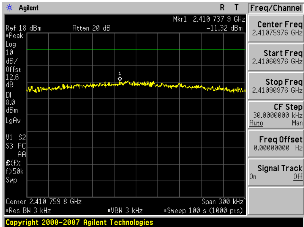
Plot 6-16. Power Spectral Density Plot (802.11n – Ch. 1)
