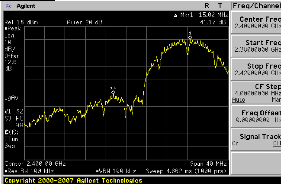
Plot 6-19. Band Edge Plot (802.11b – Ch. 1)
