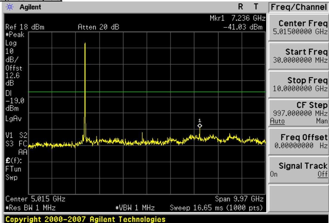
Plot 6-25. Conducted Spurious Plot (802.11b – Ch. 1)
