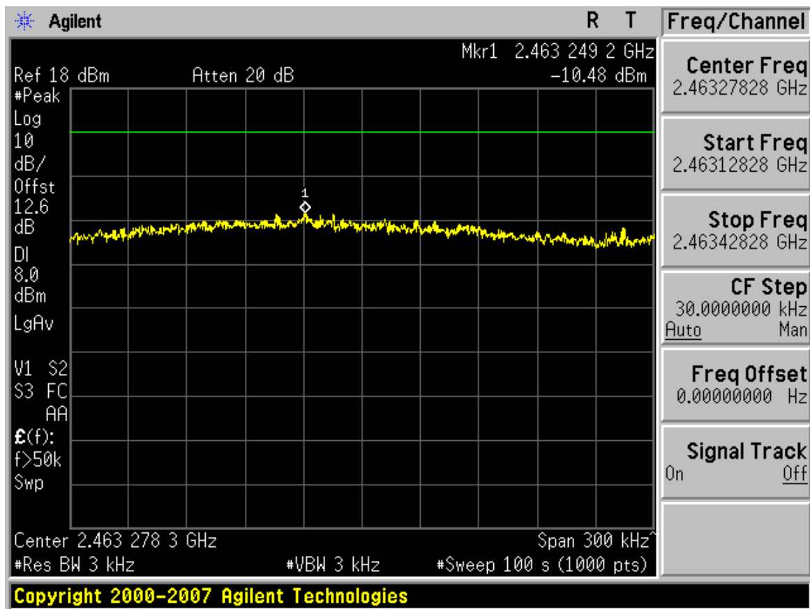
Plot 6-18. Power Spectral Density Plot (802.11n – Ch. 11)
