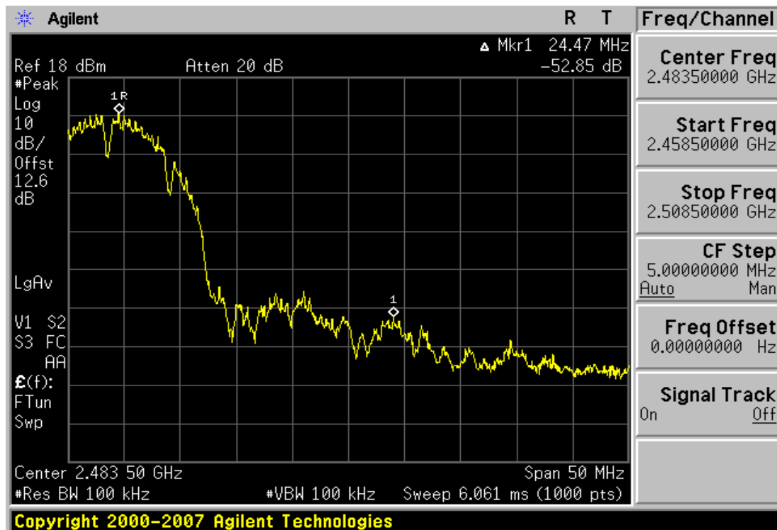
Plot 6-20. Band Edge Plot (802.11b – Ch. 11)
