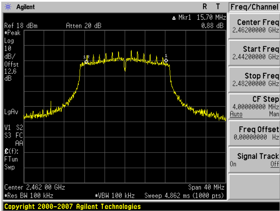
Plot 6-9. 6dB Bandwidth Plot (802.11n – Ch. 11)
