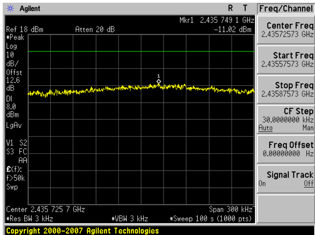
Plot 6-17. Power Spectral Density Plot (802.11n – Ch. 6)
