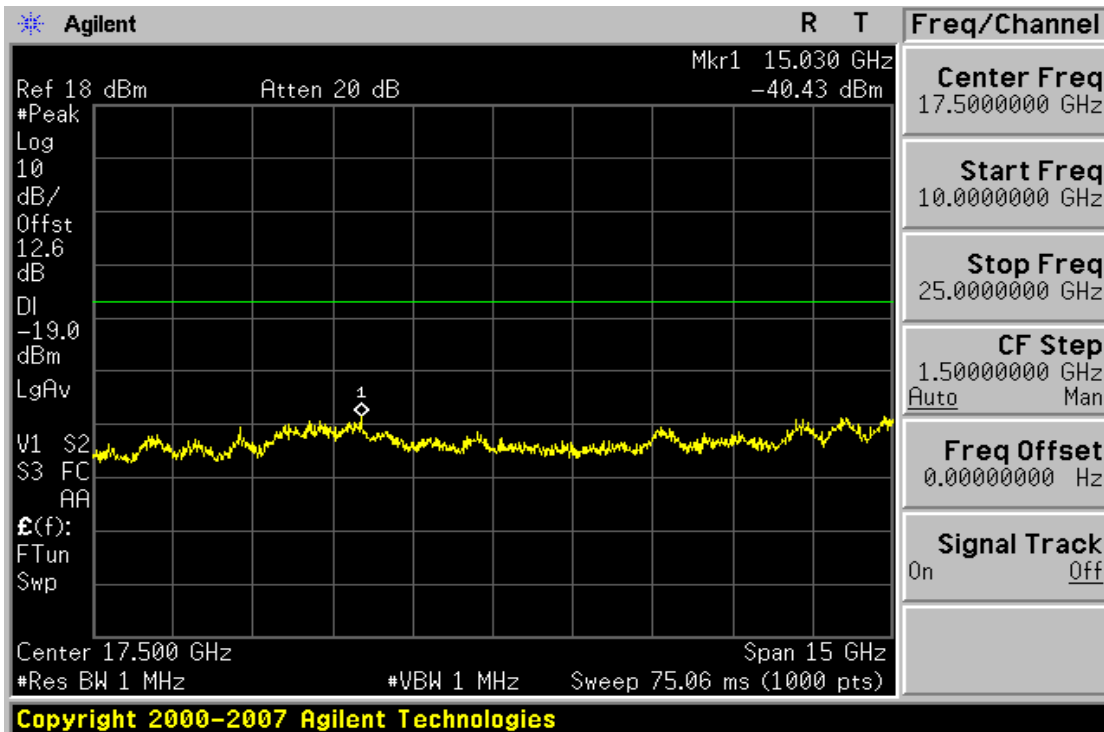
Plot 6-26. Conducted Spurious Plot (802.11b – Ch. 1)
