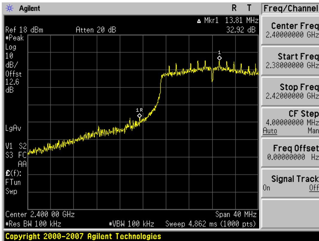
Plot 6-23. Band Edge Plot (802.11n – Ch. 1)
