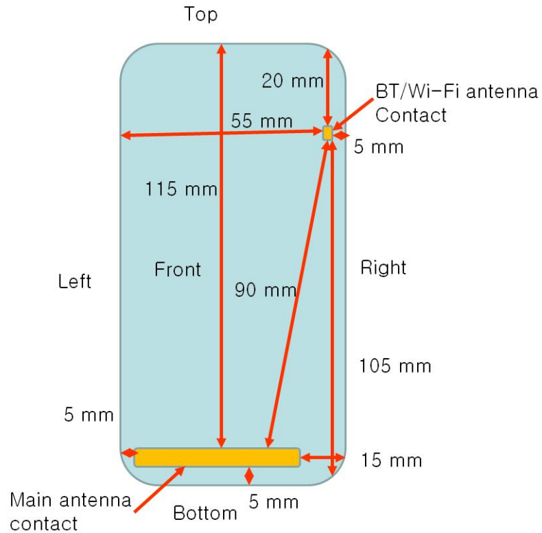
Figure 13-1 Identification of Sides for SAR Testing
