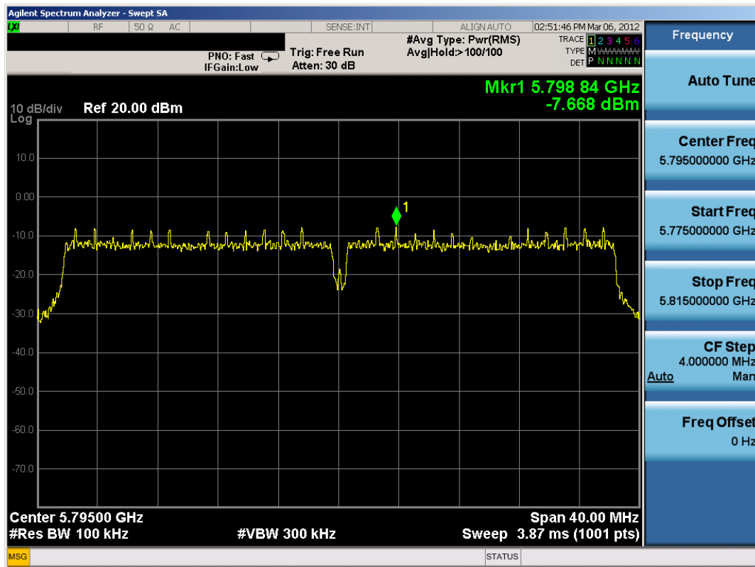
Plot 6-34. Power Spectral Density Plot (802.11n (5.8GHz, 40MHz) – Ch. 159)
