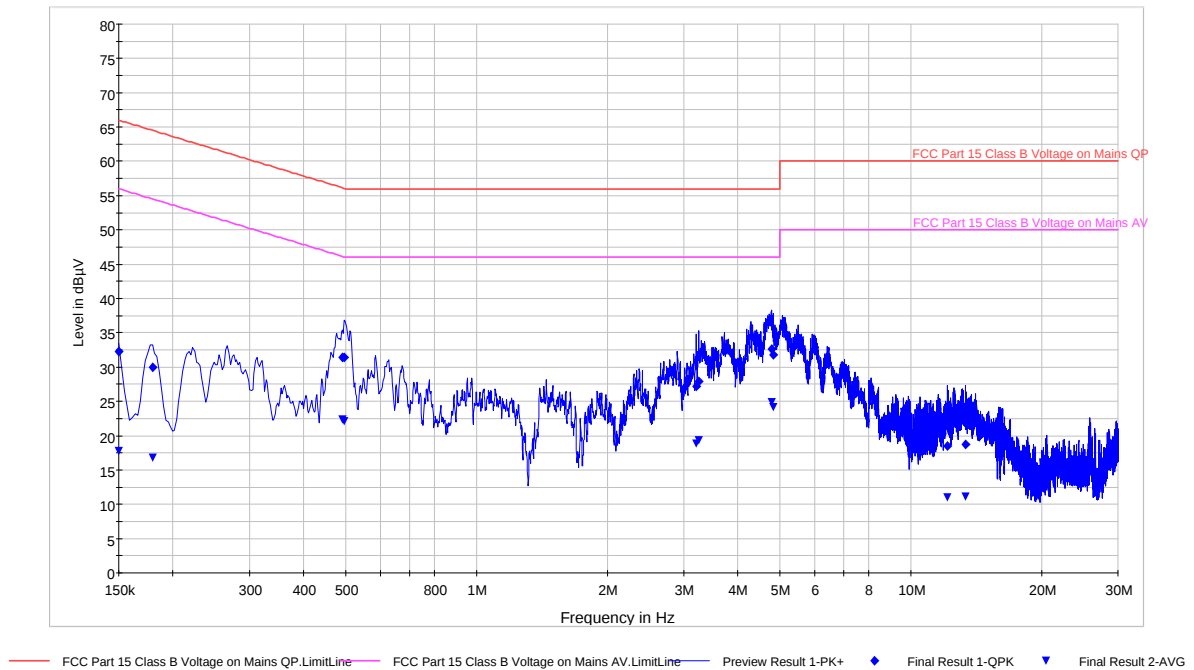
Plot 6-64. Line Conducted Plot with 802.11a – Line 1
