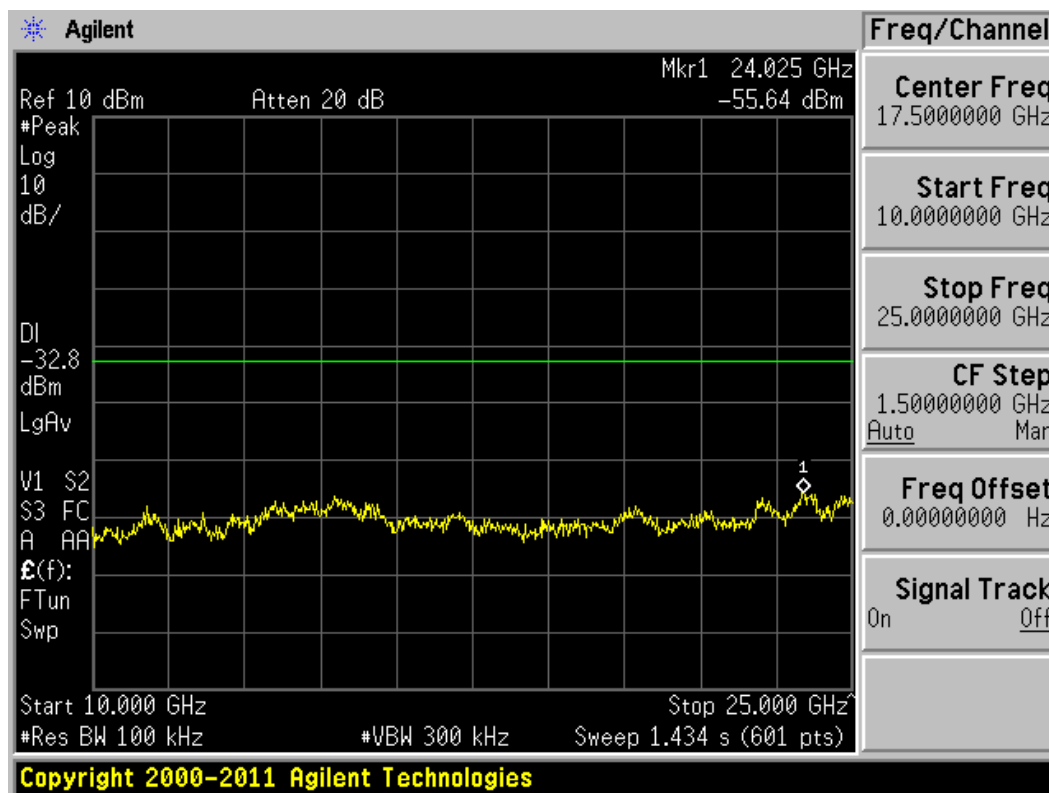
Plot 6-54. Conducted Spurious Plot (802.11a – Ch. 149)
