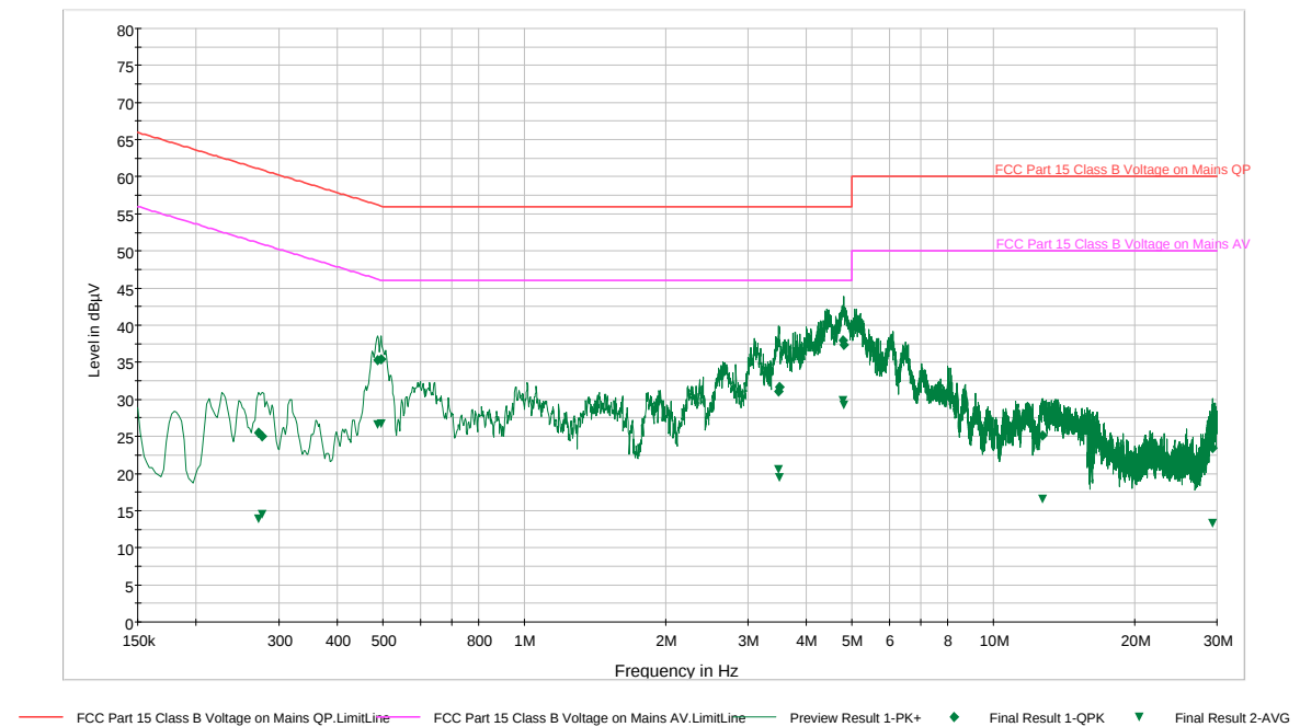
Plot 6-65. Line Conducted Plot with 802.11a – Line N
