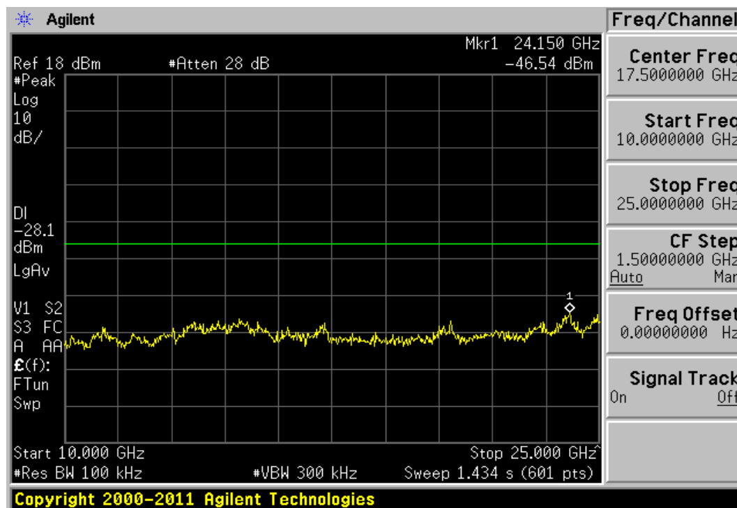
Plot 6-52. Conducted Spurious Plot (802.11b – Ch. 11)
