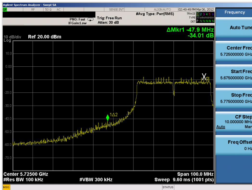
Plot 6-45. Band Edge Plot (802.11n (5.8GHz, 40MHz) – Ch. 151)
