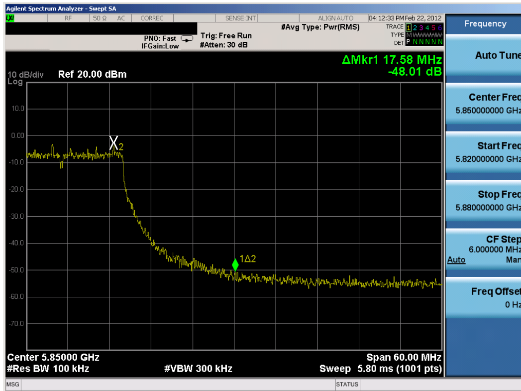
Plot 6-44. Band Edge Plot (802.11n (5.8GHz) – Ch. 165)
