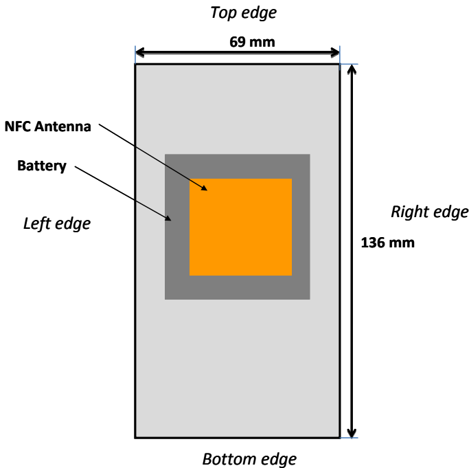
Figure 1-2 NFC Antenna Locations
