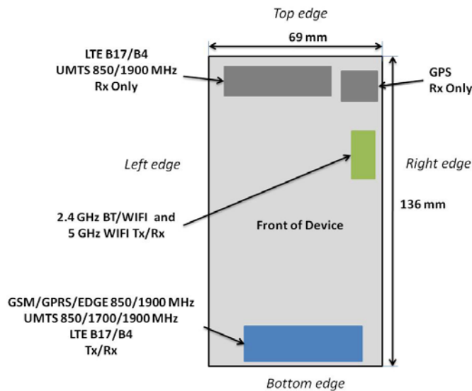
Figure 1-1 DUT Antenna Locations
