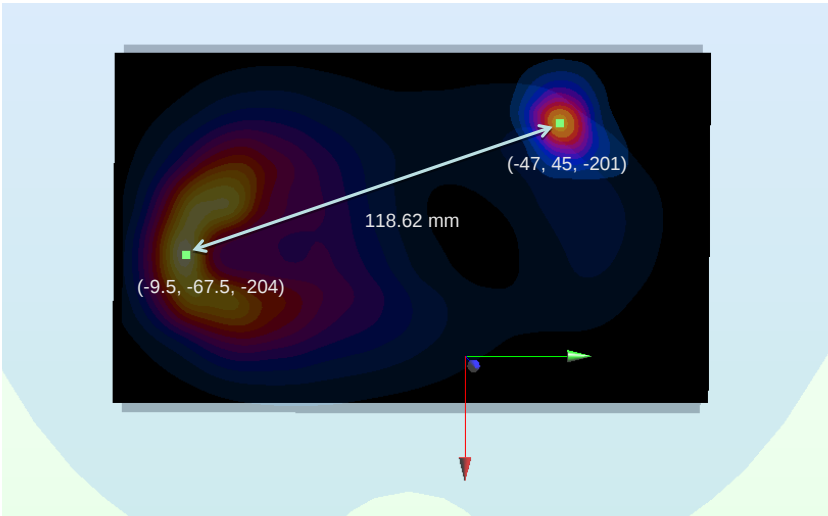
Figure 12-1 Peak SAR Location Plot of UMTS 1900 and 5 GHz WLAN
