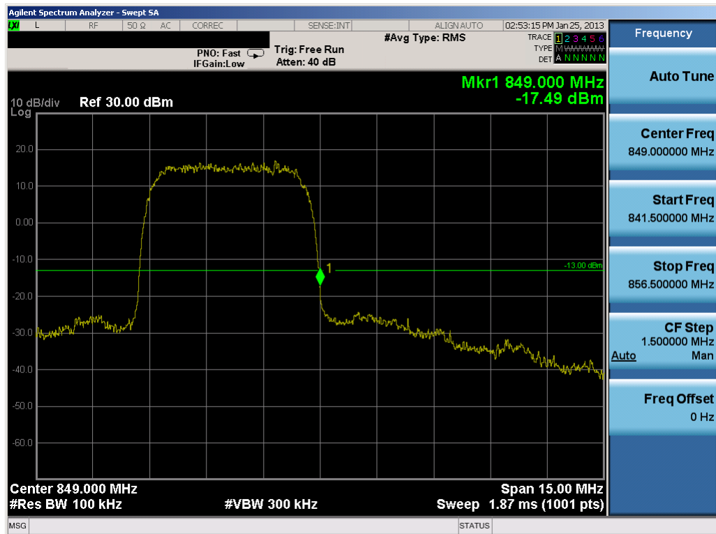
Plot 7-31. Band Edge Plot (Cellular WCDMA Mode – Ch. 4233)
