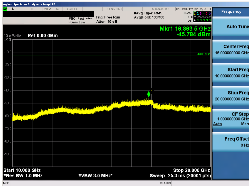
Plot 7-33. Conducted Spurious Plot (AWS WCDMA Mode – Ch. 1312)
