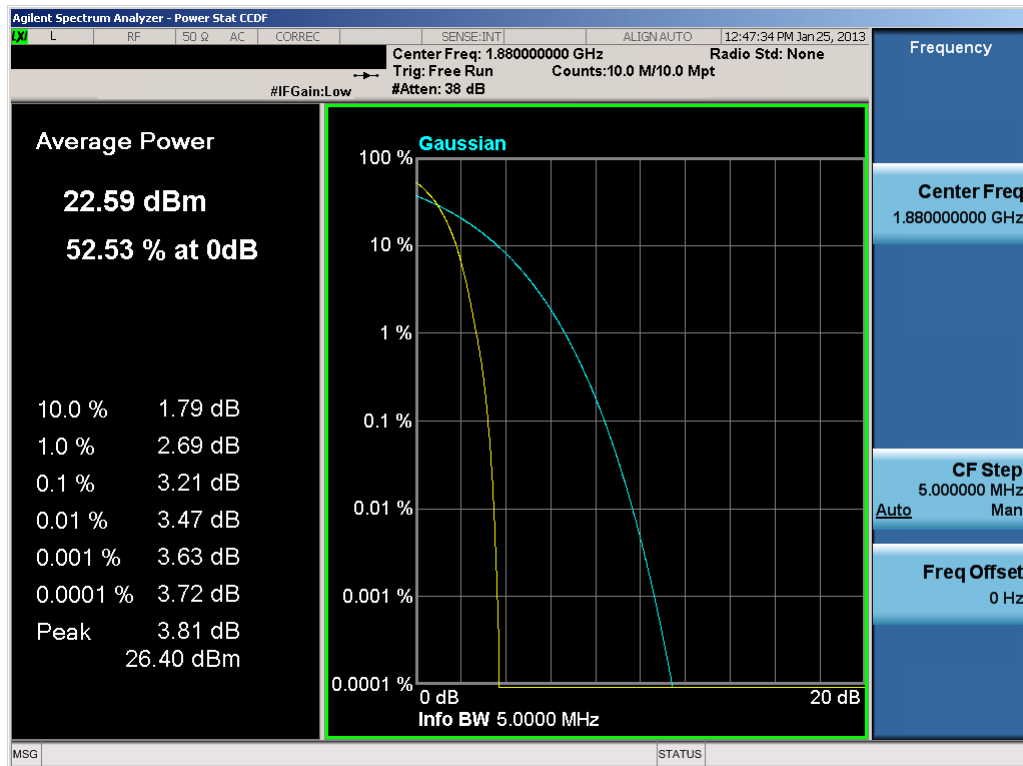
Plot 7-51. Peak-Average Ratio Plot (PCS WCDMA Mode – Ch. 9400)
