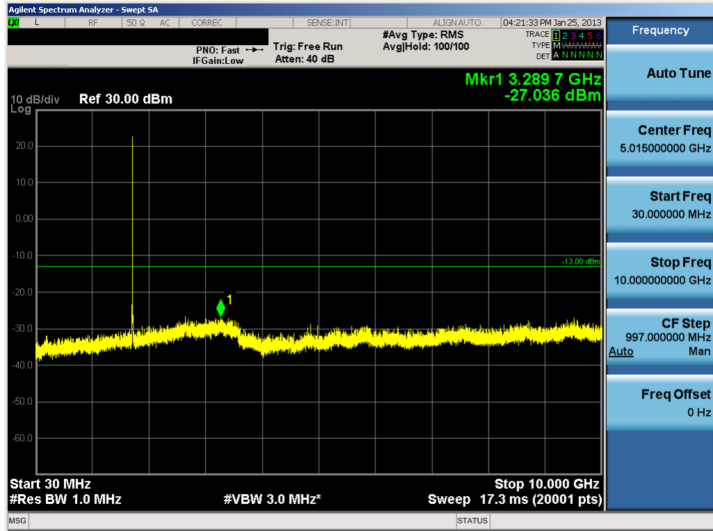
Plot 7-36. Conducted Spurious Plot (AWS WCDMA Mode – Ch. 1412)
