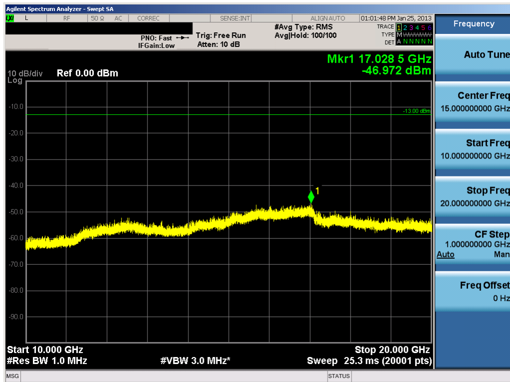
Plot 7-53. Conducted Spurious Plot (PCS WCDMA Mode – Ch. 9538)
