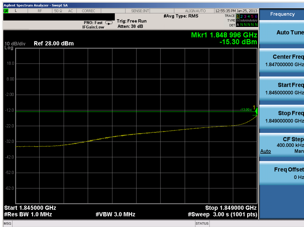
Plot 7-47. 4MHz Span Plot (PCS WCDMA Mode – Ch. 9262)
