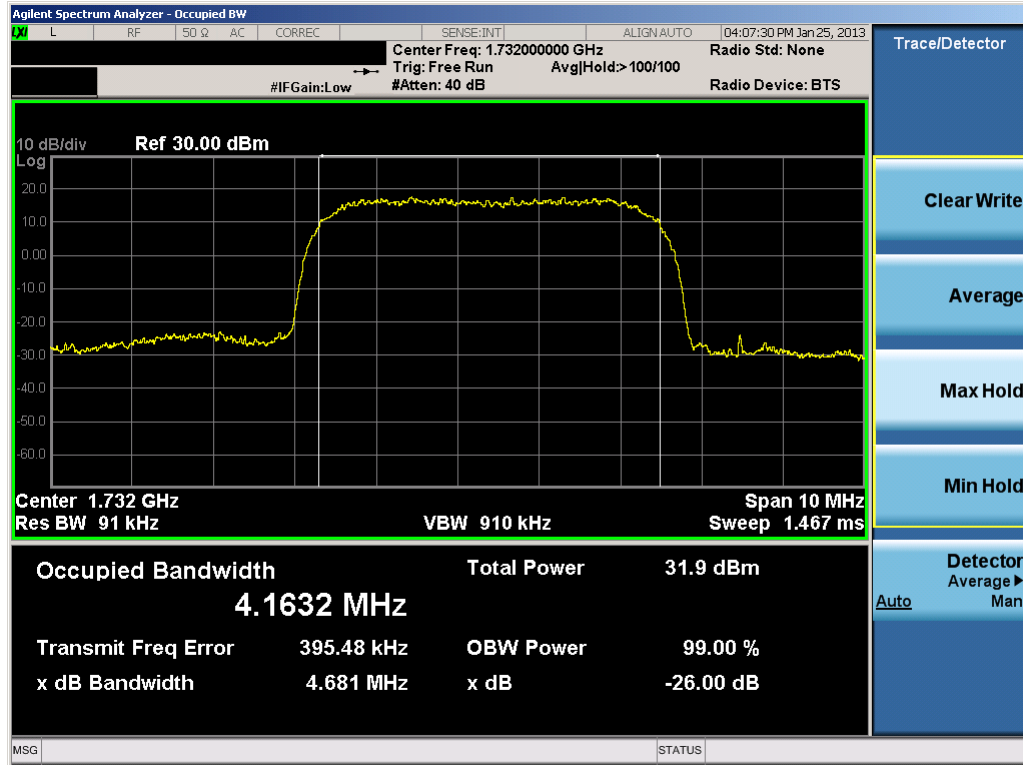
Plot 7-38. Occupied Bandwidth Plot (AWS WCDMA Mode – Ch. 1412)
