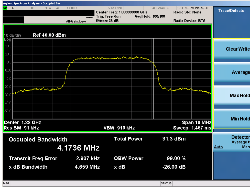
Plot 7-50. Occupied Bandwidth Plot (PCS WCDMA Mode – Ch. 9400)
