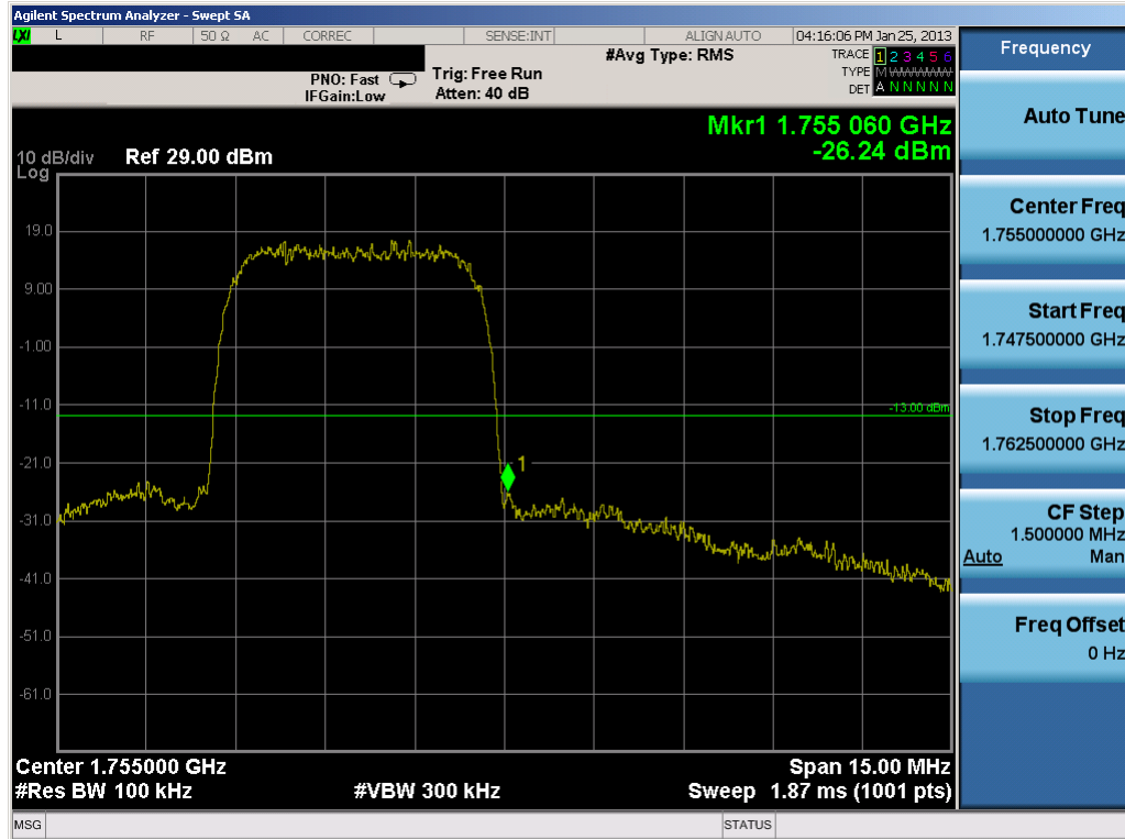
Plot 7-42. Band Edge Plot (AWS WCDMA Mode – Ch. 1862)
