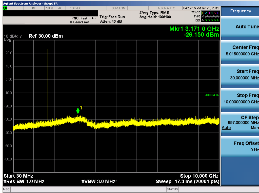
Plot 7-32. Conducted Spurious Plot (AWS WCDMA Mode – Ch. 1312)
