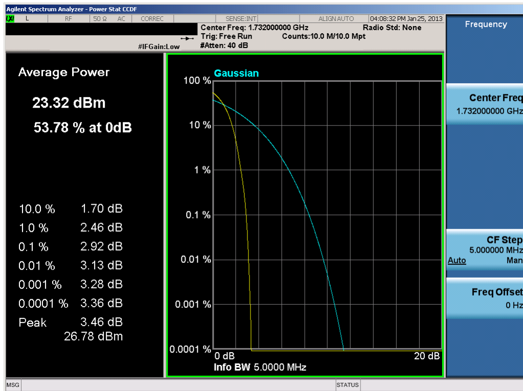
Plot 7-39. Peak-Average Ratio Plot (AWS WCDMA Mode – Ch. 1412)
