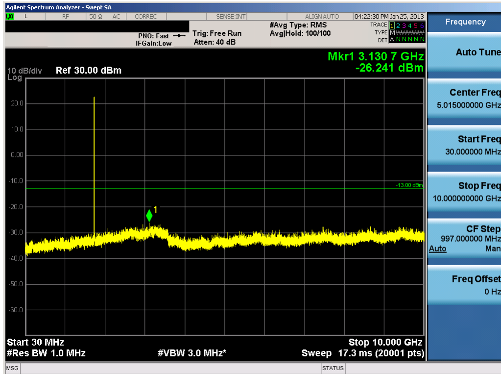
Plot 7-40. Conducted Spurious Plot (AWS WCDMA Mode – Ch. 1862)
