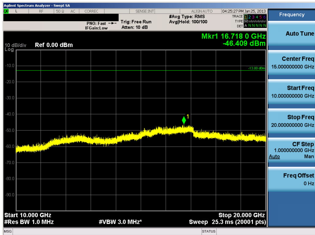
Plot 7-37. Conducted Spurious Plot (AWS WCDMA Mode – Ch. 1412)
