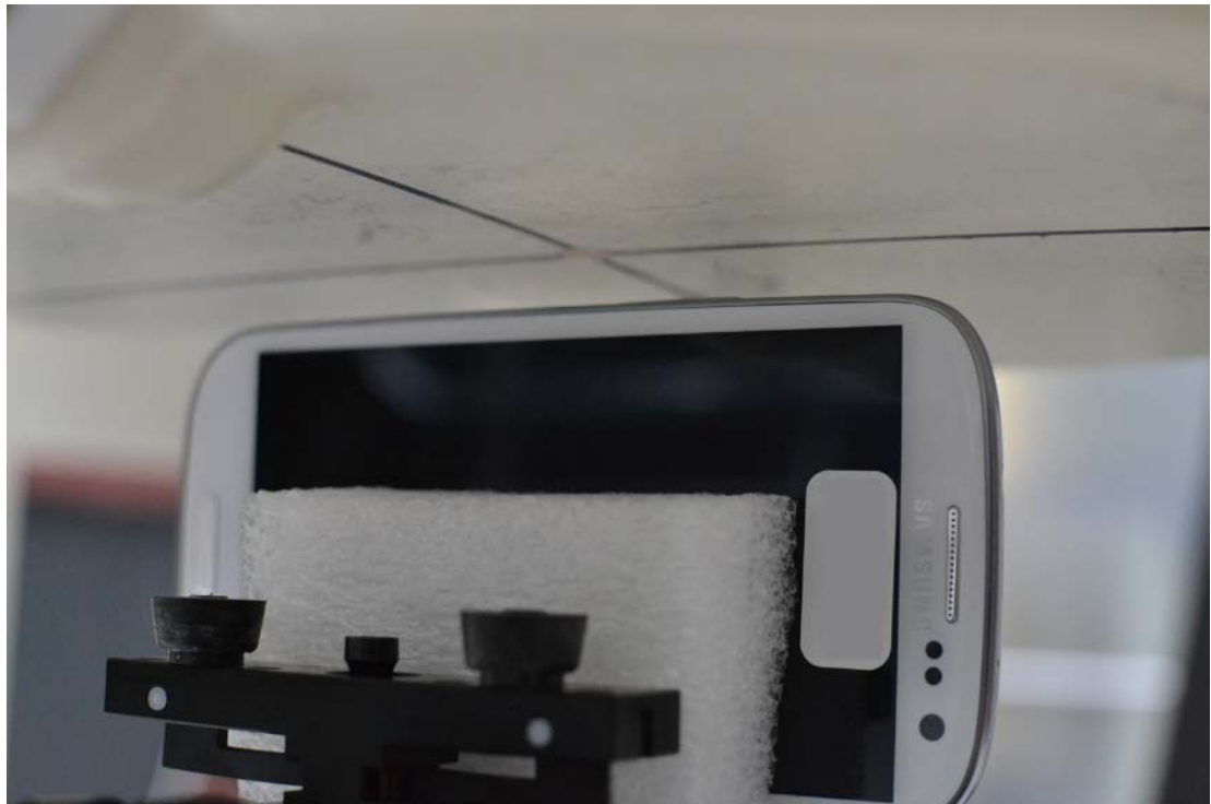
SAR Test Setup 10: Left Edge at 10 mm
