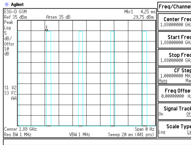
Figure 26 GSM Signal
