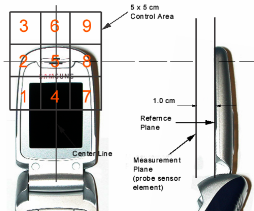
Figure 13 E/H-Field Emissions Test Setup Diagram
