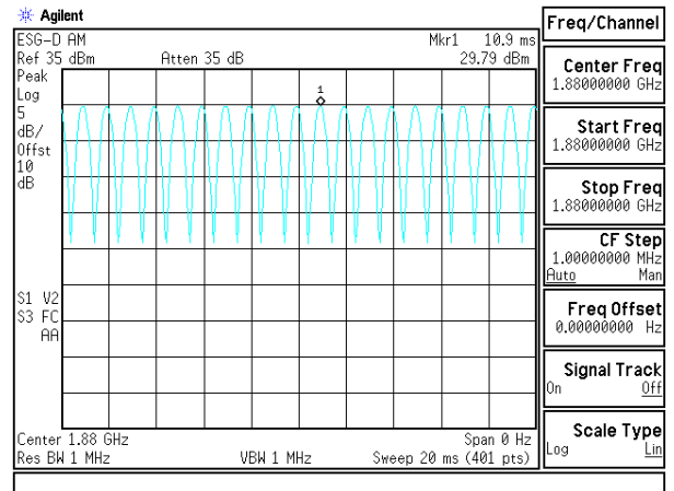
Figure 25 80% AM Signal
