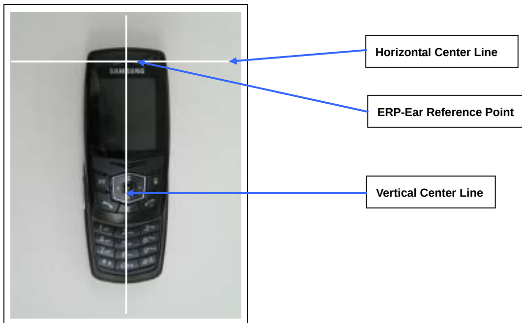
Figure 8.1 Handset Reference Points
