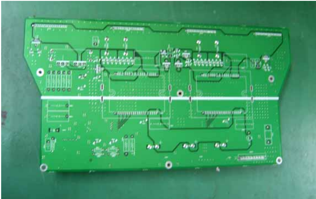
Y driver board top view
