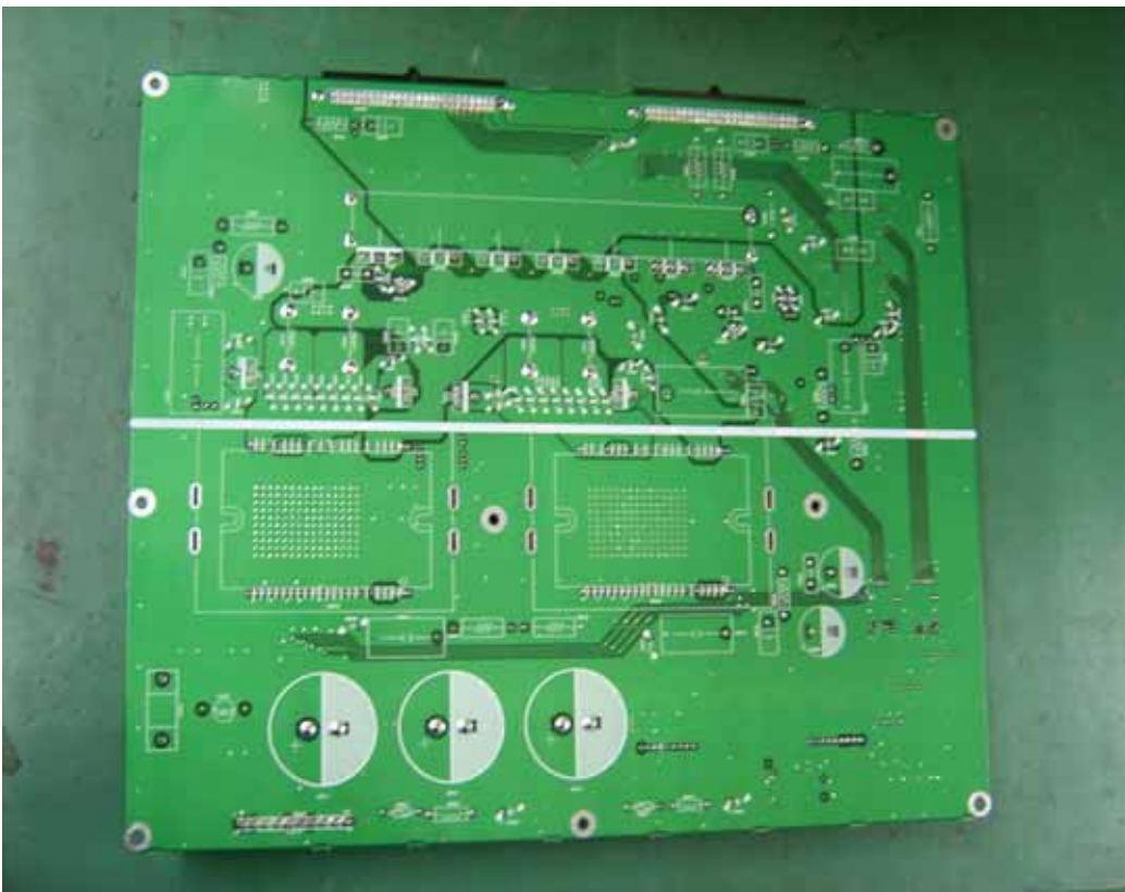
X driver board top view
