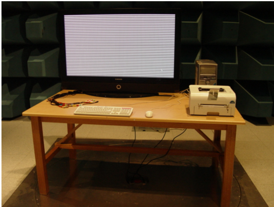
Picture 3. Radiated Emission (Front view)
