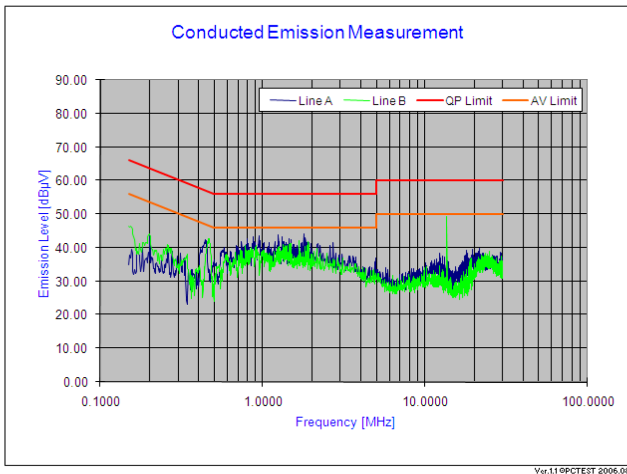
Plot 8-1. Line-Conducted Test Plot
