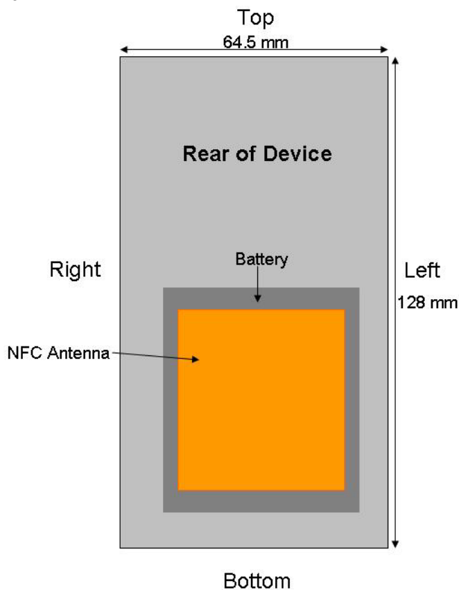
Figure 1-1 NFC Antenna Locations
