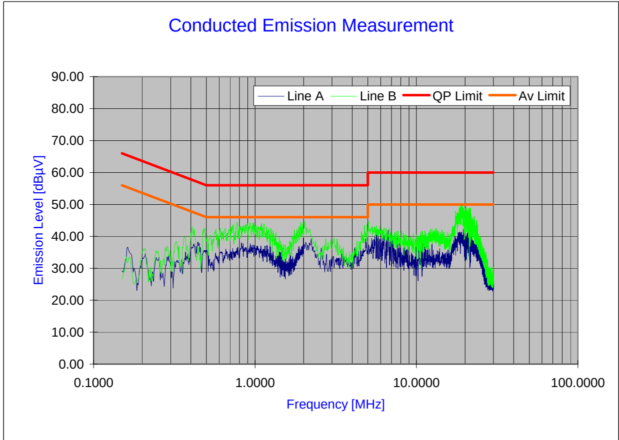
Plot 6-54. Line Conducted Plot with 802.11a
