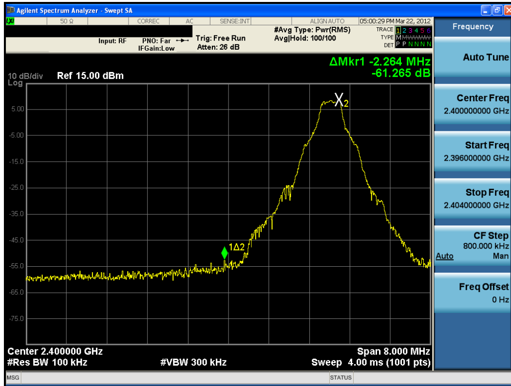
Plot 6-1. Band Edge Plot (Bluetooth (LE) – Ch. 0)
