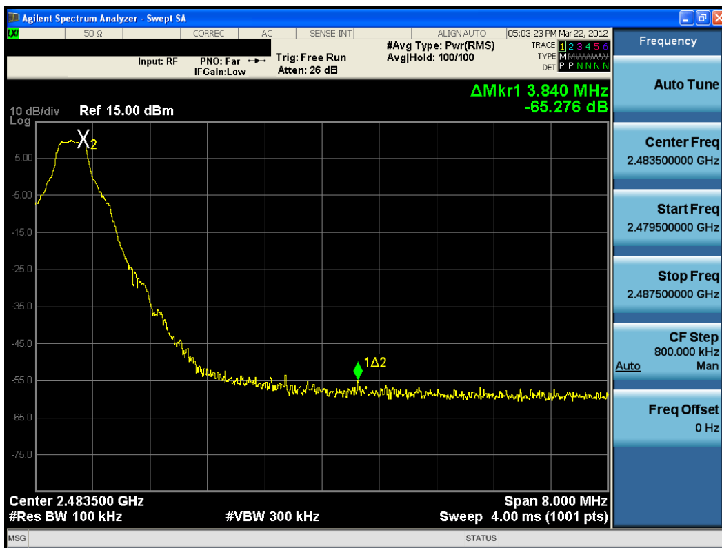
Plot 6-2. Band Edge Plot (Bluetooth (LE) – Ch. 39)
