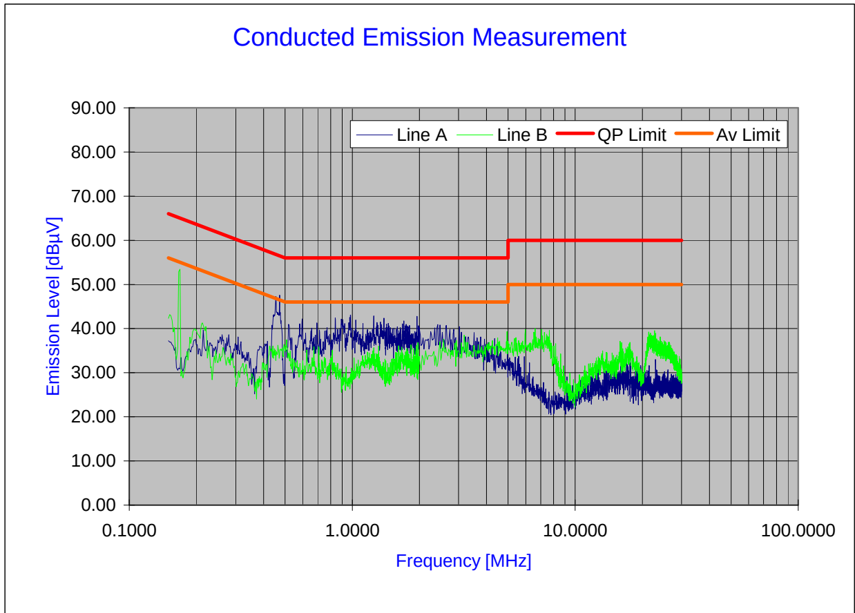
Plot 6-3. Line Conducted Plot with Bluetooth (LE)
