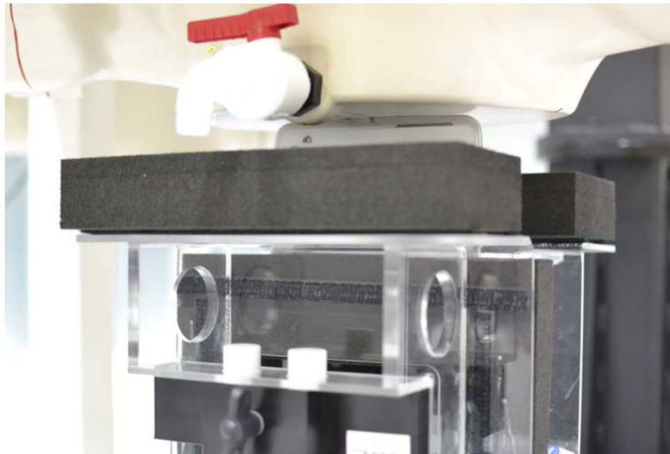
SAR Test Setup Photo 4: Left Edge at 0.0 cm
