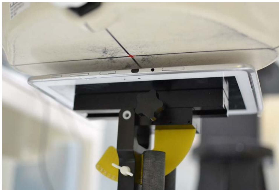
SAR Test Setup Photo 1: Back Side at 1.1 cm
