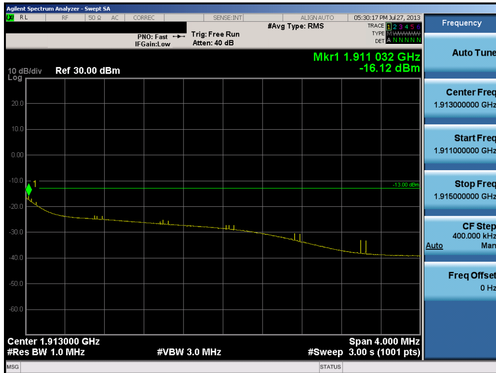
Plot 6-20. 4MHz Span Plot (PCS WCDMA Mode – Ch. 9538)
