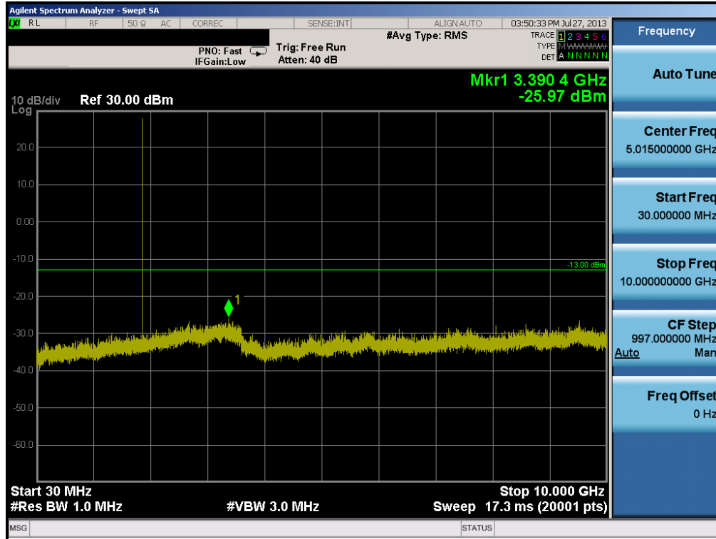
Plot 6-5. Conducted Spurious Plot (PCS GSM Mode – Ch. 661)
