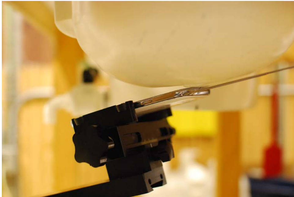
SAR Test Setup Photo 8 - Left Tilt Antenna Extended
