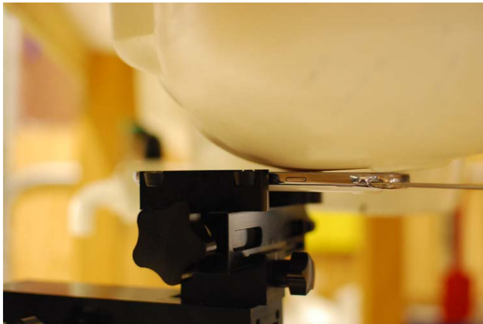
SAR Test Setup Photo 6 - Left Cheek Antenna Extended
