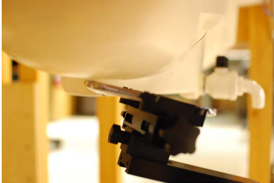
SAR Test Setup Photo 3 - Right Tilt Antenna Retracted
