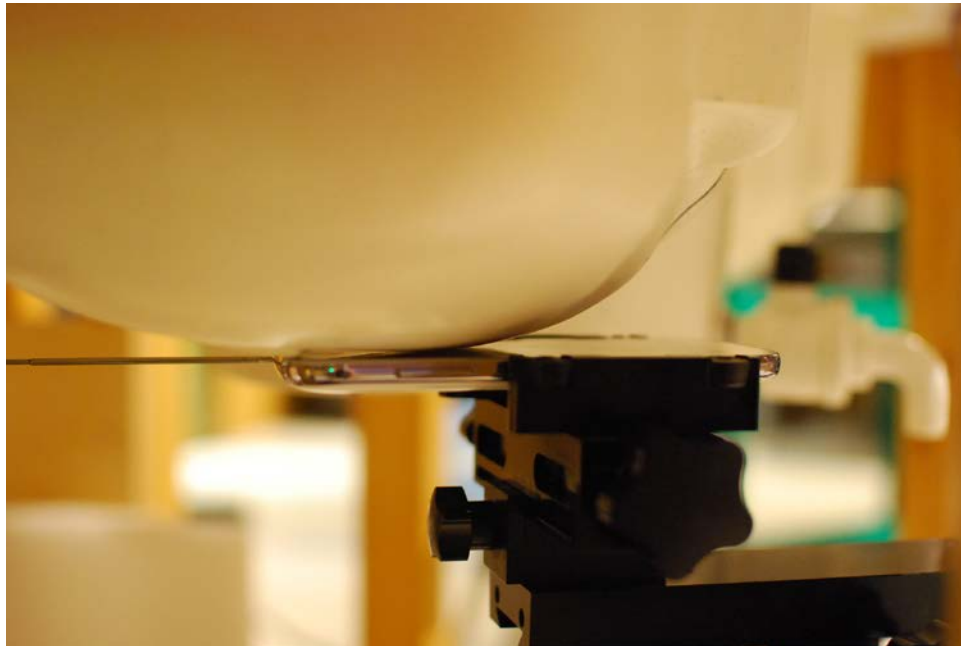
SAR Test Setup Photo 2 - Right Cheek Antenna Extended
