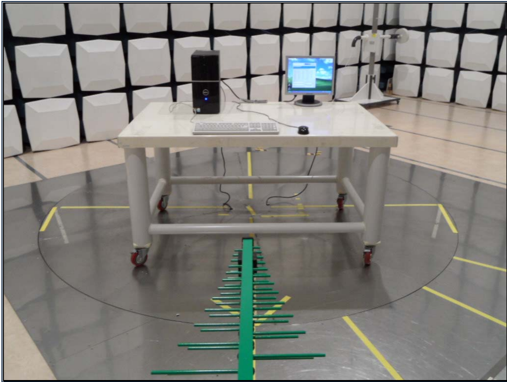
[ Radiated Disturbance – Front ]
