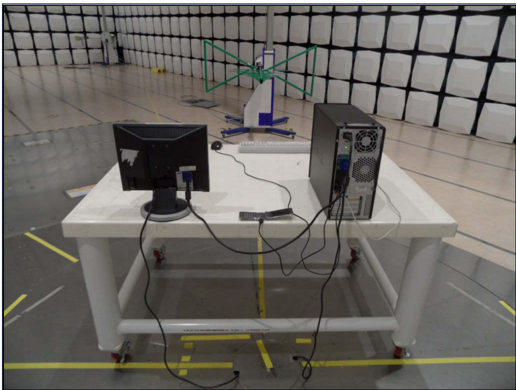
[ Radiated Disturbance – Rear ]
