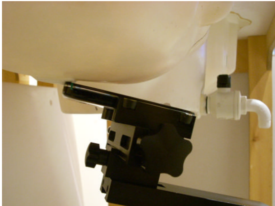
Figure 18-2 SAR Test Setup Photo 2
