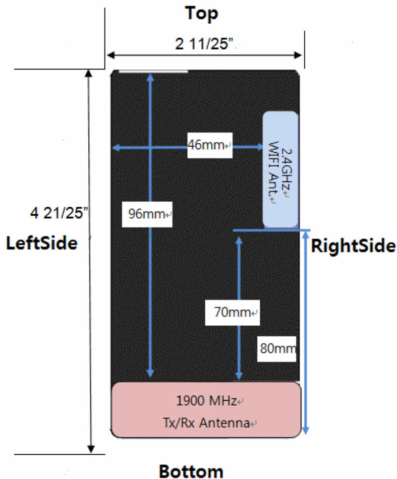
Figure 5.9 Antenna Locations, as viewed from Front of device
