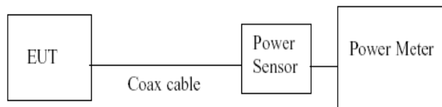
Figure 6-4. Test Instrument & Measurement Setup
