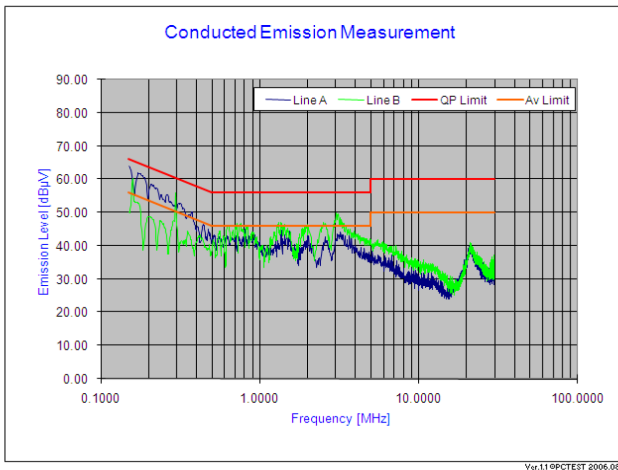
Plot 6-31. Line Conducted Plot with 802.11b
