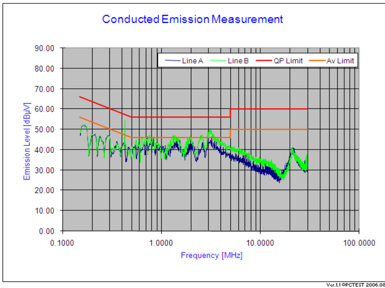
Plot 6-33. Line Conducted Plot with 802.11n
