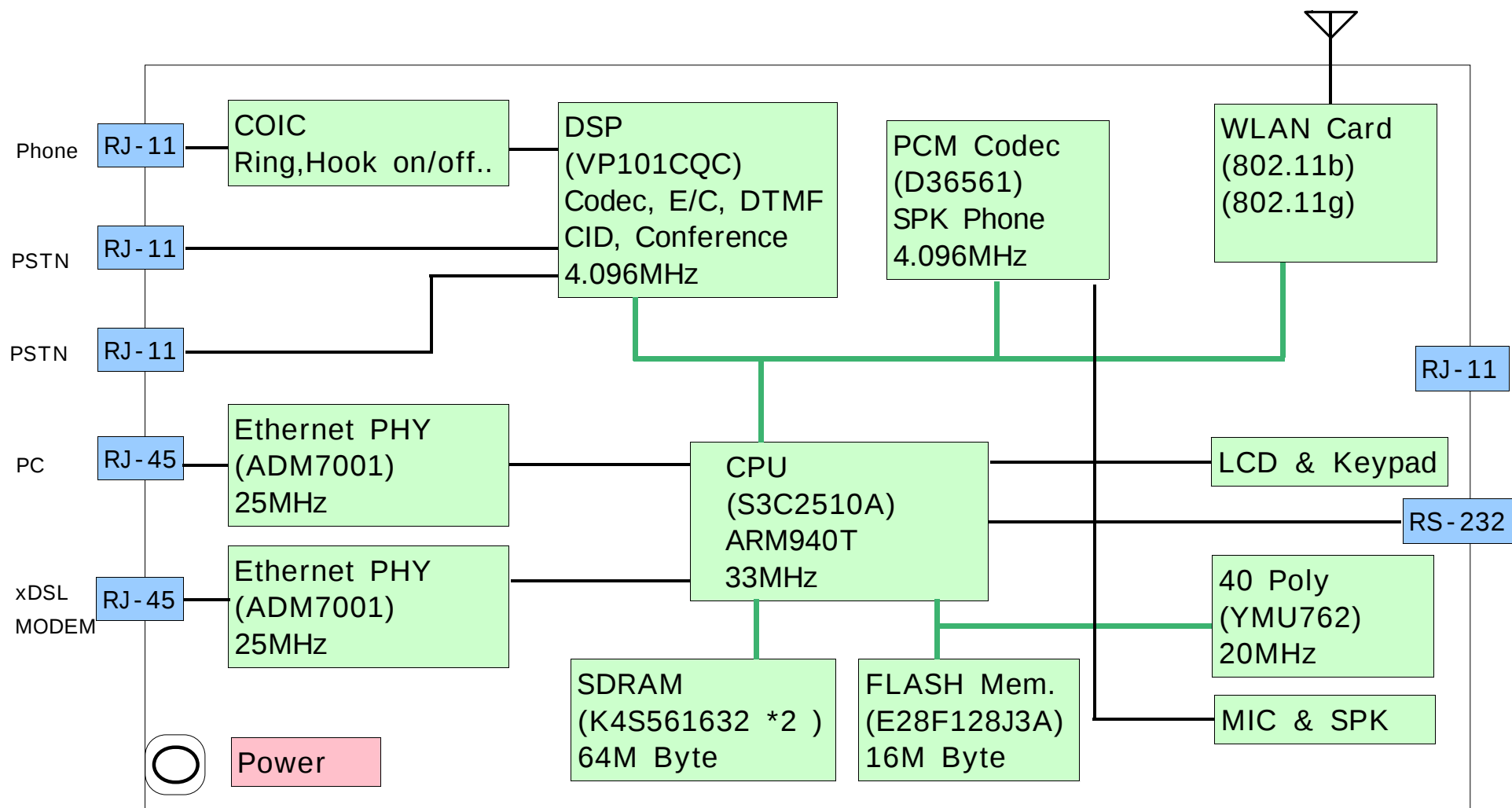
SIT200EMRB Block diagram
