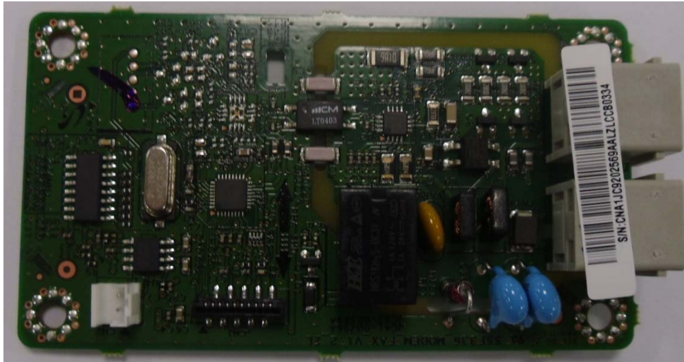
FAX PBA TOP SIDE
