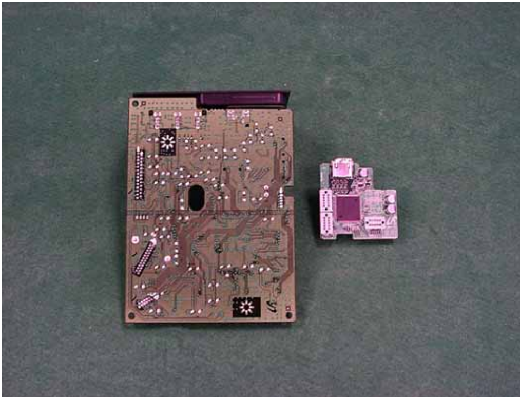
BOTTOM OF DVD PCB VIEW
