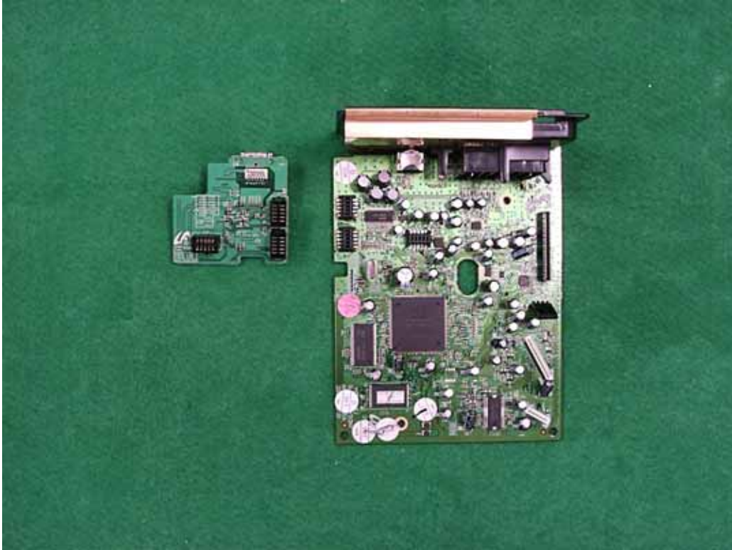
TOP OF DVD PCB VIEW
