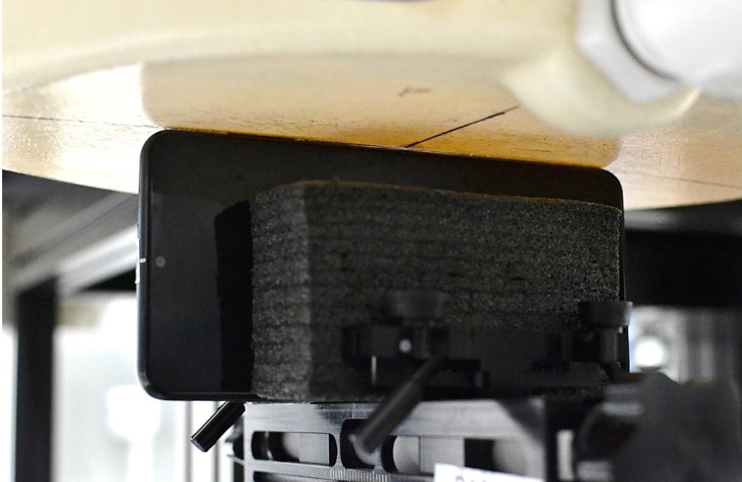
SAR Test Setup Photo 17 – Phablet, Right Edge at 0 mm
