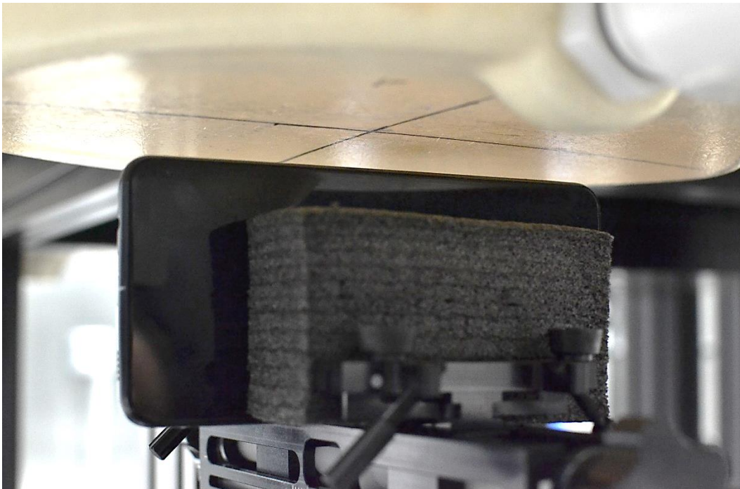
SAR Test Setup Photo 18 – Phablet, Left Edge at 11 mm
