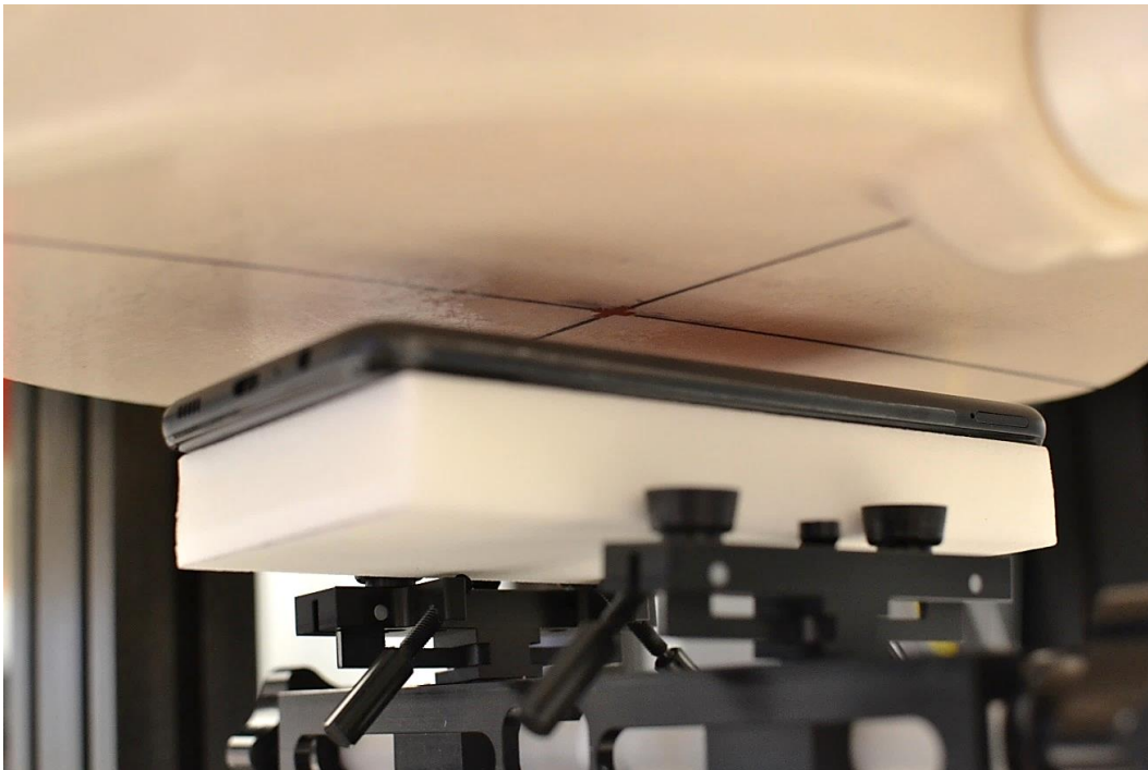
SAR Test Setup Photo 6 – Phablet, Back Side at 14 mm
