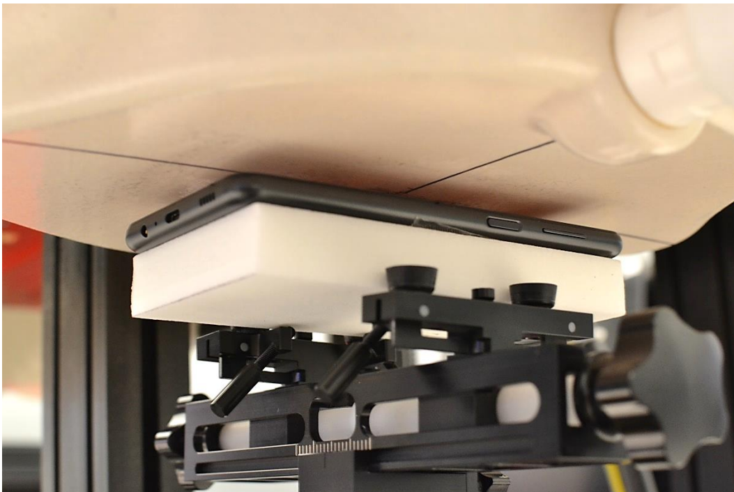
SAR Test Setup Photo 10 – Hotspot, Front Side at 10 mm
