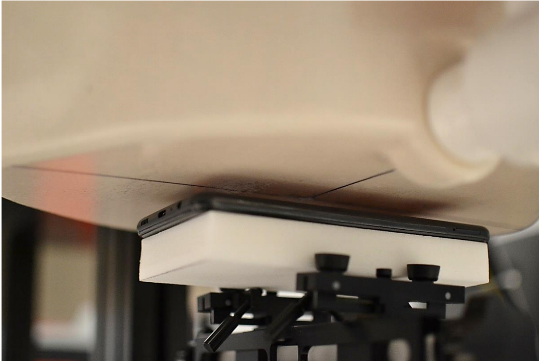
SAR Test Setup Photo 7 – Hotspot, Back Side at 10 mm
