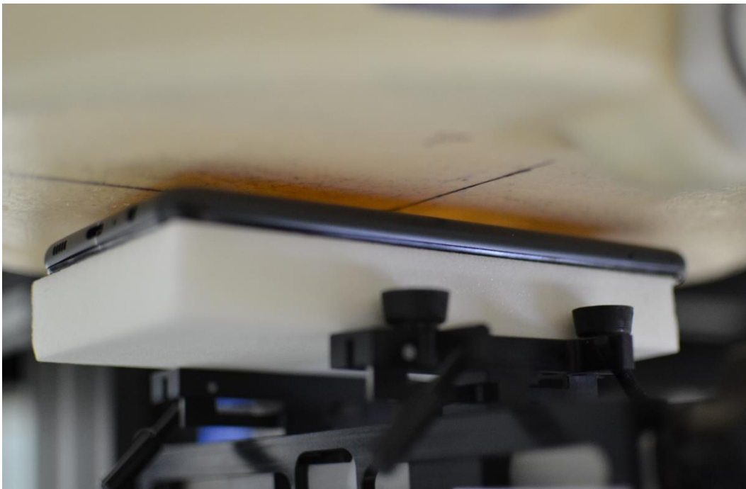
SAR Test Setup Photo 8 – Phablet, Back Side at 8 mm
