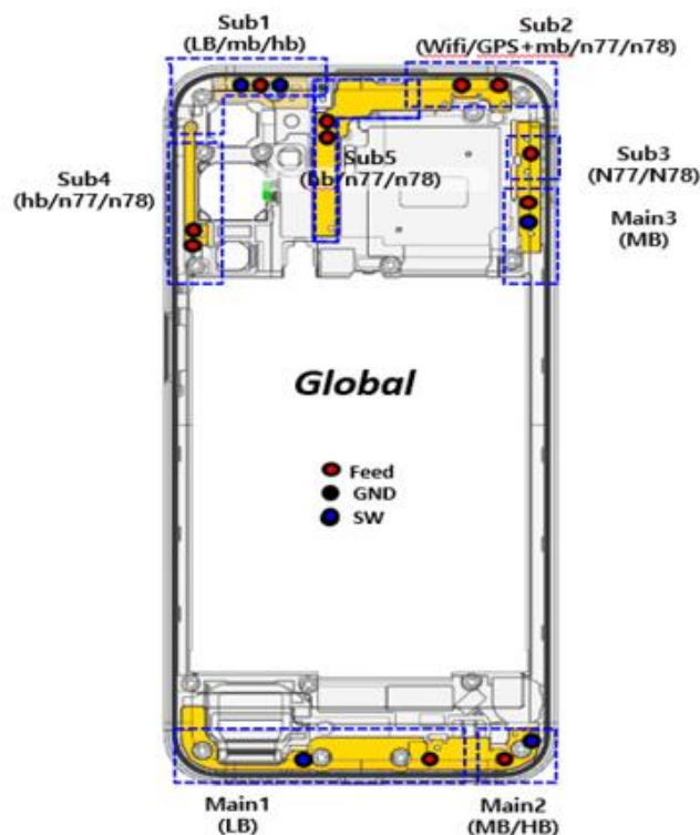
Photograph 16. Antenna position of EUT
