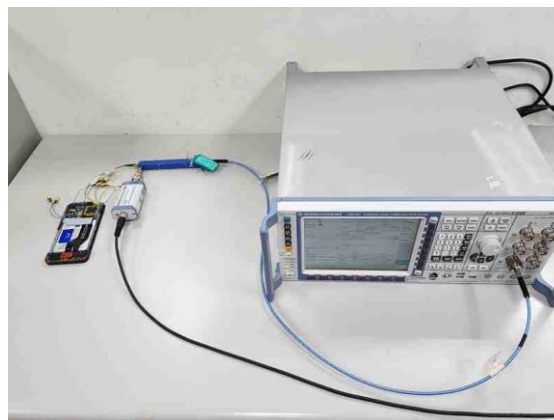
Photograph 2. Test Case 1/2/3/8/9/10, Time-varying TX power
