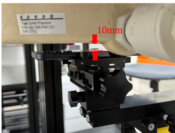
Photograph 12. Body, Back Side, 10mm
