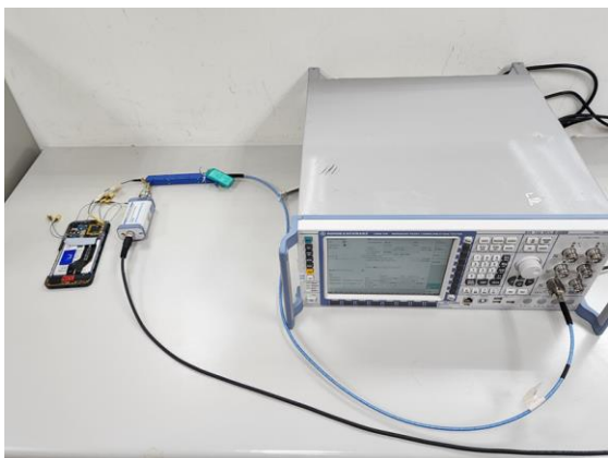
Photograph 1. Test Case 0, Range of TA SAR parameters
