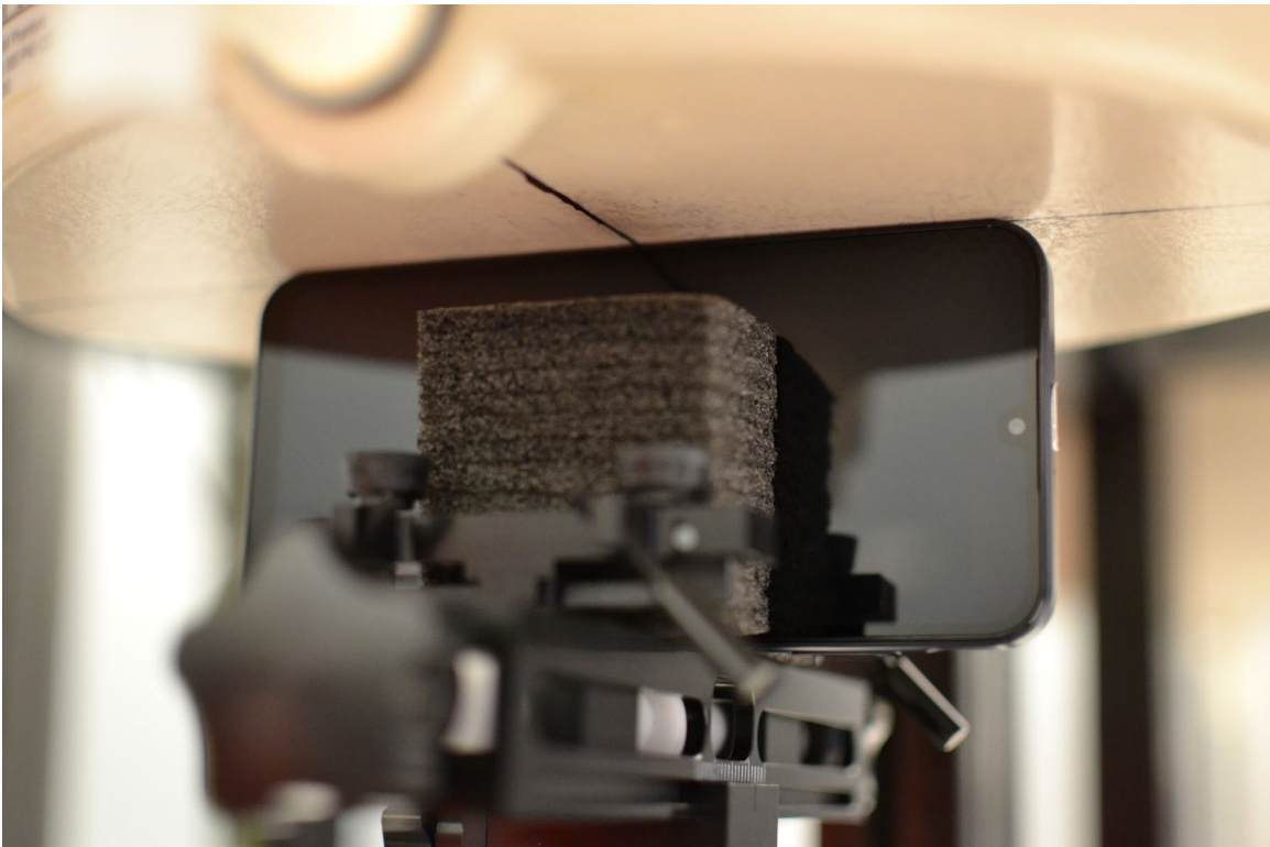
SAR Test Setup Photo 14 – Phablet, Left Edge at 0mm
