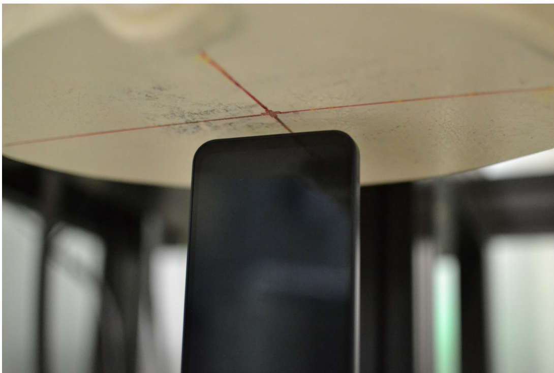
SAR Test Setup Photo 9 – Hotspot, Bottom Edge at 10mm
