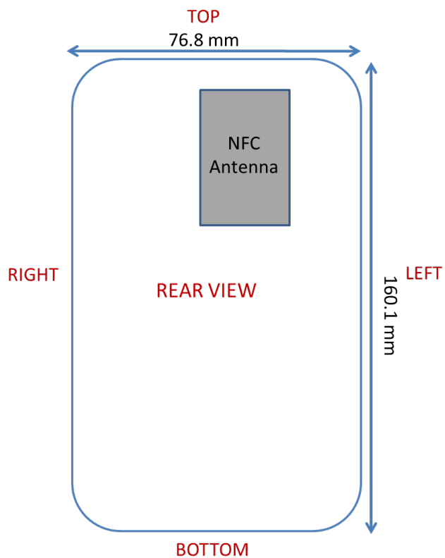
Figure J-2 NFC Antenna Locations
