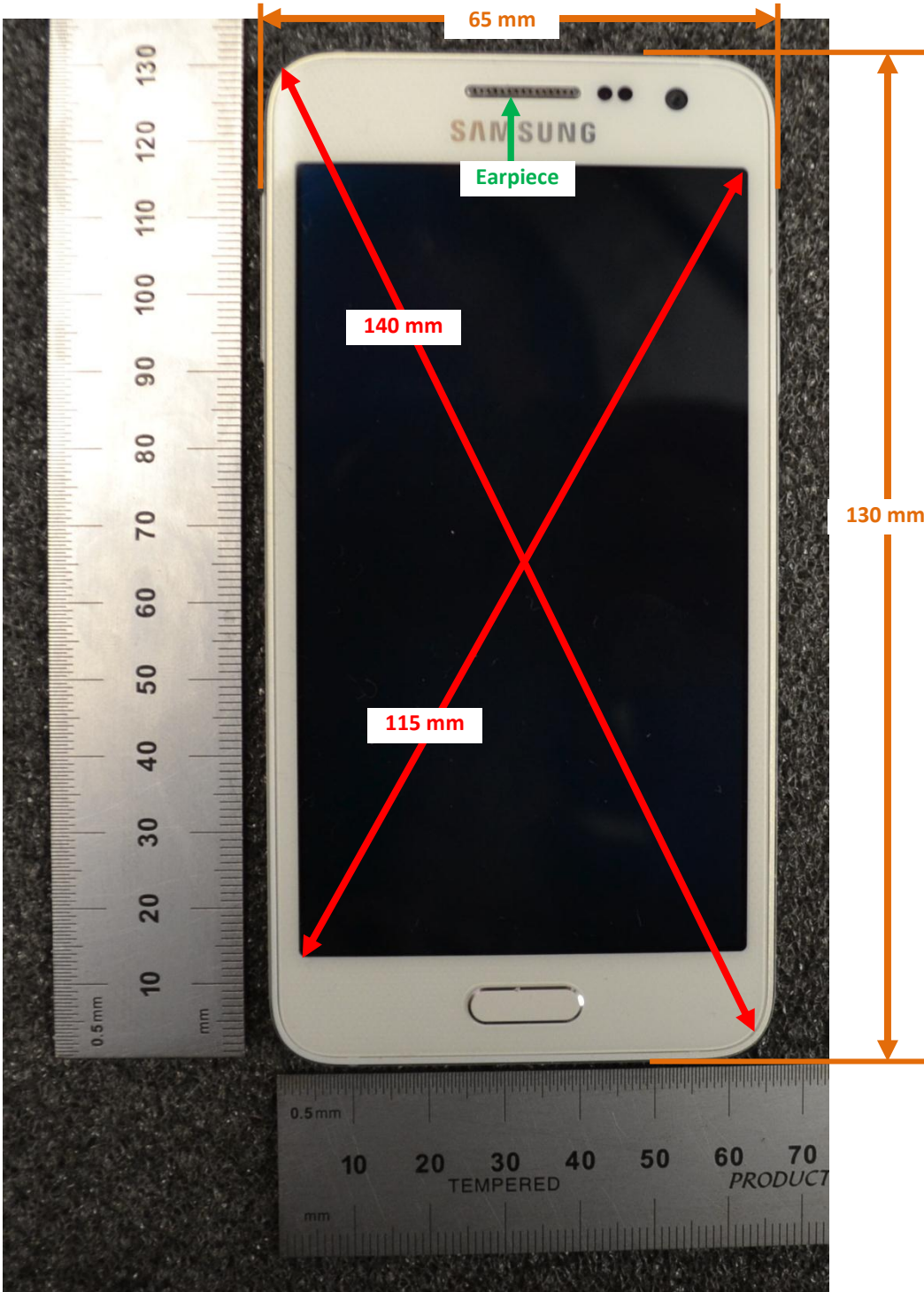
Overall Dimensions
