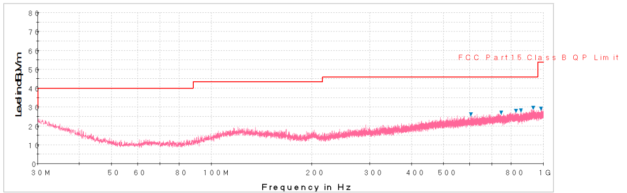
Plot 7-42. Radiated Spurious Plot below 1GHz (Pol. V)
