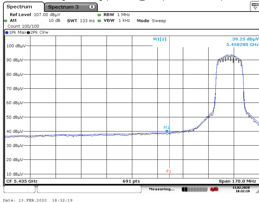
Peak Reading (802.11 a_6 Mbps, Ch.100, Y-H)
