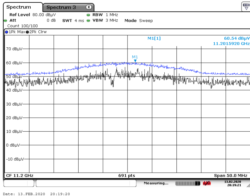
Peak Reading (802.11a, Ch.120 2nd Harmonic, Y-H)
