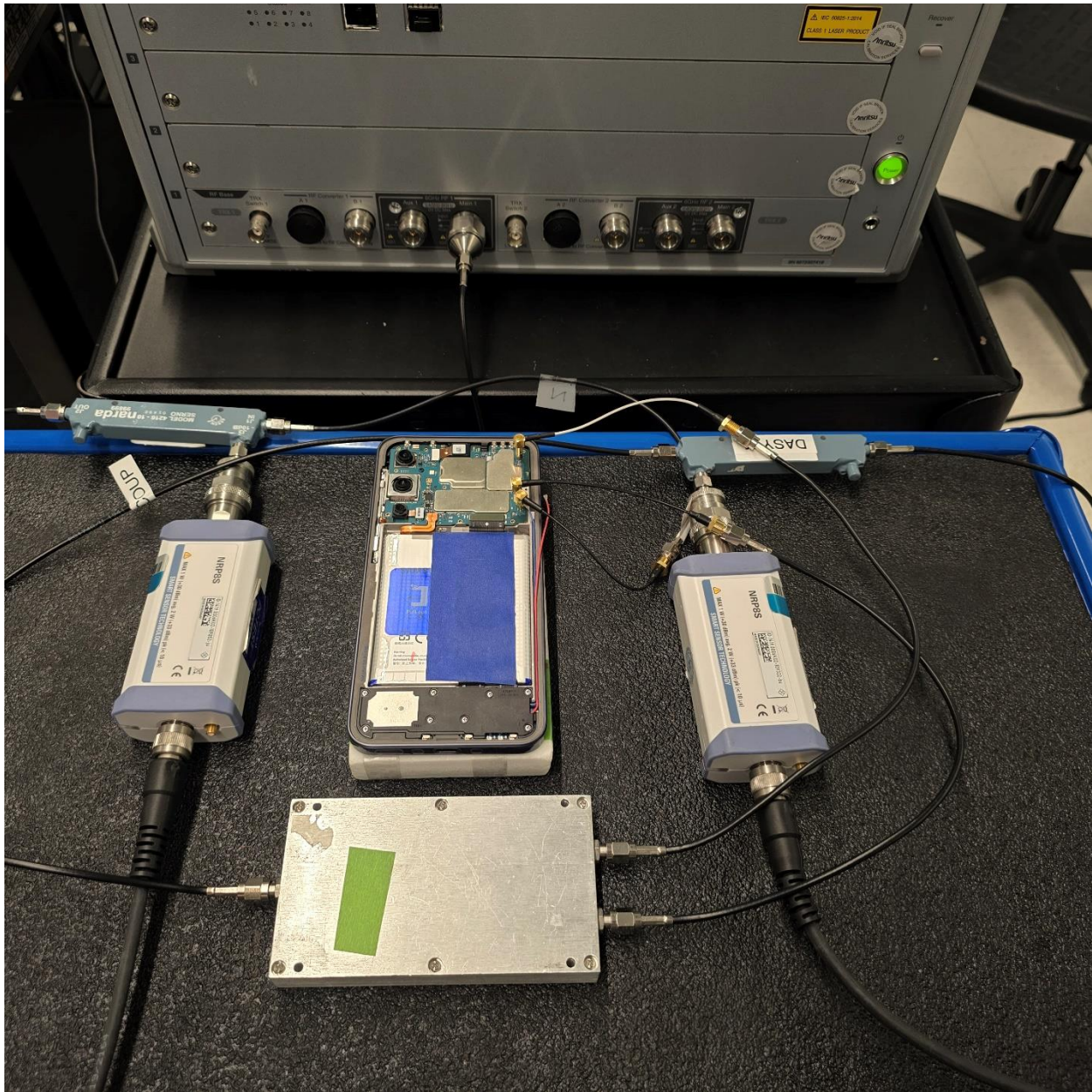
Test Setup Photo 10 – Conducted Test Setup (Figure 6-1d)
