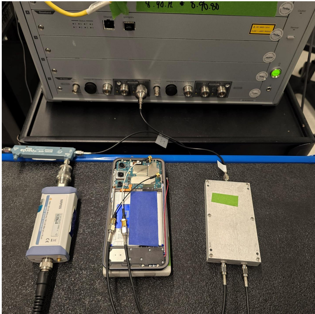
Test Setup Photo 8 – Conducted Test Setup (Figure 6-1b)
