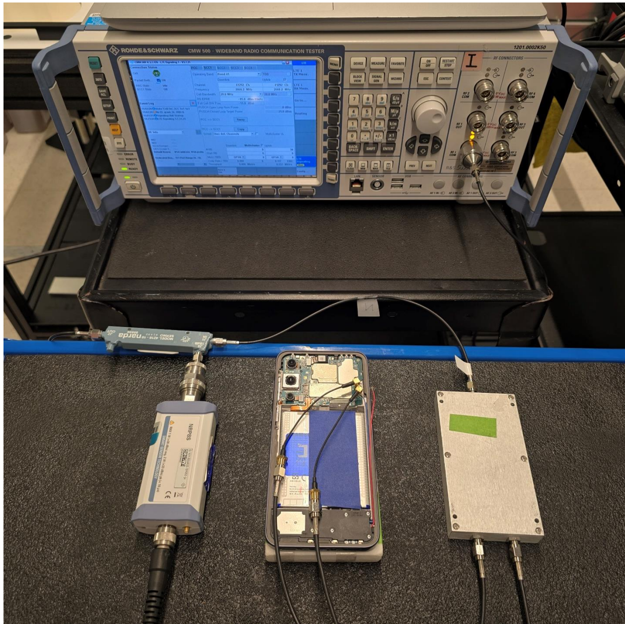
Test Setup Photo 6 – Conducted Test Setup (Figure 6-1b)
