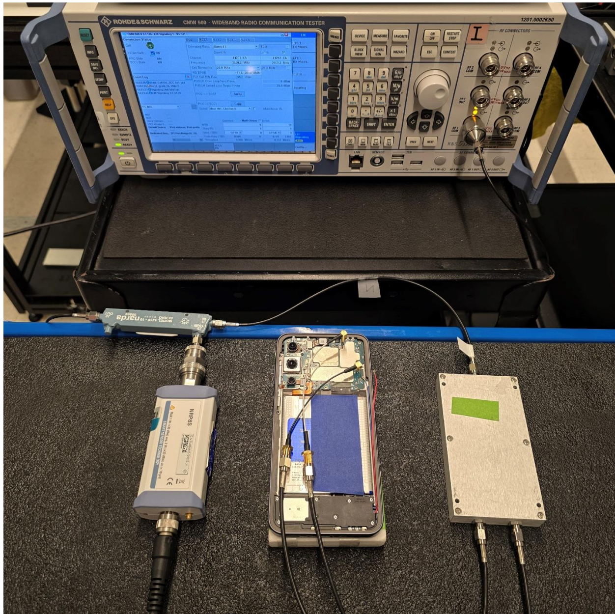
Test Setup Photo 7 – Conducted Test Setup (Figure 6-1b)
