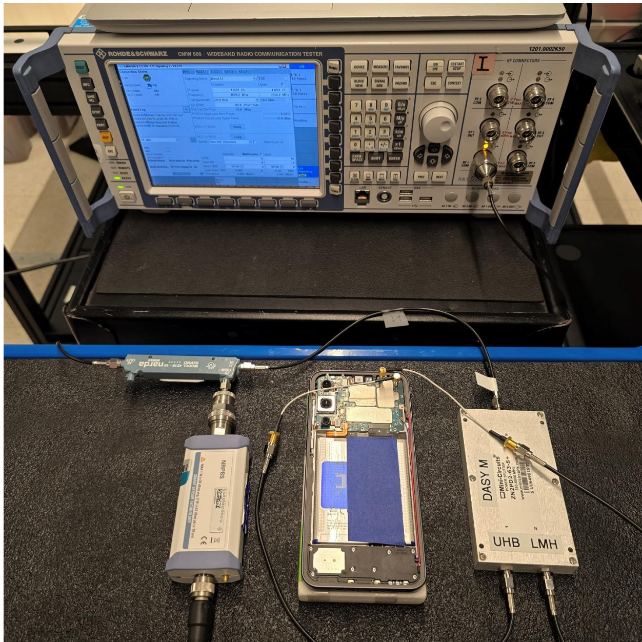
Test Setup Photo 4 - Conducted Test Setup (Figure 6-1b)
