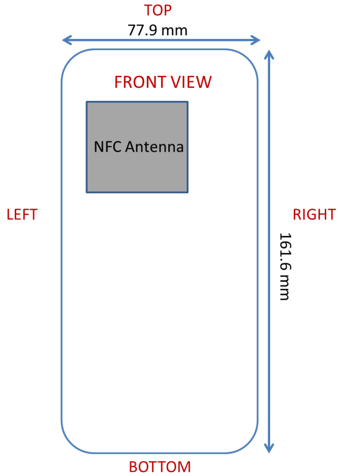
Figure K-2 NFC Antenna Locations
