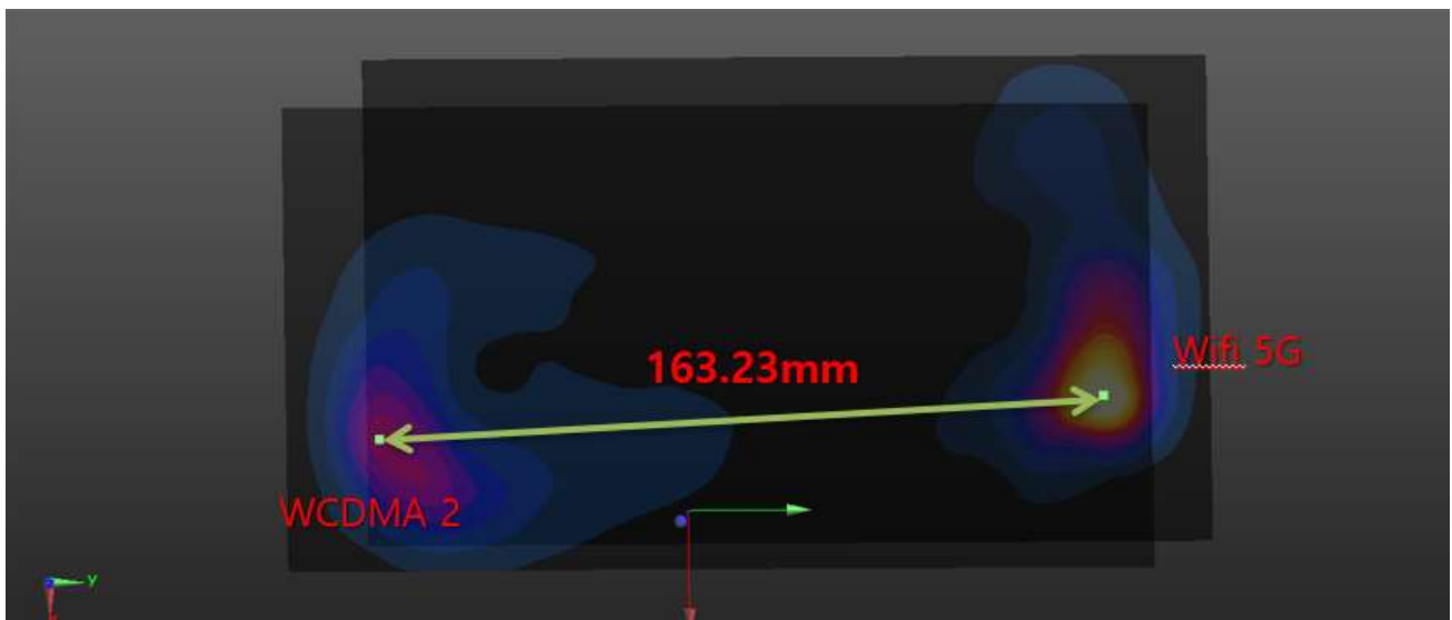
Plot #4 WCDMA B2 + WLAN 5GHz (Hotspot Mode)
