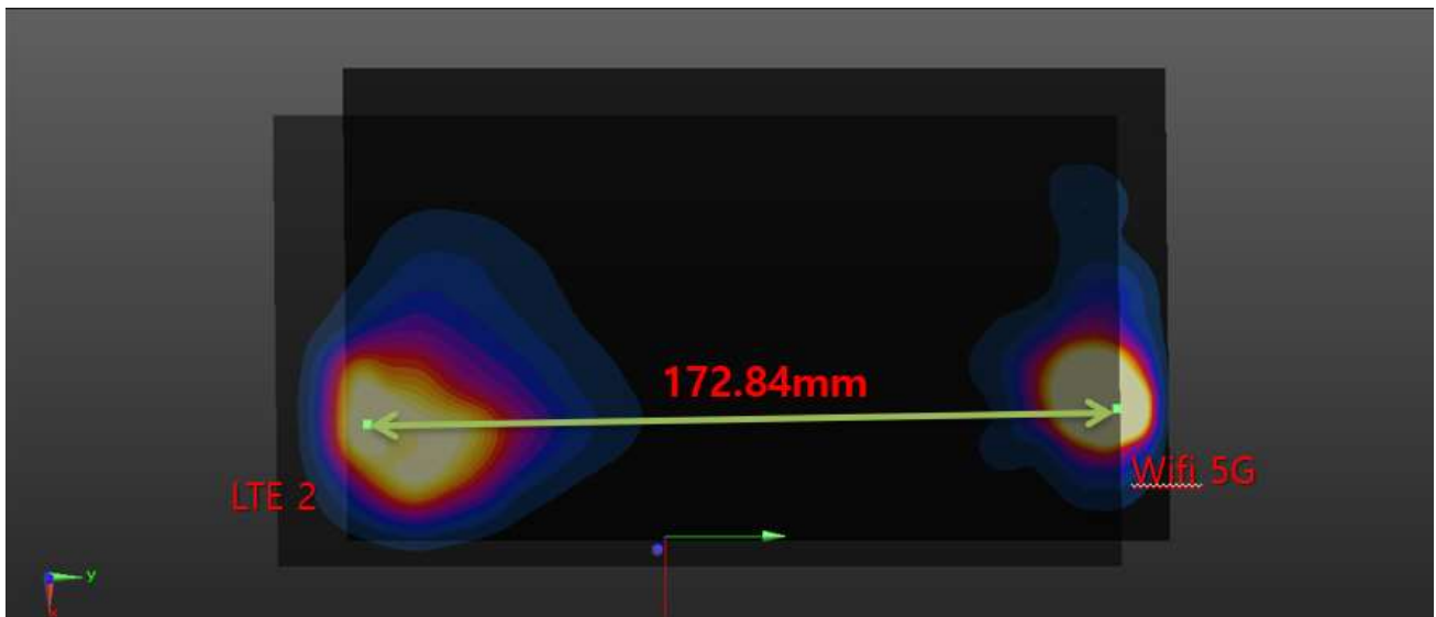
Plot #8 LTE Band 2 + WLAN 5GHz (Phablet Mode)
