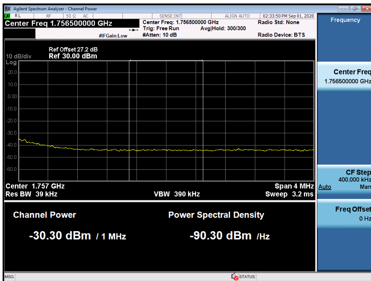
BAND 4. Upper Extended Band Edge Plot (20M BW Ch.20300 QPSK_RB100) -3
