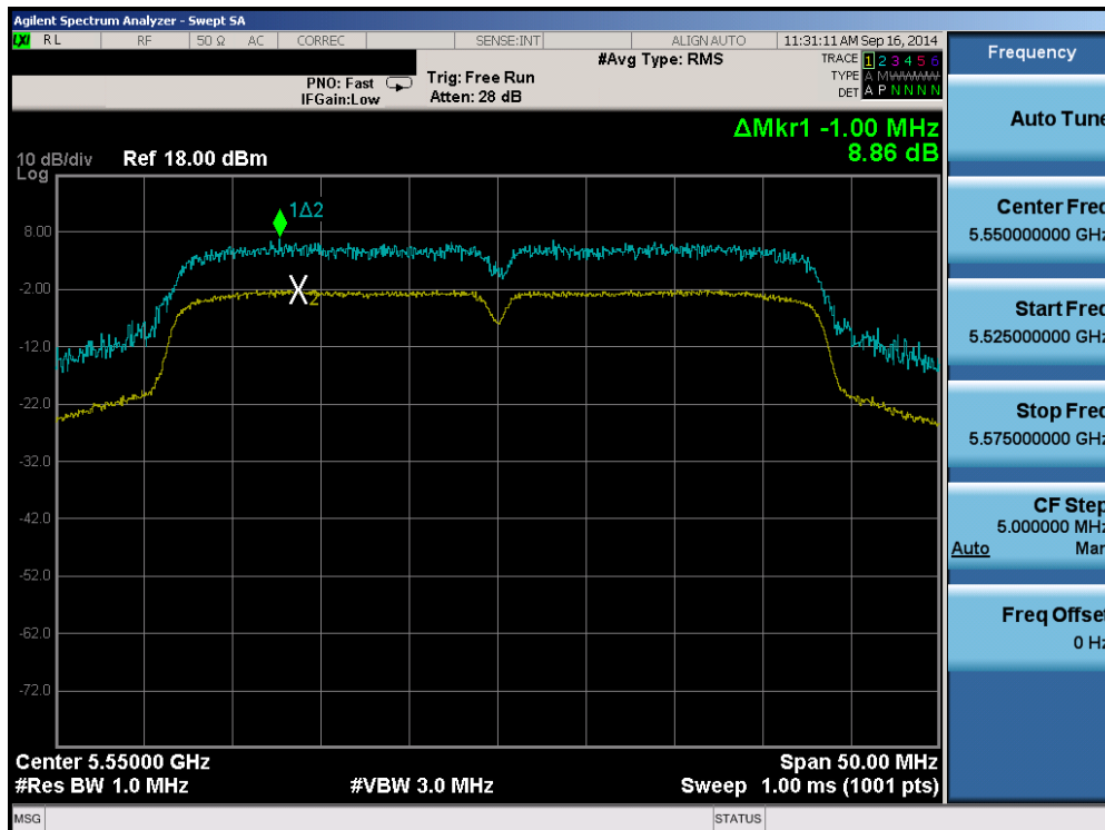
Plot 6-58. Peak Excursion Ratio Plot (40MHz BW 802.11n (UNII Band 2C) – Ch. 110)
