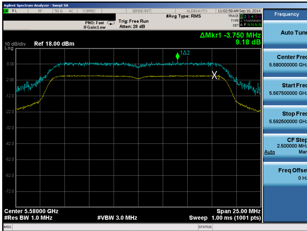
Plot 6-57. Peak Excursion Ratio Plot (20MHz BW 802.11n (UNII Band 2C) – Ch. 116)
