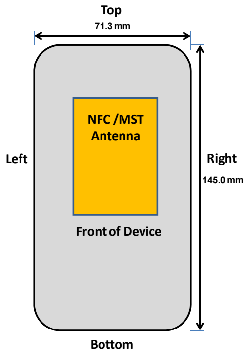
Figure F-2 NFC/MST Antenna Locations
