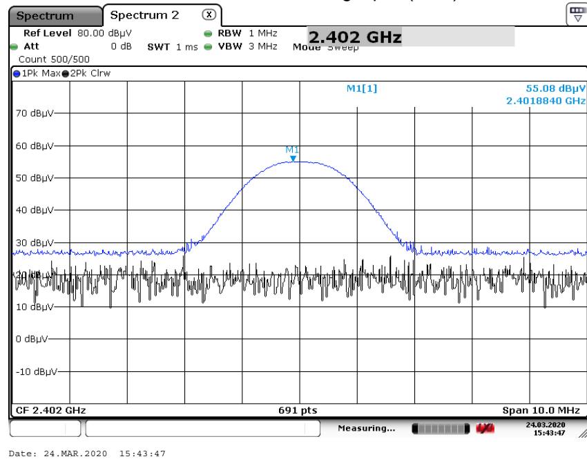
Fundamental Field Strength plot (Ch.0)
