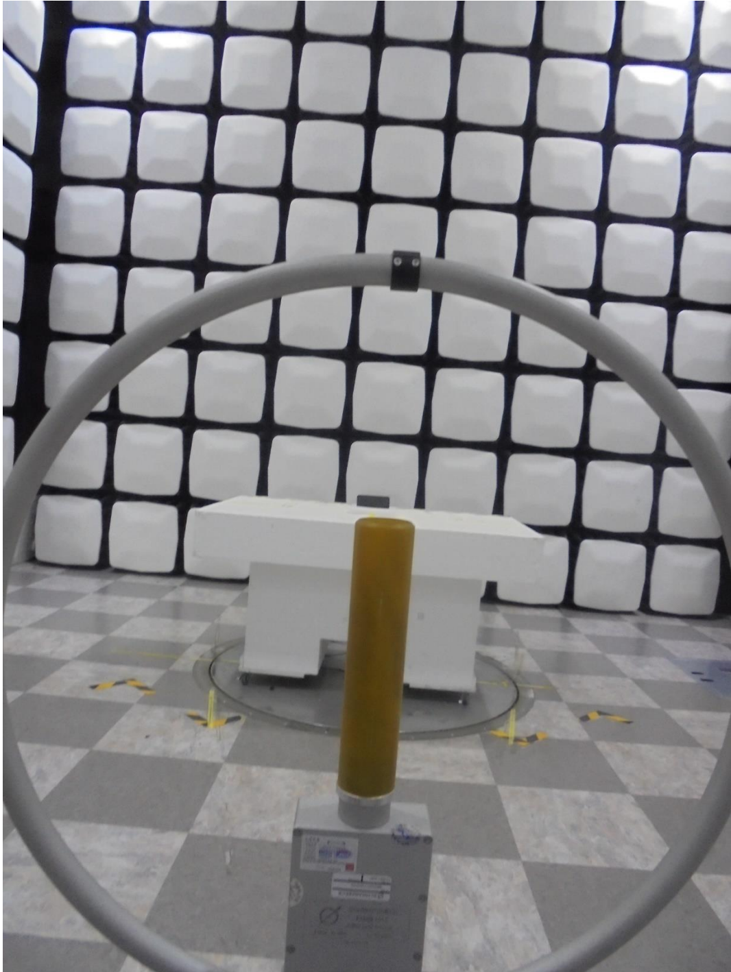
NFC Radiated Test Setup Photo for 9 kHz ~ 30 MHz:
