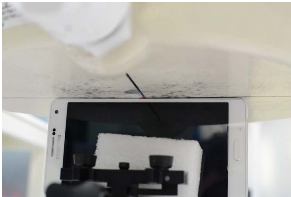
SAR Test Setup Photo 15 – Right Edge at 0.0 cm
