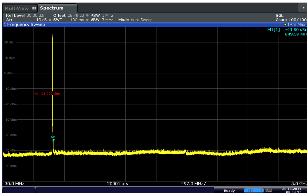
Plot 6-45. Conducted Spurious Plot (Band 5–10.0MHz–QPSK–RB Size 1–RB Offset 0– Ch.20525)
