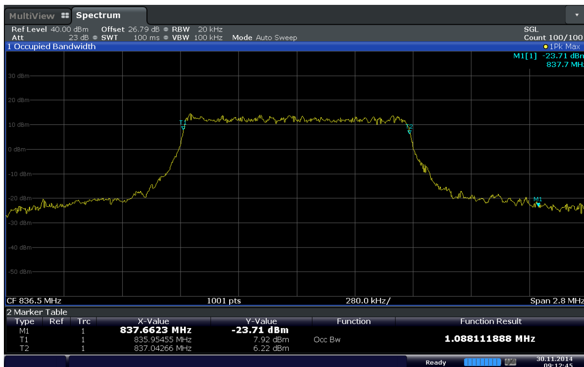
Plot 6-5. Occupied Bandwidth Plot (Band 5 – 1.4MHz QPSK - RB Size 6)
