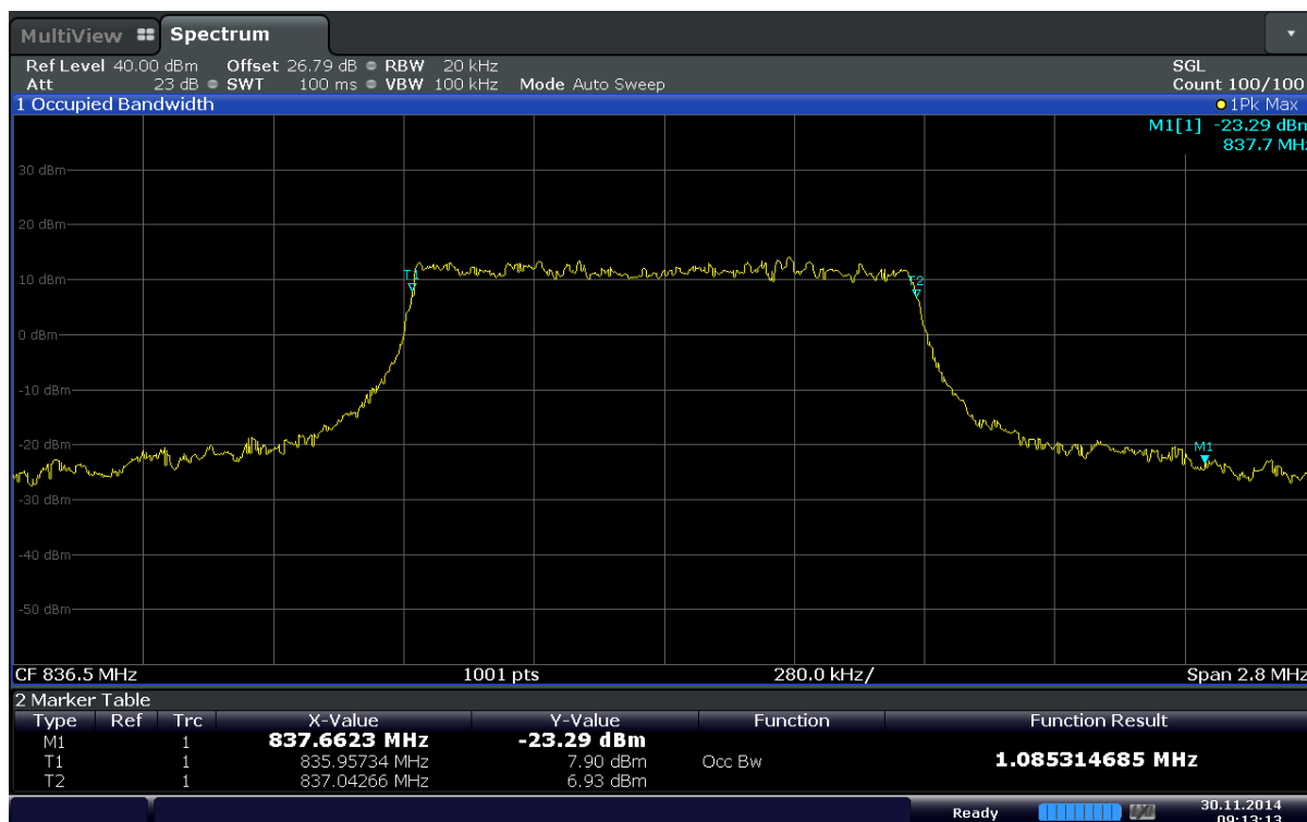
Plot 6-6. Occupied Bandwidth Plot (Band 5 – 1.4MHz 16QAM - RB Size 6)
