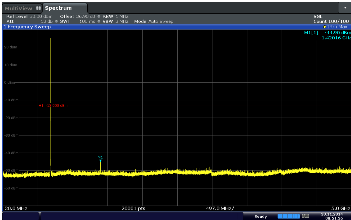
Plot 6-15. Conducted Spurious Plot (Band 17–5MHz–QPSK–RB Size 1–RB Offset 12–Ch.23790)
