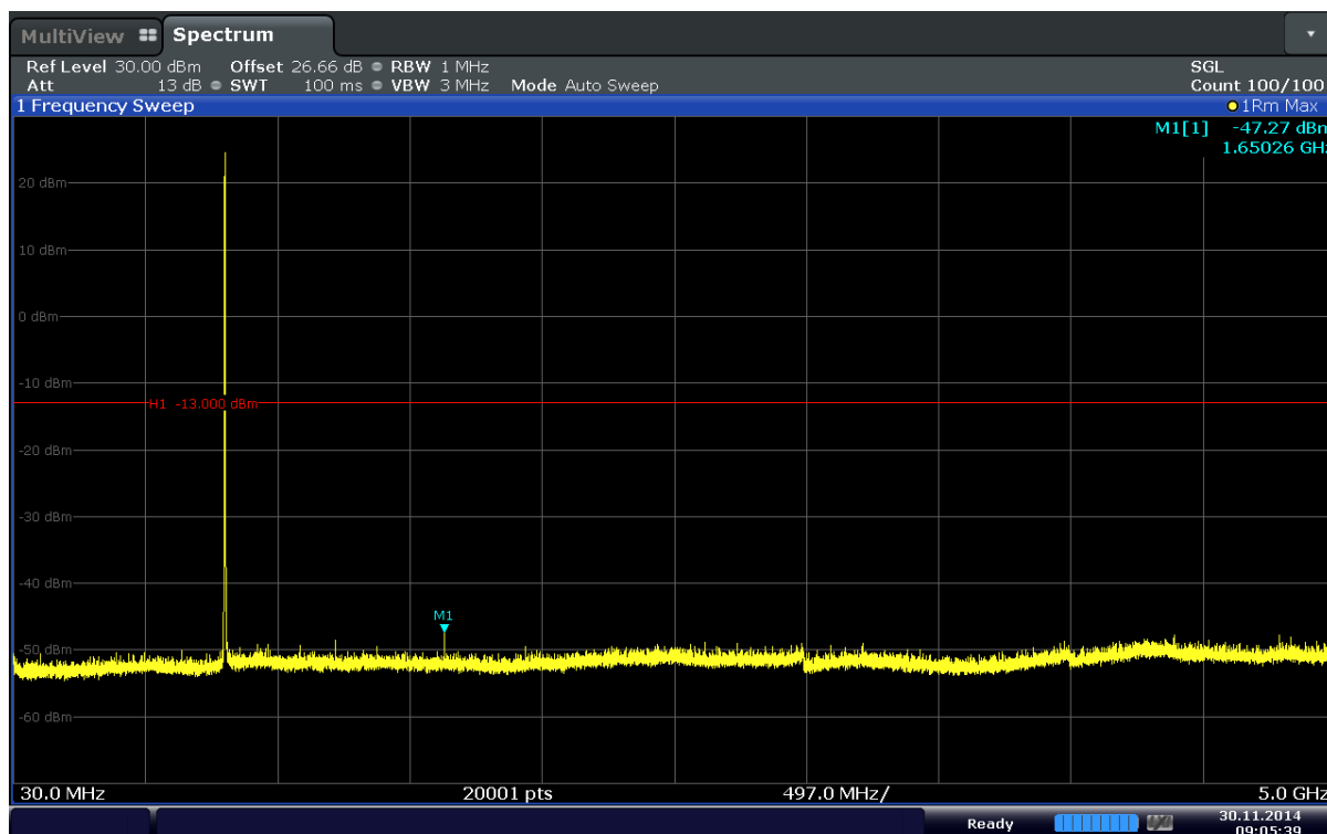
Plot 6-27. Conducted Spurious Plot (Band 5–1.4MHz–QPSK–RB Size 3–RB Offset 3–Ch.20525)
