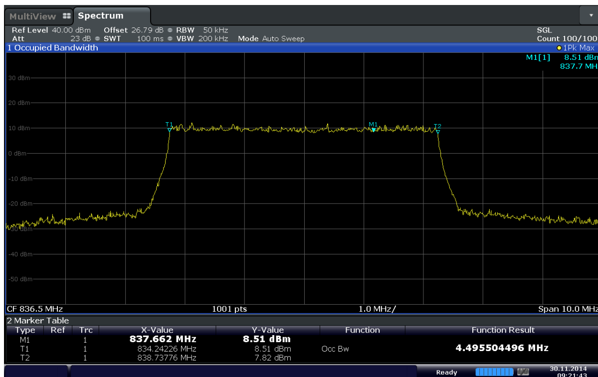
Plot 6-10. Occupied Bandwidth Plot (Band 5 - 5.0MHz 16QAM - RB Size 25)
