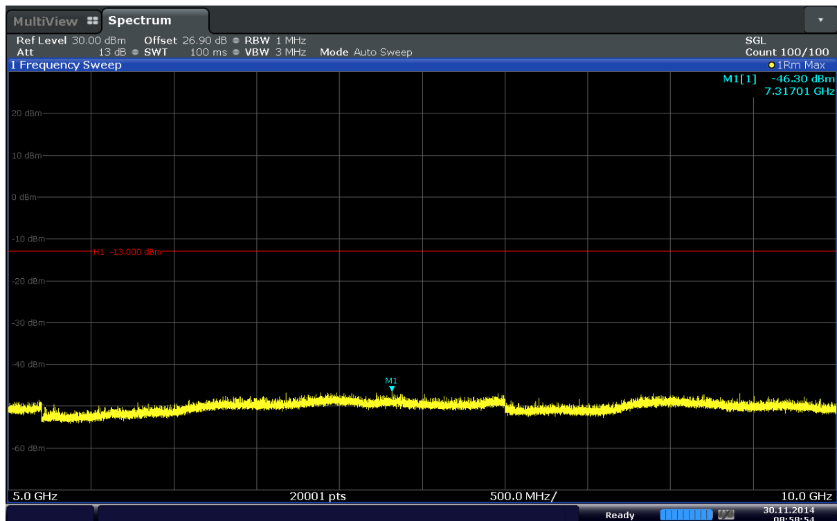
6-22. Conducted Spurious Plot (Band 17–10MHz–QPSK–RB Size 1–RB Offset 49–Ch.23790)
