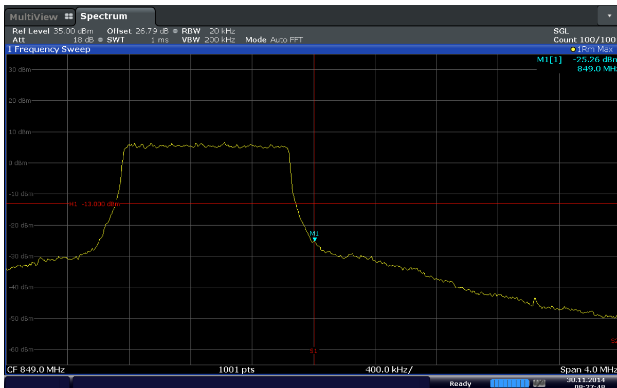
Plot 6-56. Upper Band Edge Plot (Band5 – 1.4MHz – QPSK – RB Size 6)
