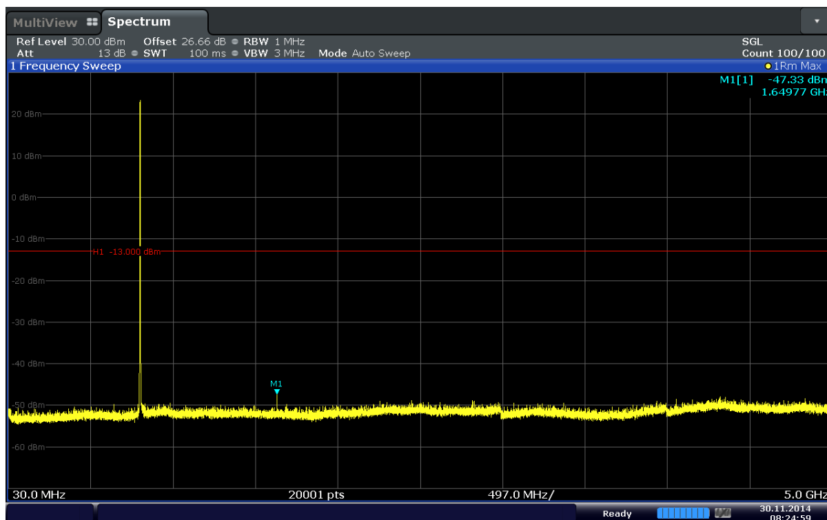
Plot 6-25. Conducted Spurious Plot (Band 5–1.4MHz–QPSK–RB Size 3–RB Offset 2–Ch.20407)
