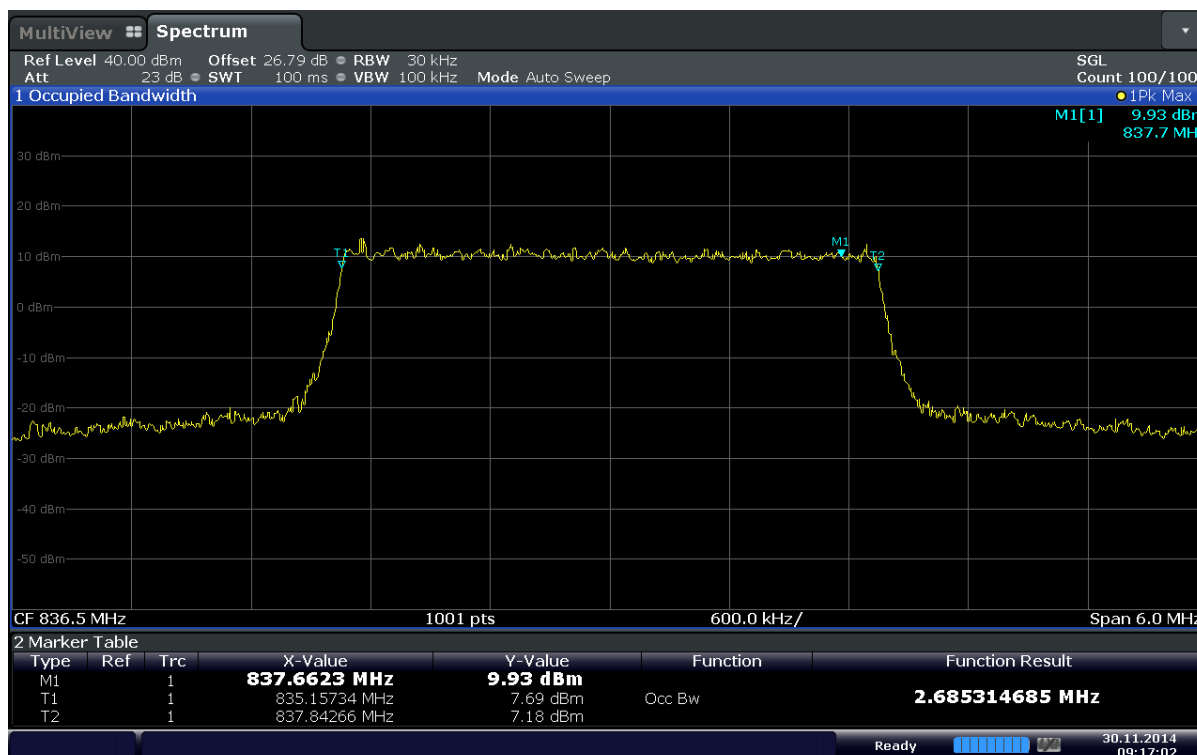
Plot 6-7. Occupied Bandwidth Plot (Band 5 - 3.0MHz QPSK - RB Size 15)
