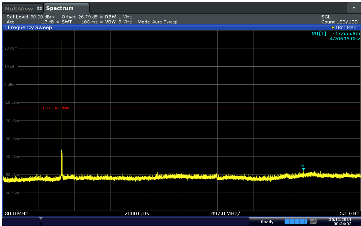
Plot 6-35. Conducted Spurious Plot (Band 5–3.0MHz–QPSK–RB Size 1–RB Offset 7– Ch.20635)
