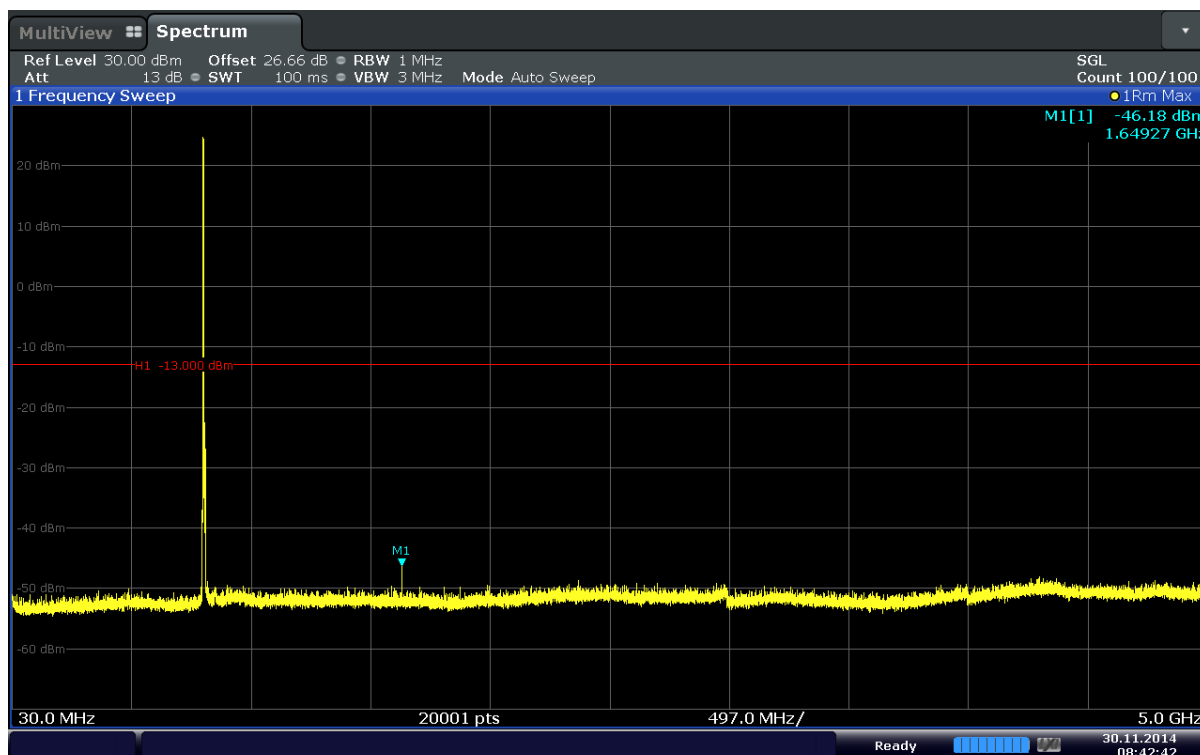
Plot 6-43. Conducted Spurious Plot (Band 5–10.0MHz–QPSK–RB Size 1–RB Offset 0– Ch.20450)
