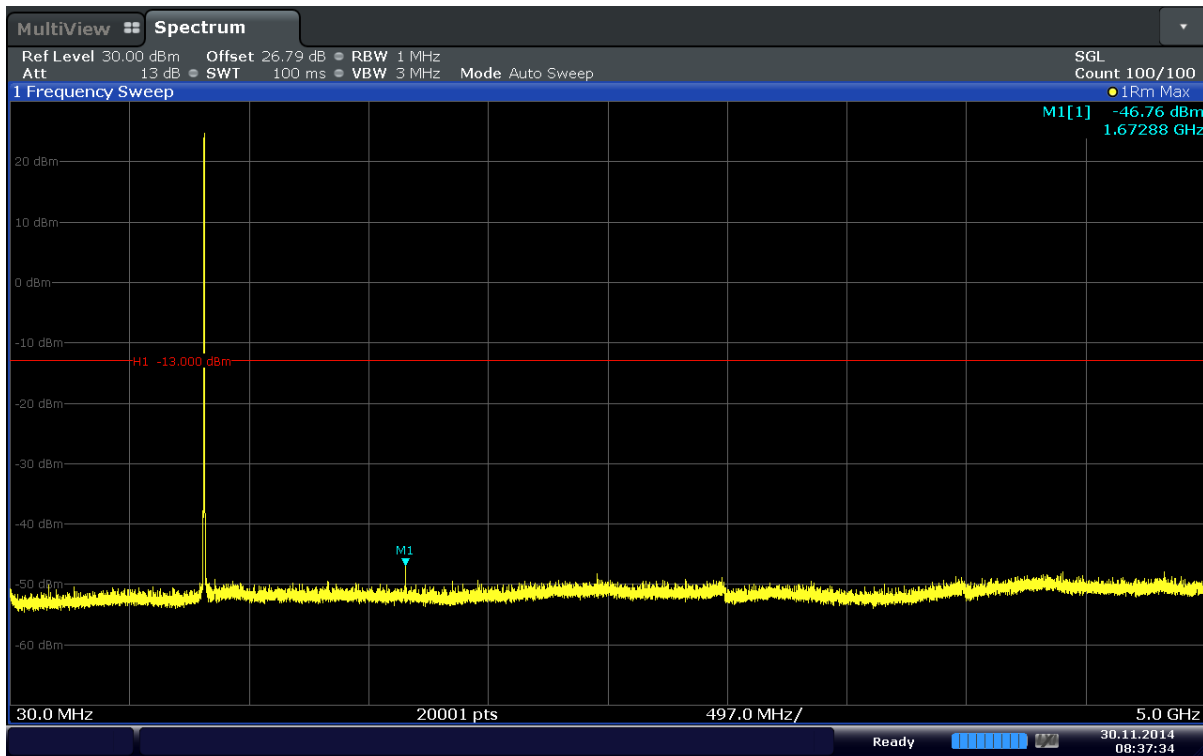
Plot 6-39. Conducted Spurious Plot (Band 5–5.0MHz–QPSK–RB Size 1–RB Offset 12– Ch.20525)
