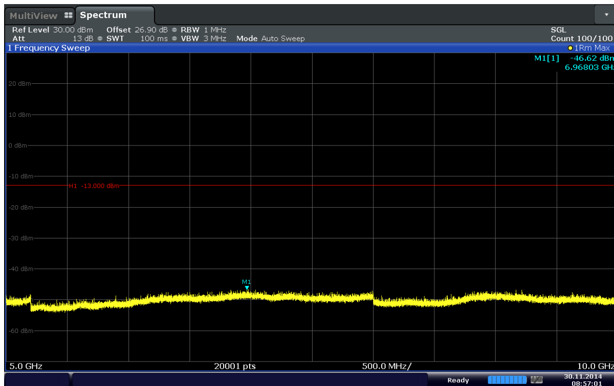
6-20. Conducted Spurious Plot (Band 17–10MHz–QPSK–RB Size 1–RB Offset 0–Ch.23780)
