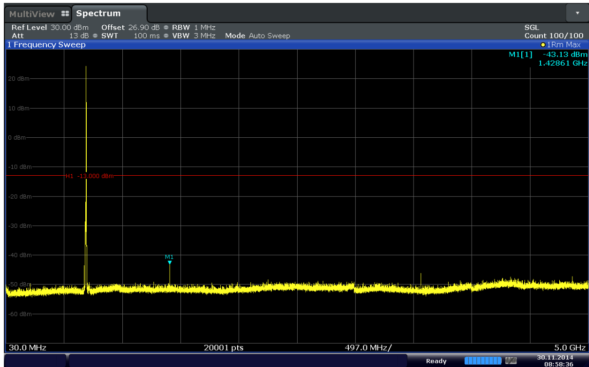
Plot 6-21. Conducted Spurious Plot (Band 17–10MHz–QPSK–RB Size 1–RB Offset 49–Ch.23790)
