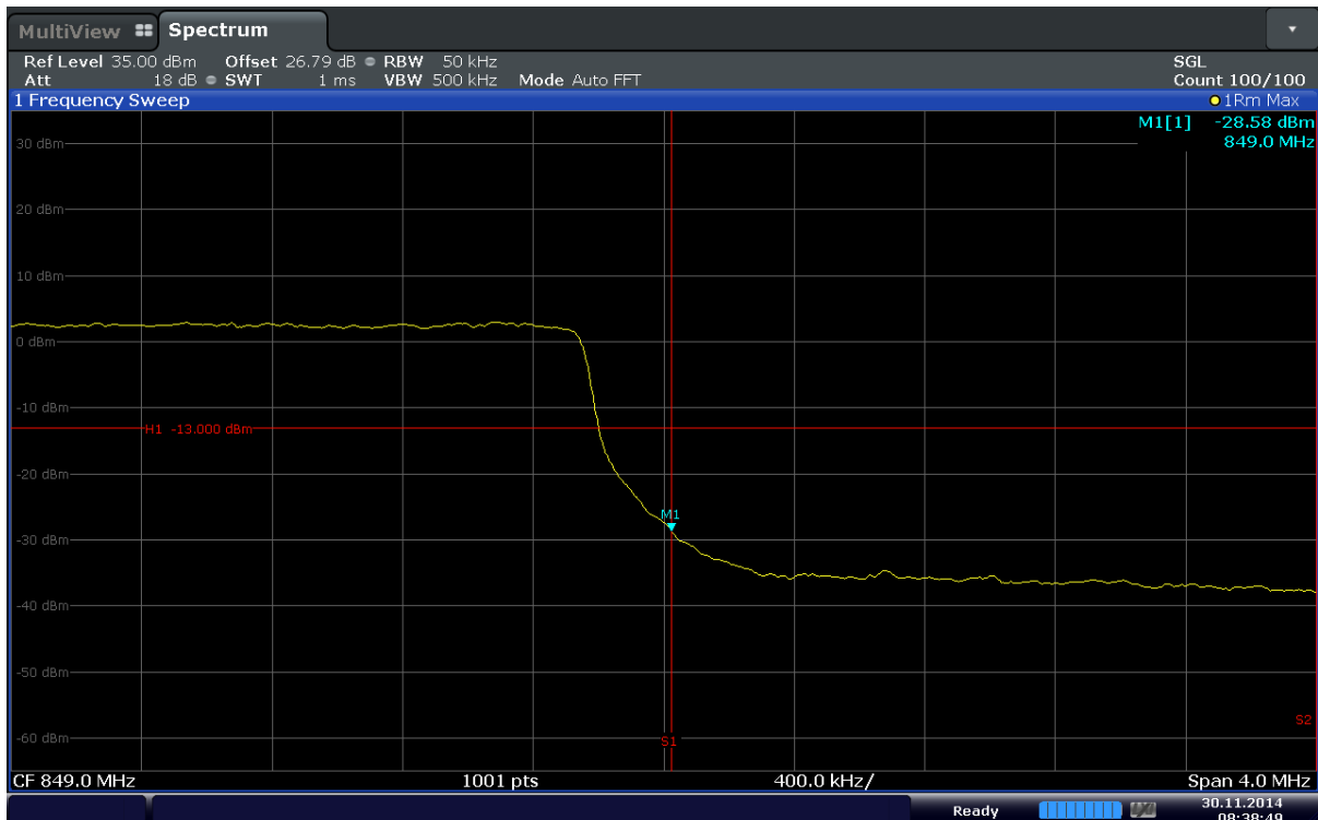
Plot 6-60. Upper Band Edge Plot (Band 5 – 5.0MHz – QPSK – RB Size 25)
