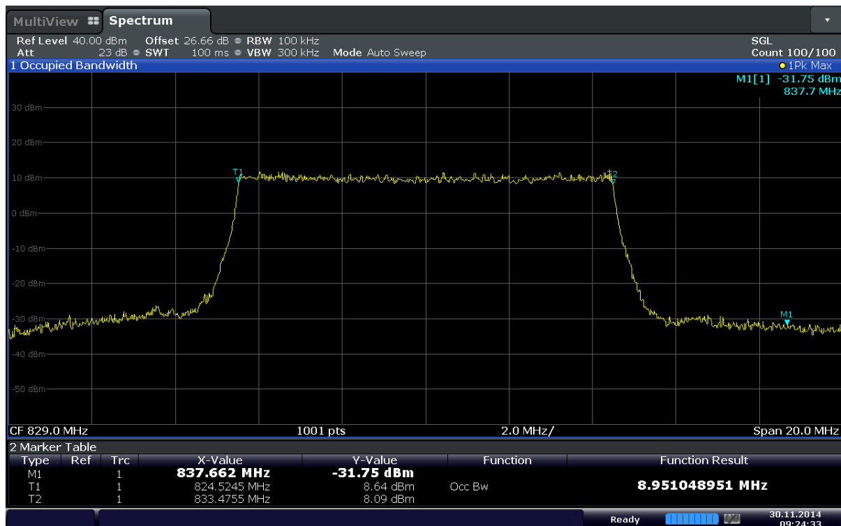
Plot 6-12. Occupied Bandwidth Plot (Band 5 - 10.0MHz 16QAM - RB Size 50)
