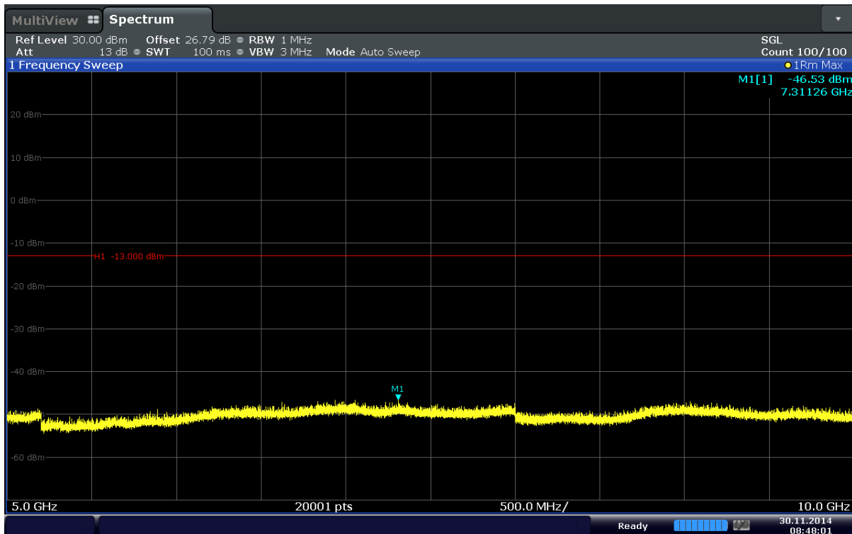
Plot 6-48. Conducted Spurious Plot (Band 5–10.0MHz–QPSK–RB Size 1–RB Offset 0– Ch.20600)
