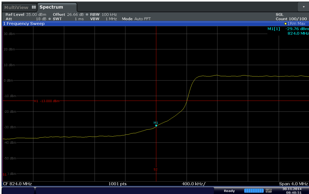
Plot 6-61. Lower Band Edge Plot (Band 5 – 10.0MHz – QPSK – RB Size 50)
