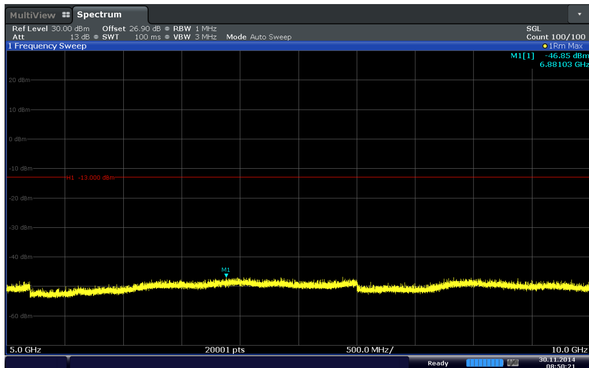
6-14. Conducted Spurious Plot (Band 17–5MHz–QPSK–RB Size 1–RB Offset 0–Ch.23755)
