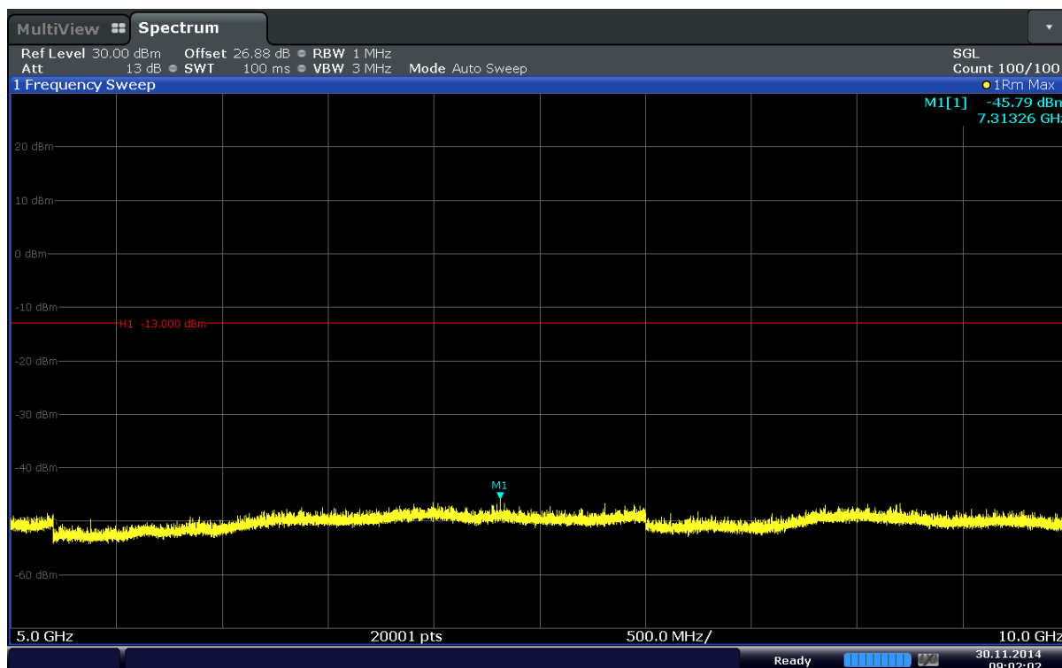
6-24. Conducted Spurious Plot (Band 17–10MHz–QPSK–RB Size 1–RB Offset 24–Ch.23800)
