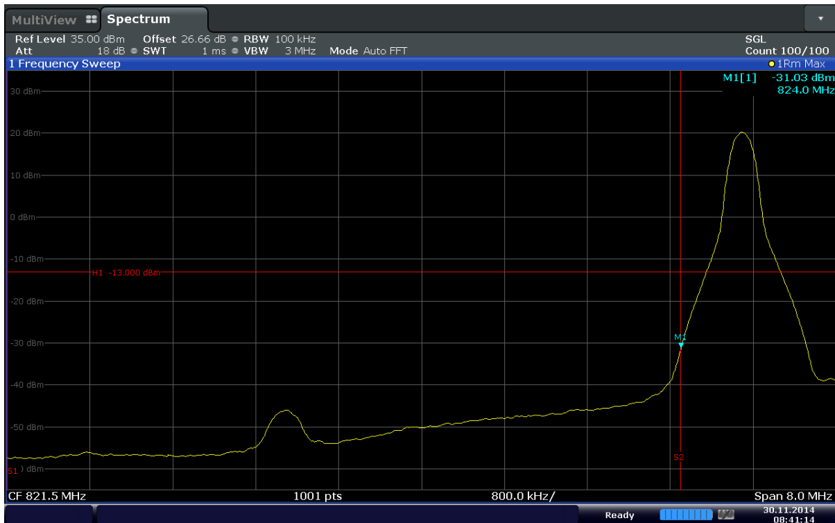
Plot 6-62. Lower Band Edge Plot (Band 5 – 10.0MHz – QPSK – RB Size 1 – RB Offset 0)
