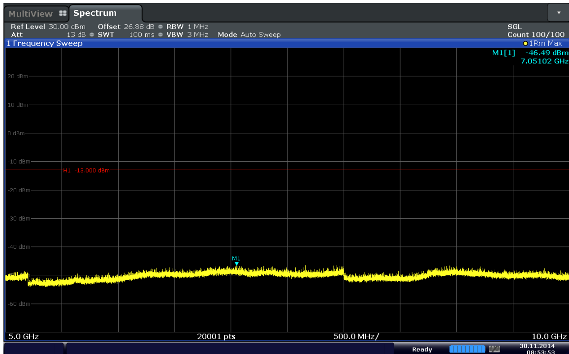
6-18. Conducted Spurious Plot (Band 17–5MHz–QPSK–RB Size 1–RB Offset 24–Ch.23825)
