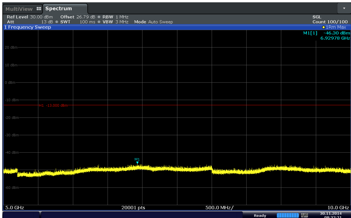
Plot 6-34. Conducted Spurious Plot (Band 5–3.0MHz–QPSK–RB Size 1–RB Offset 14– Ch.20525)
