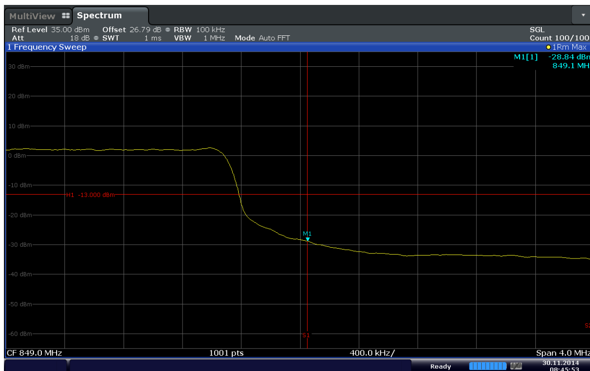
Plot 6-63. Upper Band Edge Plot (Band 5 – 10.0MHz – QPSK – RB Size 50)
