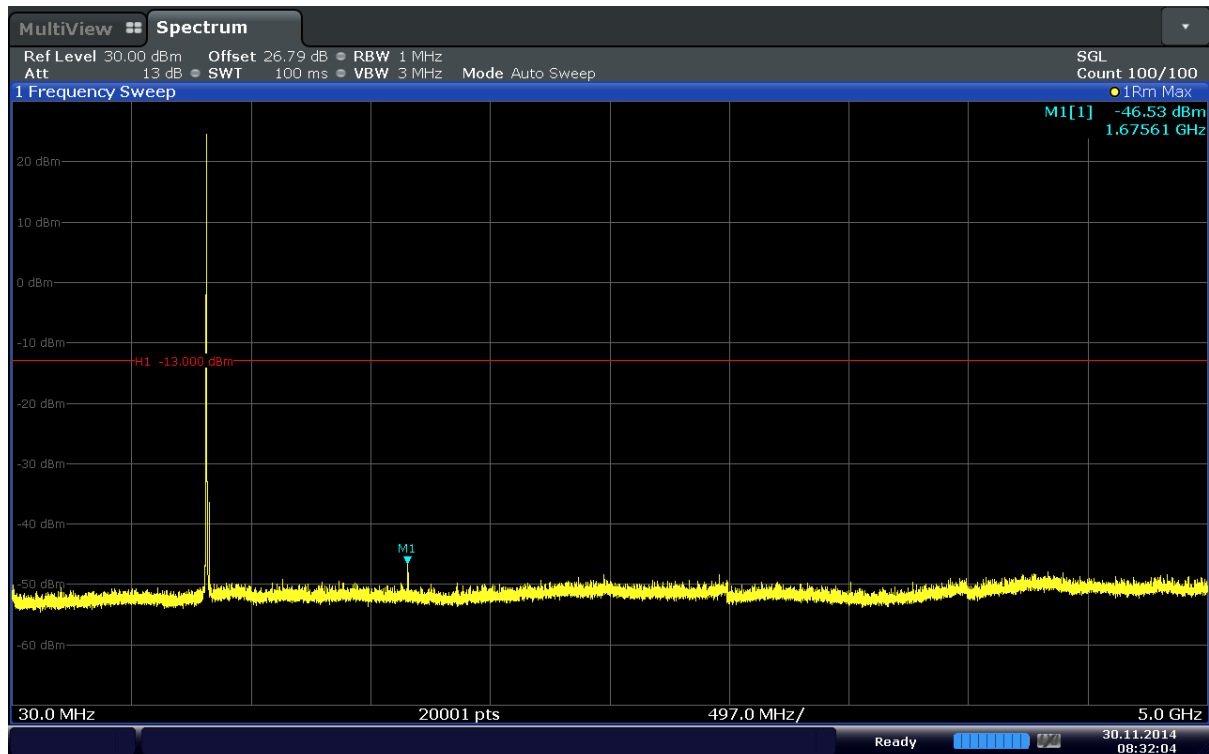
Plot 6-33. Conducted Spurious Plot (Band 5–3.0MHz–QPSK–RB Size 1–RB Offset 14– Ch.20525)
