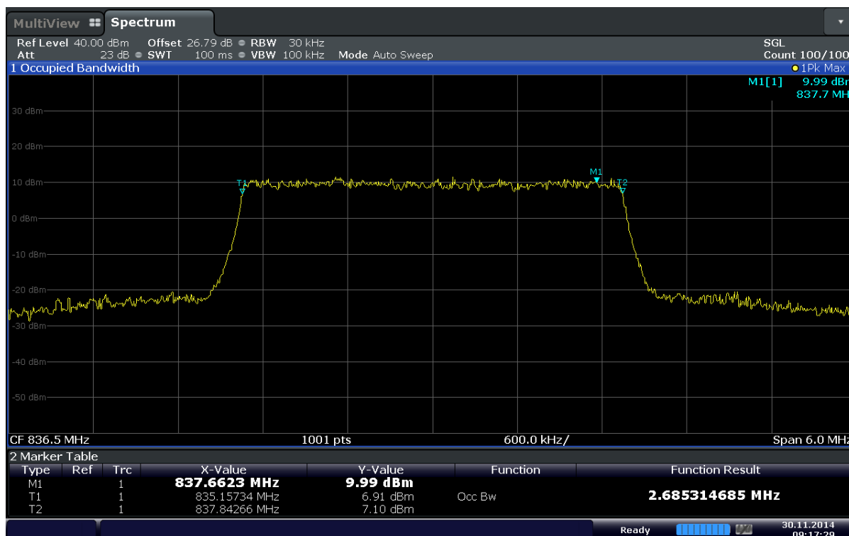
Plot 6-8. Occupied Bandwidth Plot (Band 5 - 3.0MHz 16QAM - RB Size 15)
