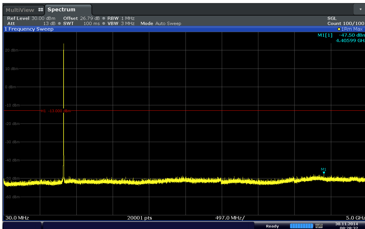
Plot 6-29. Conducted Spurious Plot (Band 5–1.4MHz–QPSK–RB Size 3–RB Offset 3– Ch.20643)
