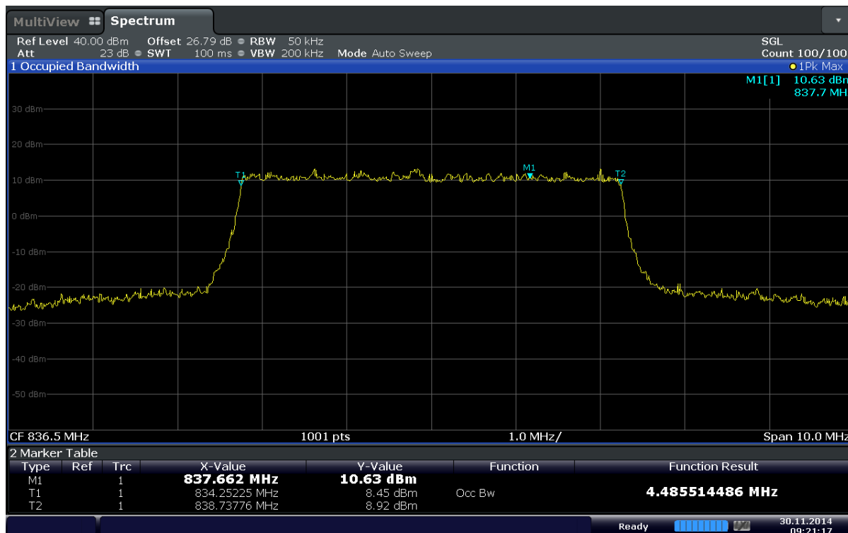
Plot 6-9. Occupied Bandwidth Plot (Band 5 - 5.0MHz QPSK - RB Size 25)
