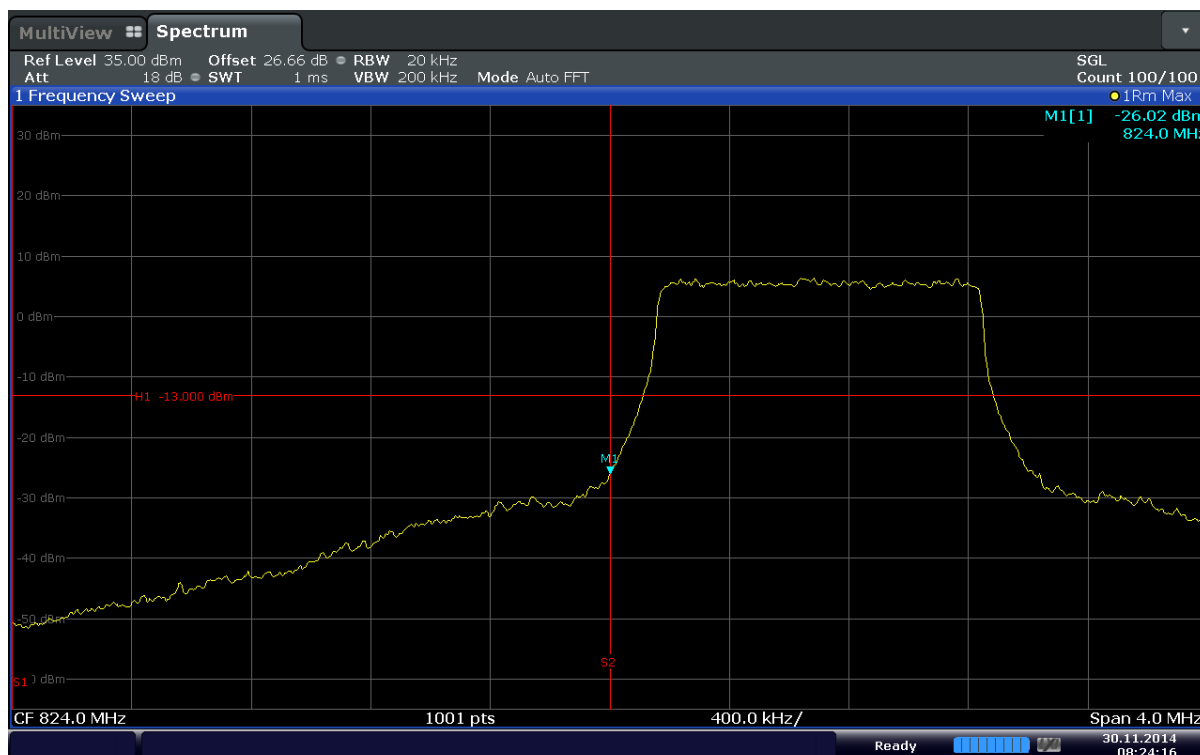
Plot 6-55. Lower Band Edge Plot (Band5 – 1.4MHz – QPSK – RB Size 6)
