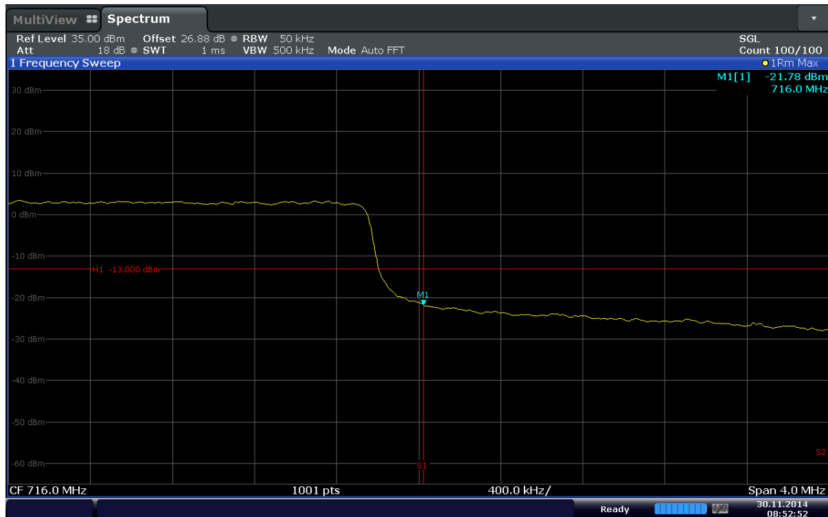
Plot 6-50. Upper Band Edge Plot (Band17 – 5MHz – QPSK – RB Size 25)
