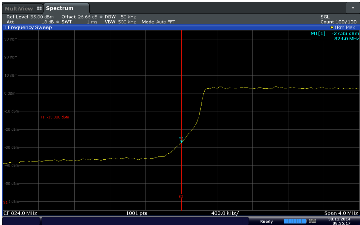
Plot 6-59. Lower Band Edge Plot (Band 5 – 5.0MHz – QPSK – RB Size 25)
