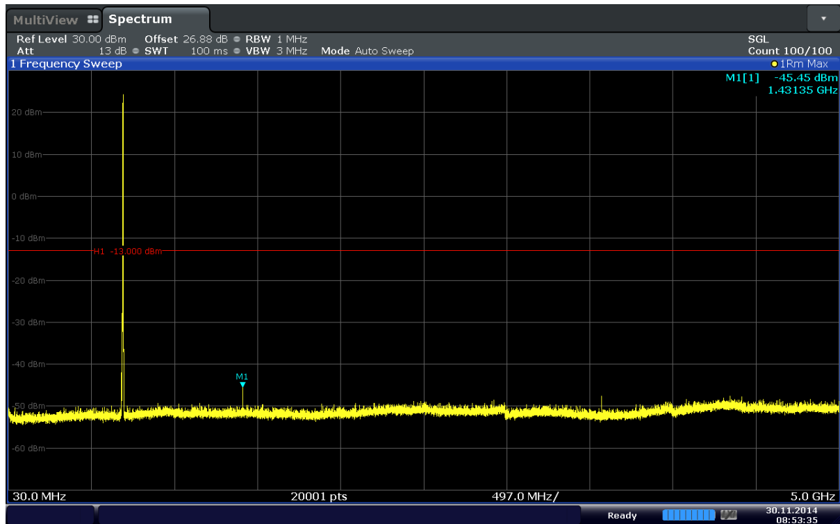
Plot 6-17. Conducted Spurious Plot (Band 17–5MHz–QPSK–RB Size 1–RB Offset 24–Ch.23825)
