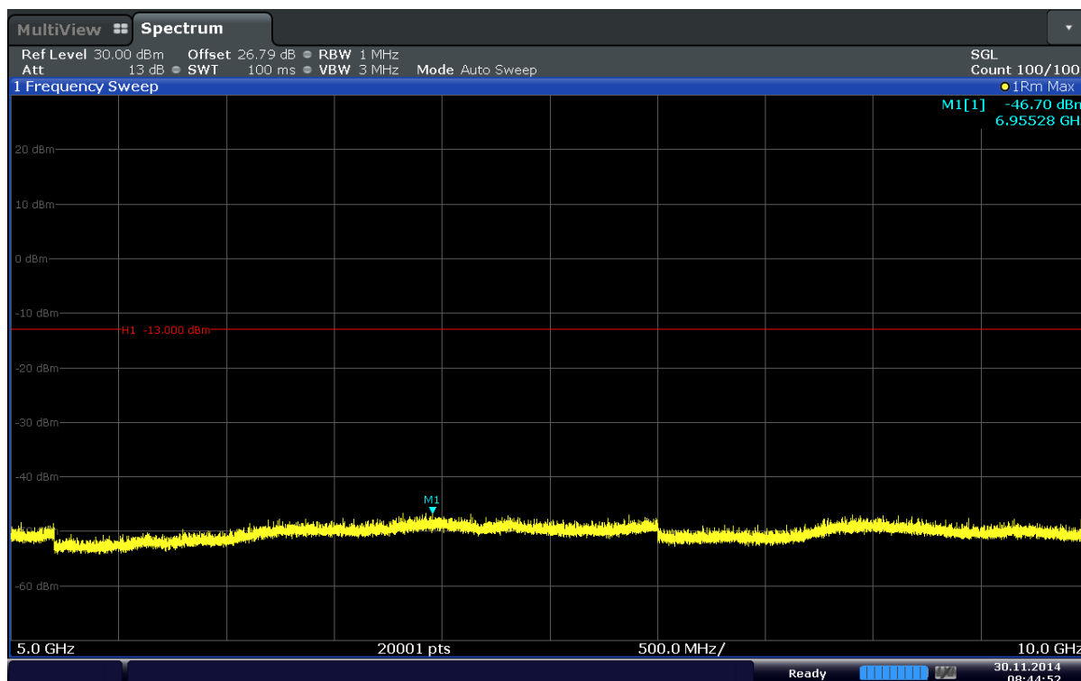
Plot 6-46. Conducted Spurious Plot (Band 5–10.0MHz–QPSK–RB Size 1–RB Offset 0– Ch.20525)
