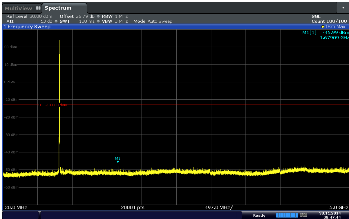
Plot 6-47. Conducted Spurious Plot (Band 5–10.0MHz–QPSK–RB Size 1–RB Offset 0– Ch.20600)
