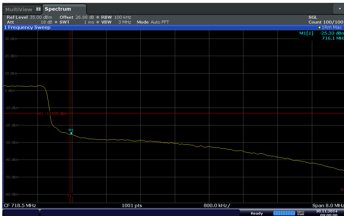
Plot 6-53. Upper Band Edge Plot (Band17 – 10MHz – QPSK – RB Size 50)
