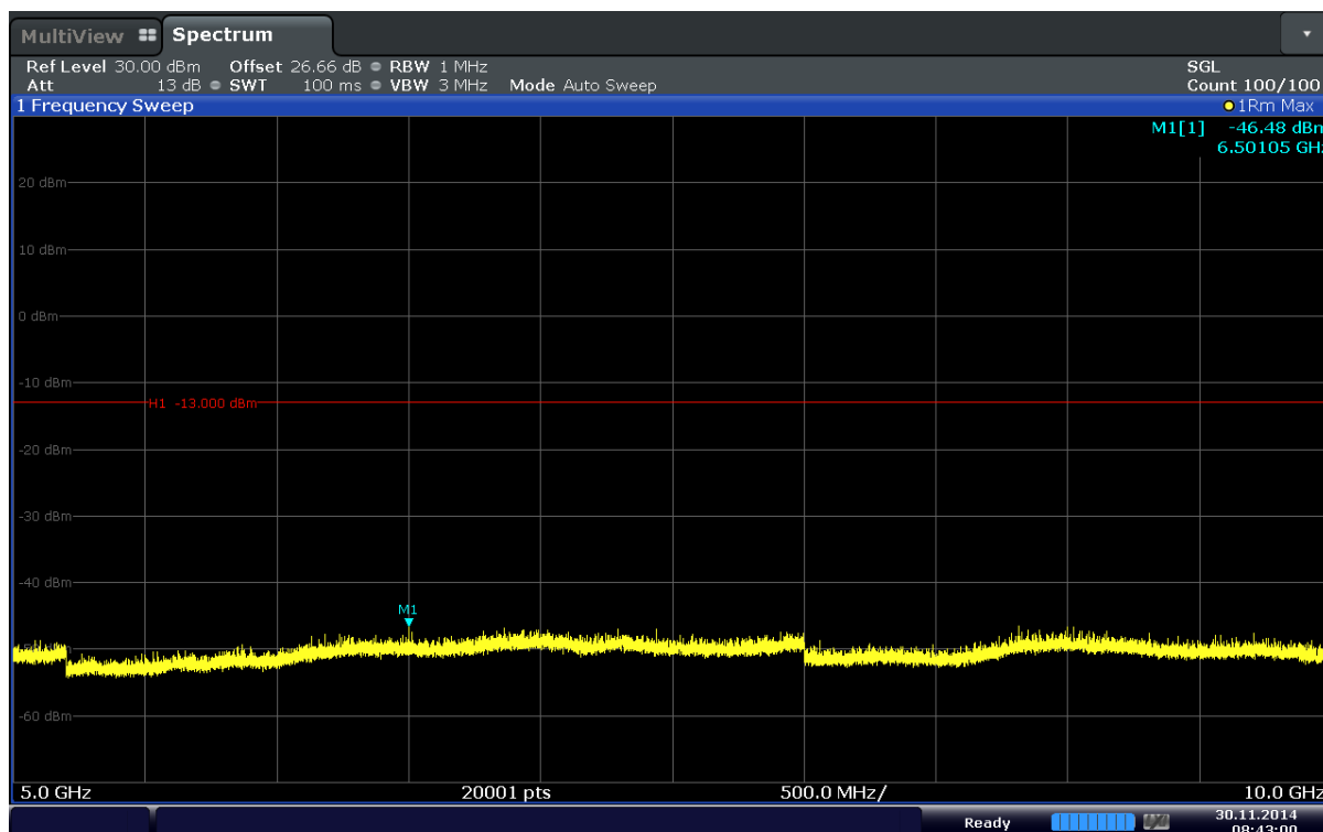
Plot 6-44. Conducted Spurious Plot (Band 5–10.0MHz–QPSK–RB Size 1–RB Offset 0– Ch.20450)
