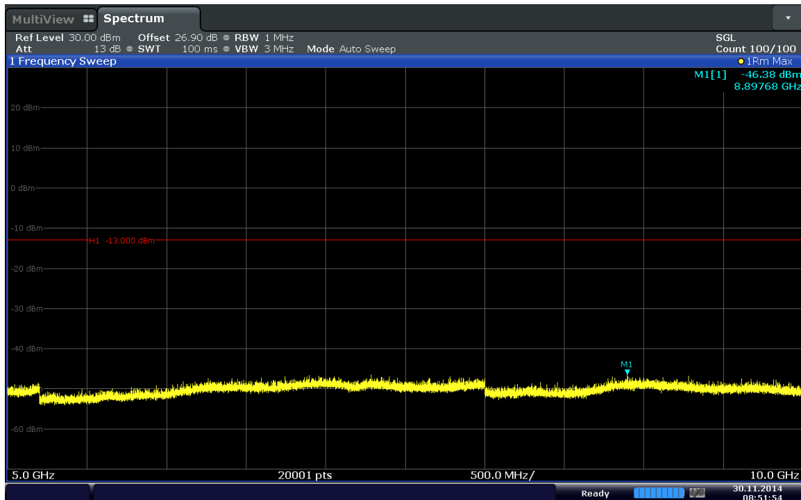
6-16. Conducted Spurious Plot (Band 17–5MHz–QPSK–RB Size 1–RB Offset 12–Ch.23790)
