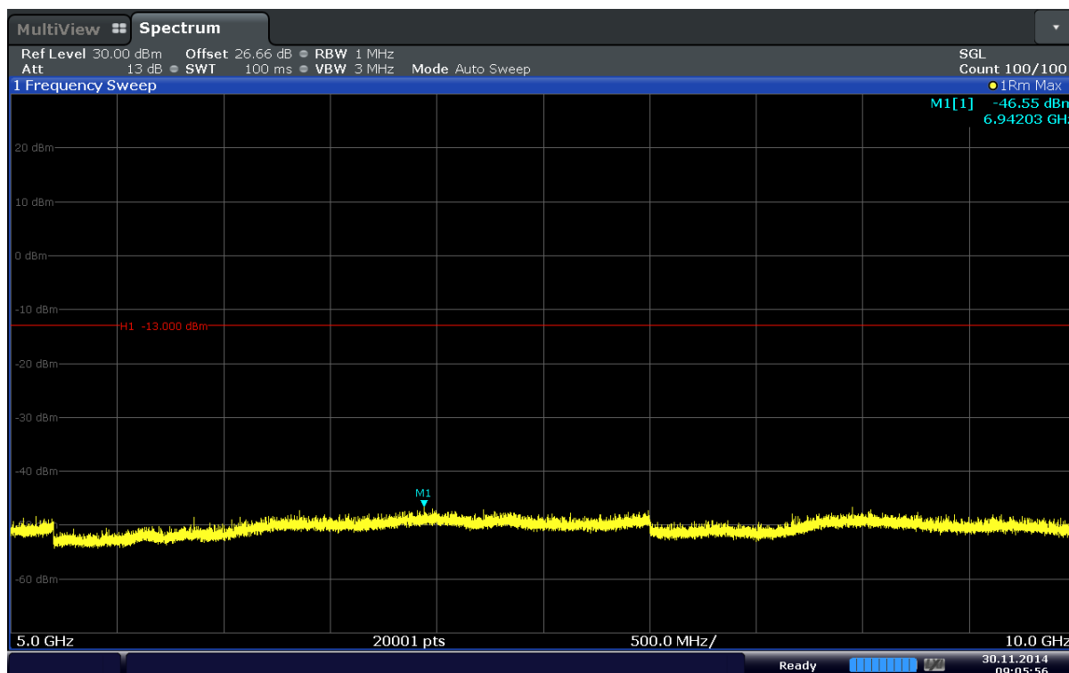
Plot 6-28. Conducted Spurious Plot (Band 5–1.4MHz–QPSK–RB Size 3–RB Offset 3–Ch.20525)
