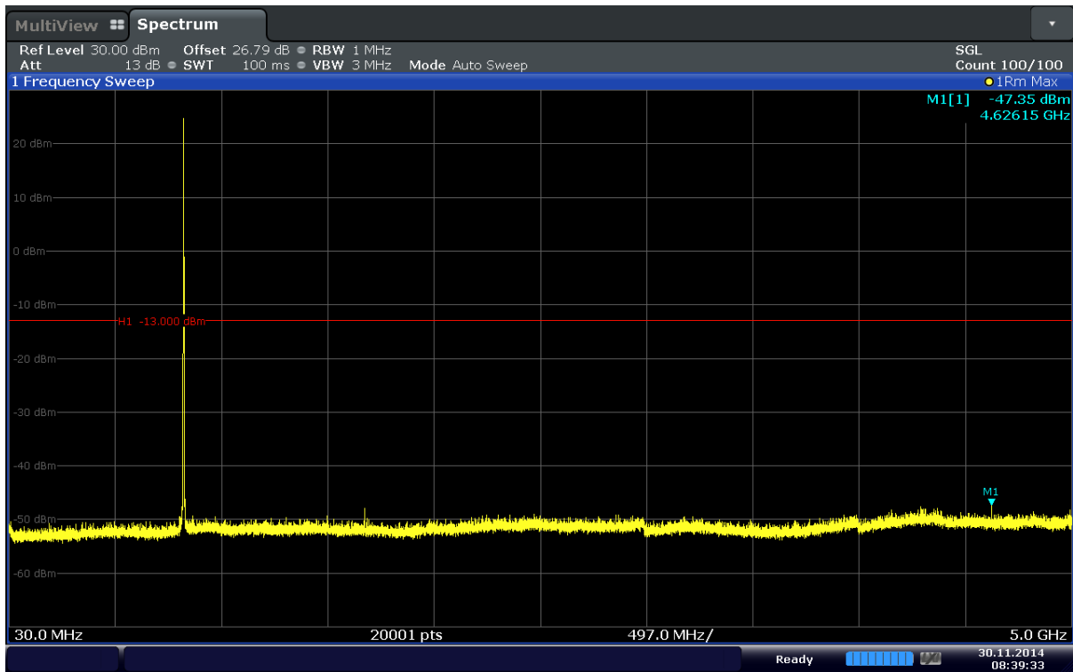
Plot 6-41. Conducted Spurious Plot (Band 5–5.0MHz–QPSK–RB Size 1–RB Offset 12– Ch.20625)
