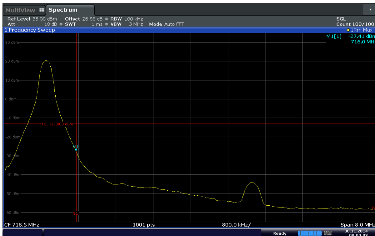
Plot 6-54. Upper Band Edge Plot (Band17 – 10MHz – QPSK – RB Size 1 – RB Offset 49)
