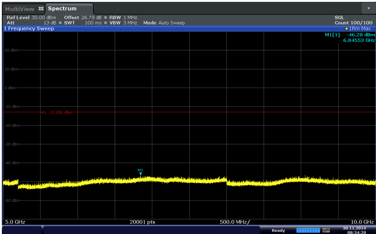
Plot 6-36. Conducted Spurious Plot (Band 5–3.0MHz–QPSK–RB Size 1–RB Offset 7– Ch.20635)
