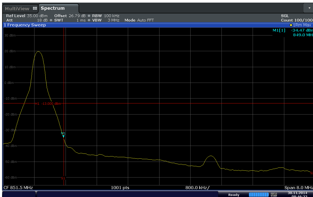
Plot 6-64. Upper Band Edge Plot (Band 5 – 10.0MHz – QPSK – RB Size 1 – RB Offset 49)
