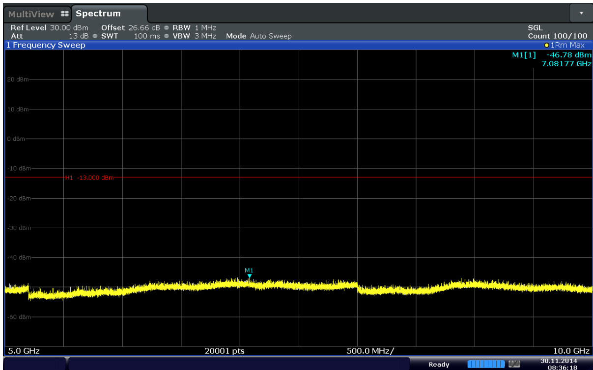
Plot 6-38. Conducted Spurious Plot (Band 5–5.0MHz–QPSK–RB Size 1–RB Offset 12– Ch.20425)
