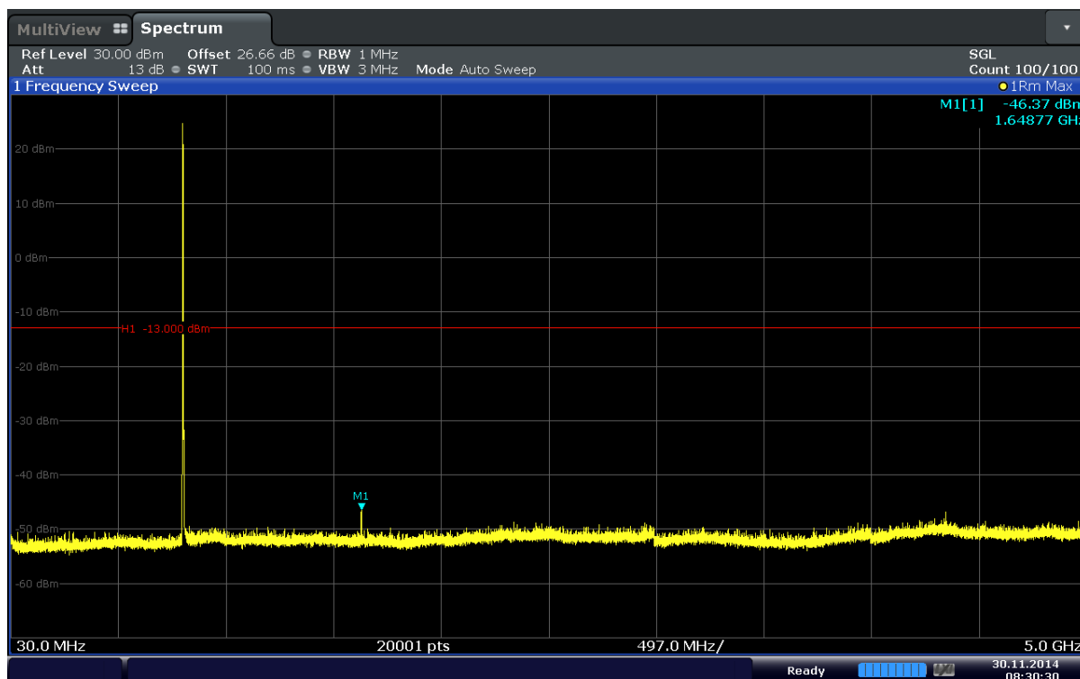
Plot 6-31. Conducted Spurious Plot (Band 5–3.0MHz–QPSK–RB Size 1–RB Offset 0– Ch.20415)
