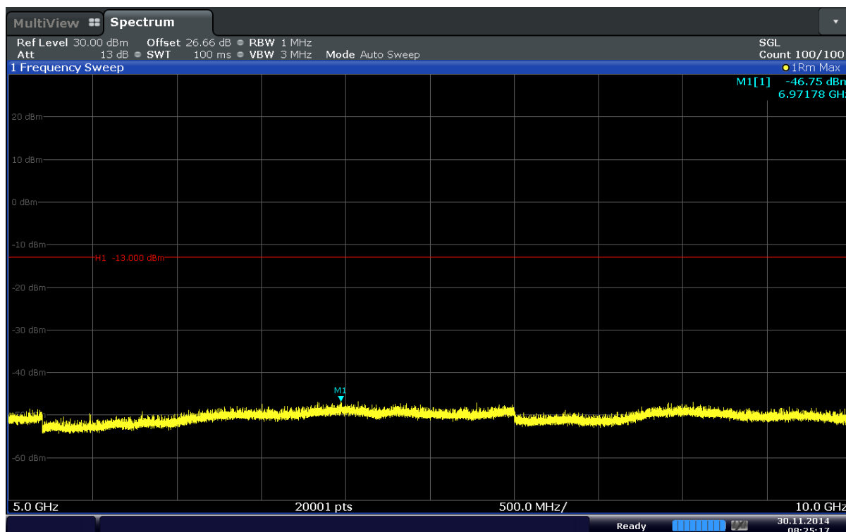
Plot 6-26. Conducted Spurious Plot (Band 5–1.4MHz–QPSK–RB Size 3–RB Offset 2– Ch.20407)
