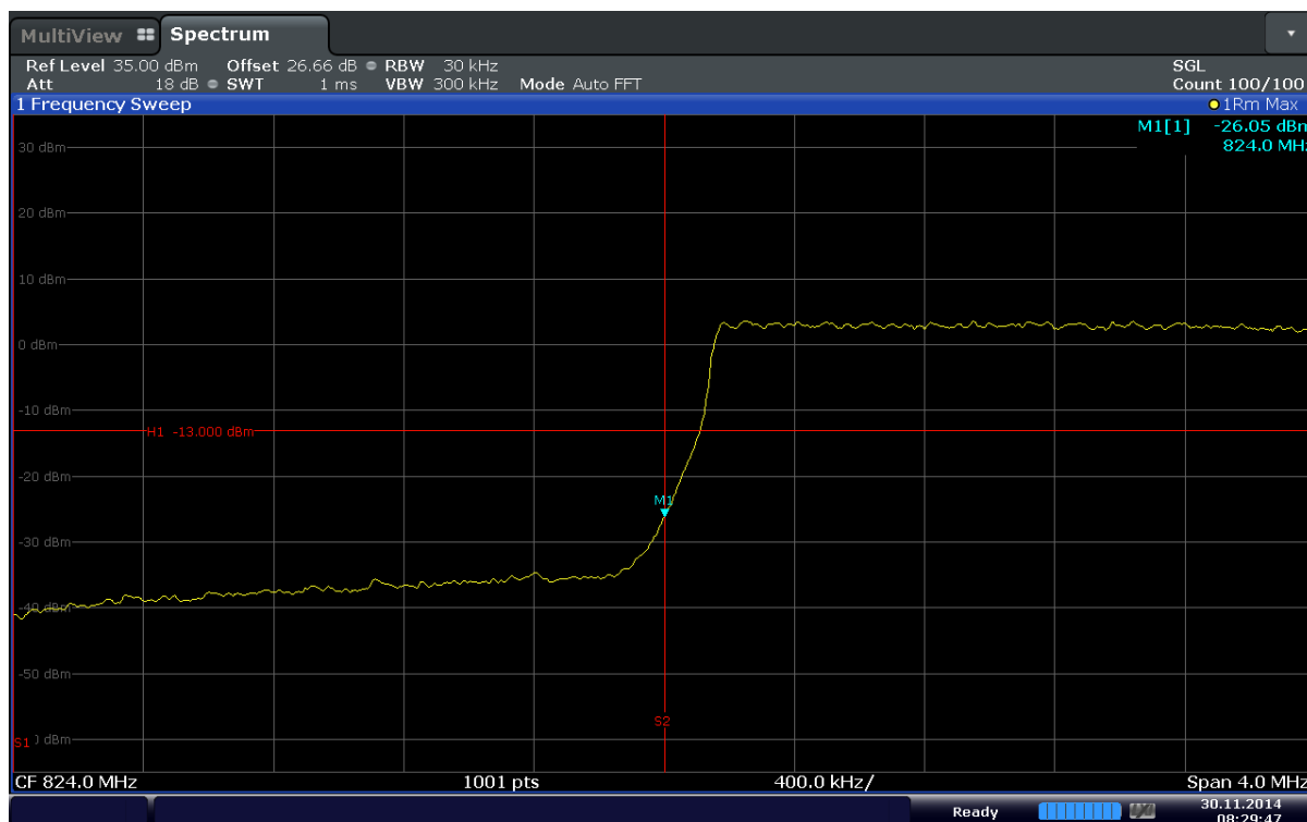
Plot 6-57. Lower Band Edge Plot (Band 5 – 3.0MHz – QPSK – RB Size 15)
