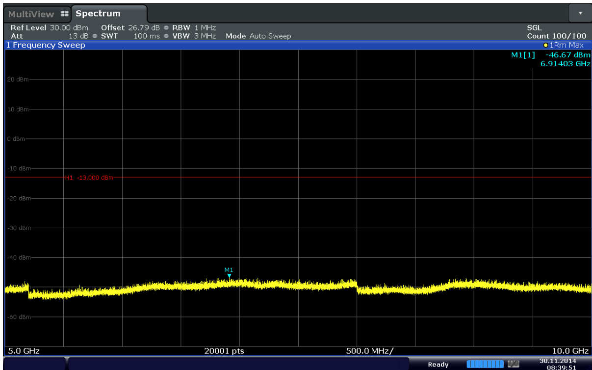
Plot 6-42. Conducted Spurious Plot (Band 5–5.0MHz–QPSK–RB Size 1–RB Offset 12– Ch.20625)
