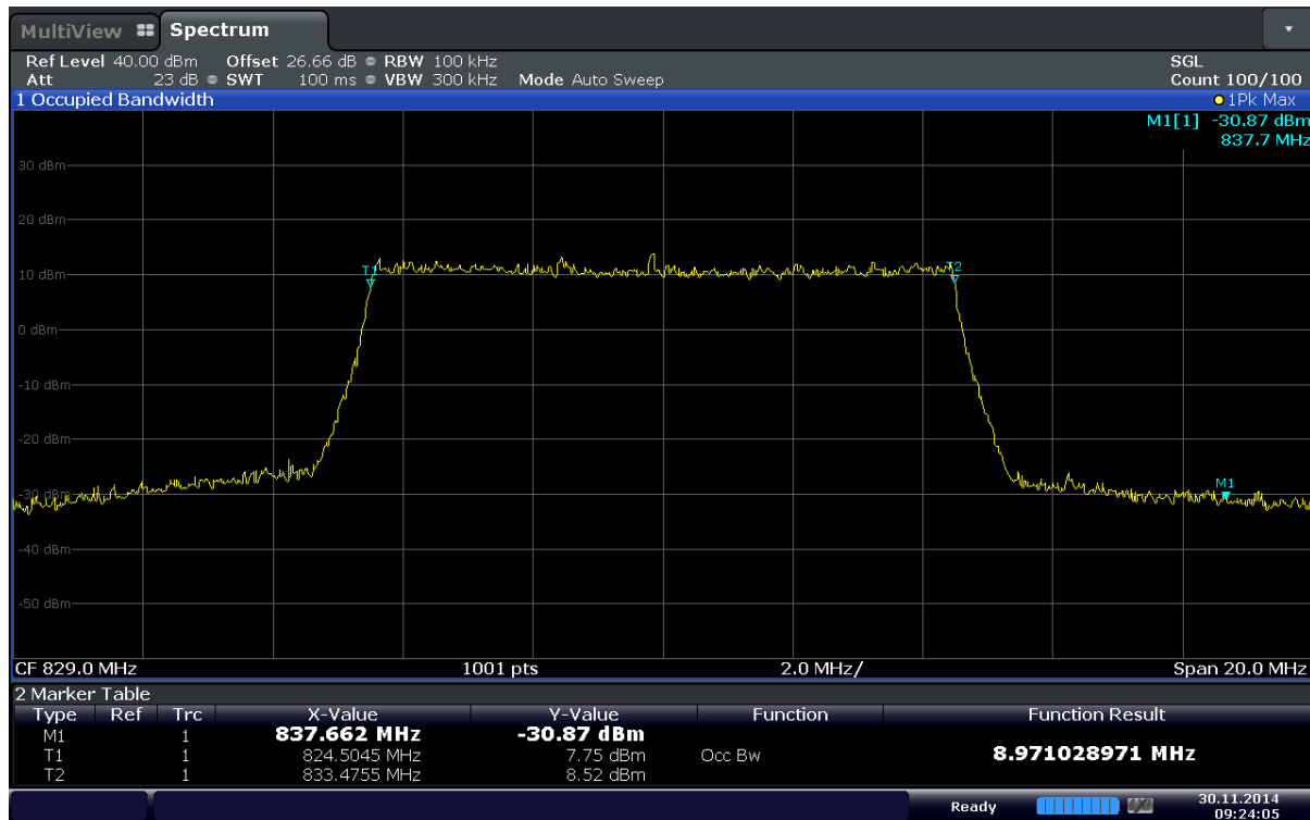
Plot 6-11. Occupied Bandwidth Plot (Band 5 - 10.0MHz QPSK - RB Size 50)
