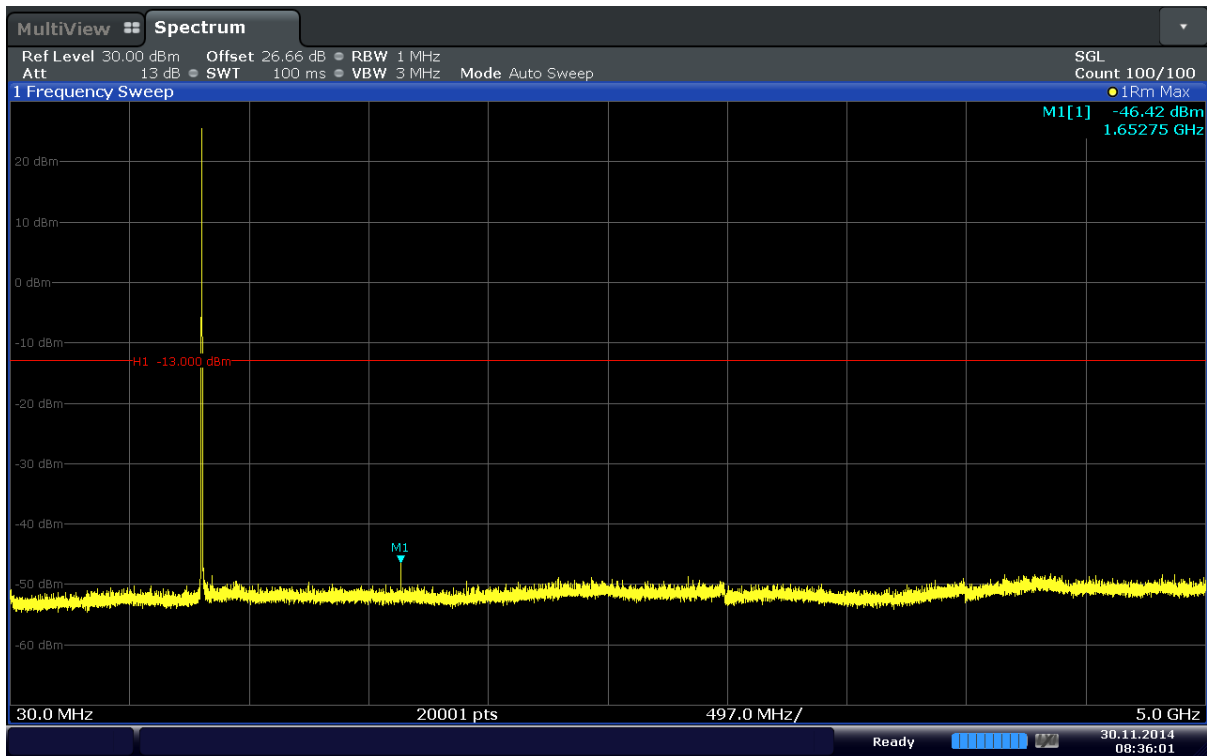
Plot 6-37. Conducted Spurious Plot (Band 5–5.0MHz–QPSK–RB Size 1–RB Offset 12– Ch.20425)
