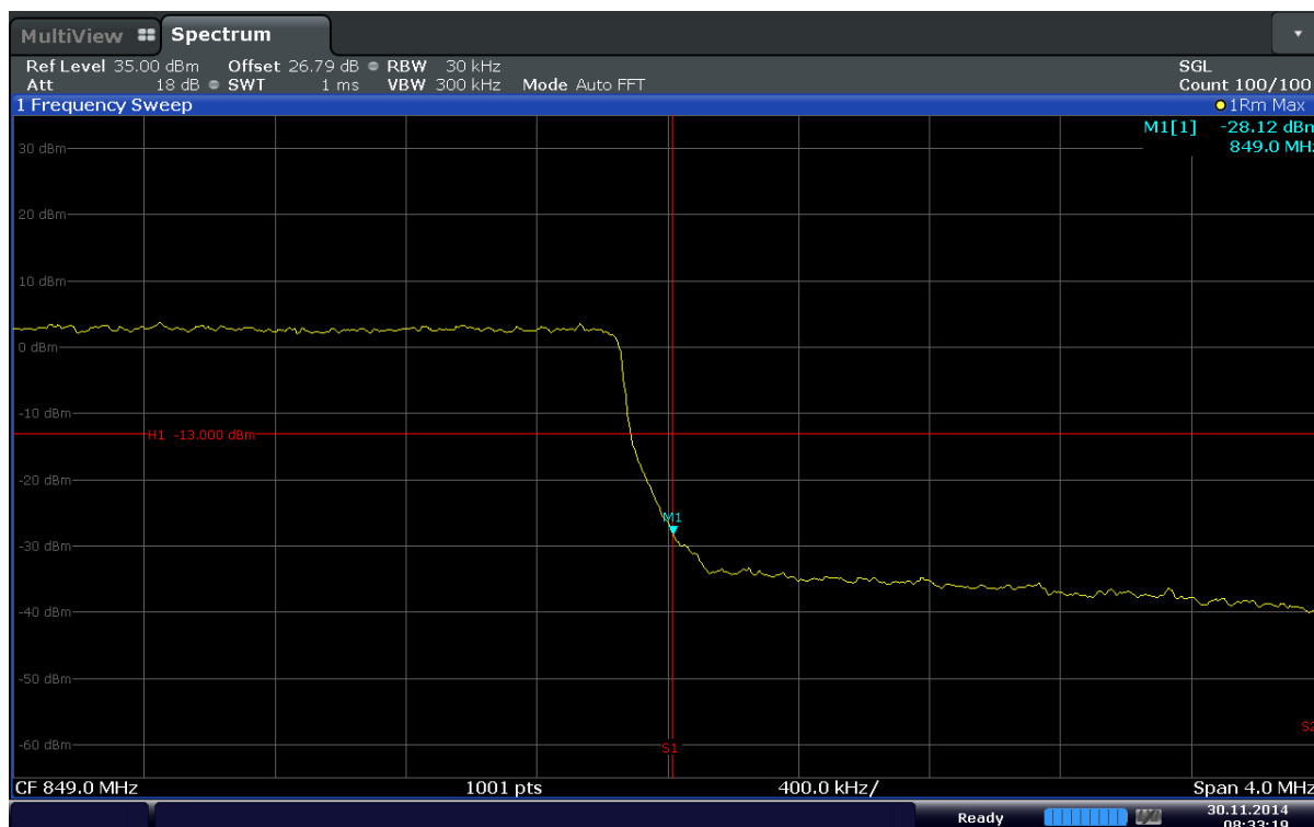
Plot 6-58. Upper Band Edge Plot (Band 5 – 3.0MHz – QPSK – RB Size 15)
