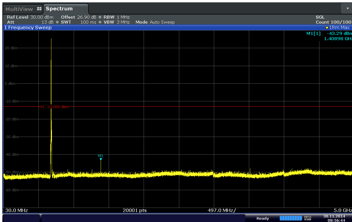
Plot 6-19. Conducted Spurious Plot (Band 17–10MHz–QPSK–RB Size 1–RB Offset 0–Ch.23780)
