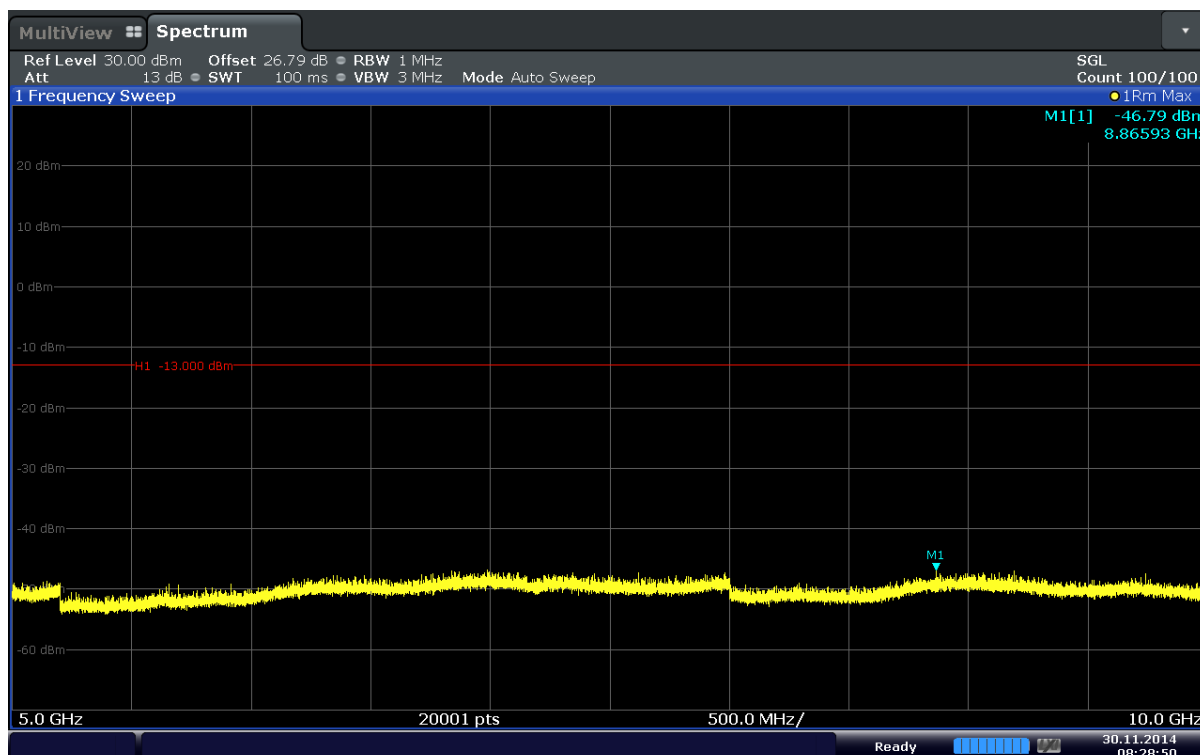
Plot 6-30. Conducted Spurious Plot (Band 5–1.4MHz–QPSK–RB Size 3–RB Offset 3– Ch.20643)
