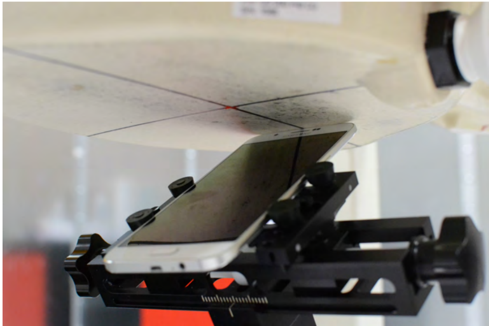
SAR Test Setup Photo 6: Mouth-Jaw Replacing Left Tilt
