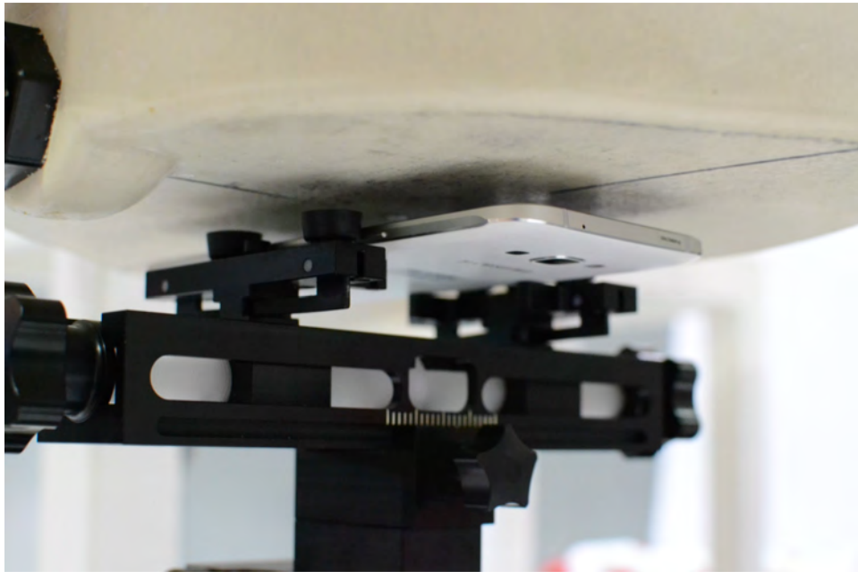
SAR Test Setup Photo 10: Front Side at 1.0 cm
