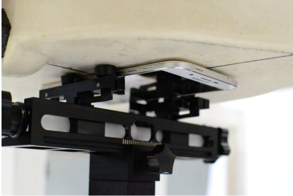
SAR Test Setup Photo 9: Back Side at 0.0 cm
