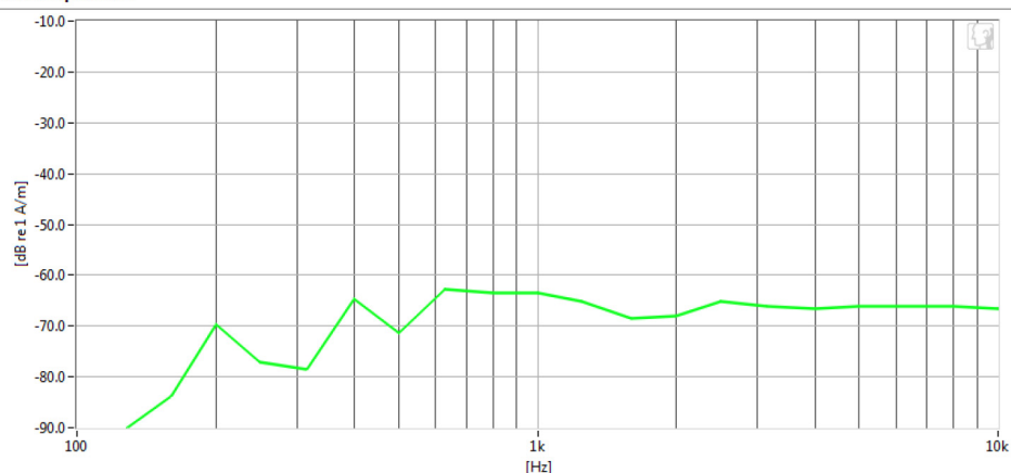
Noise Spectrum
