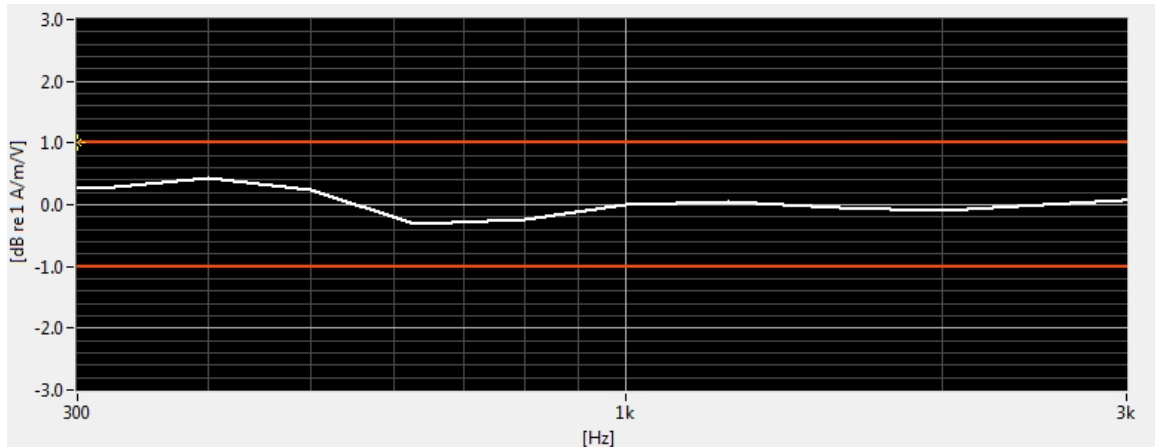
Figure 7-3 Helmholtz Coil Validation for Frequency Response
