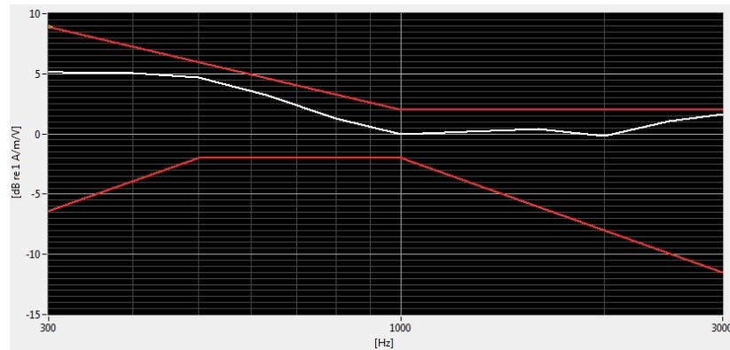
Figure 7-1 Axial Frequency Response
