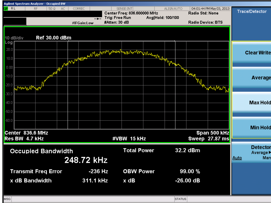
Plot 7-13. Occupied Bandwidth Plot (EDGE850 Mode – Ch. 190)
