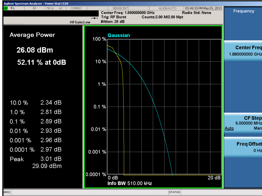
Plot 7-25. Peak-Average Ratio Plot (EDGE1900 Mode – Ch. 661)
