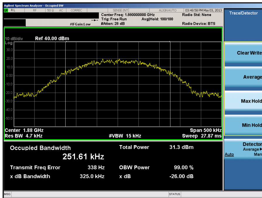
Plot 7-24. Occupied Bandwidth Plot (EDGE1900 Mode – Ch. 661)
