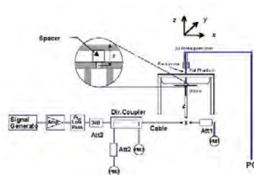
Figure 10-1 System Verification Setup Diagram
