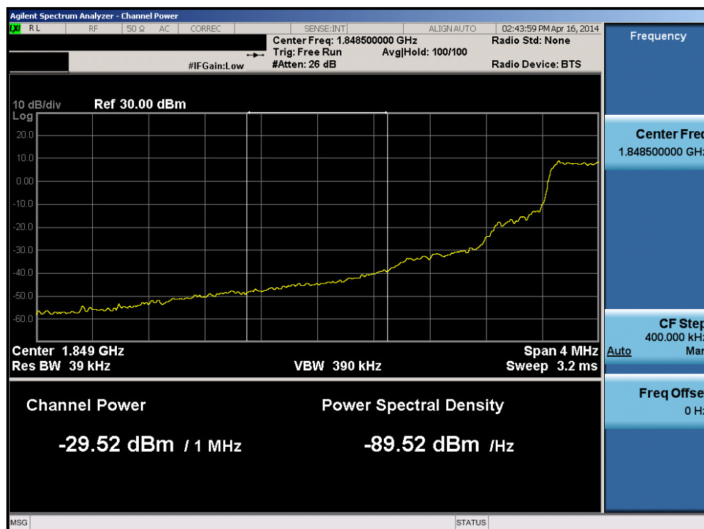
Plot 6-193. Lower Extended Band Edge Plot (Band 2 – 1.4MHz QPSK – RB Size 6)
