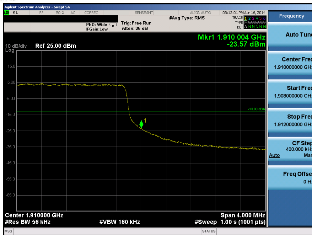
Plot 6-202. Upper Band Edge Plot (Band 2 – 5.0MHz QPSK – RB Size 25)
