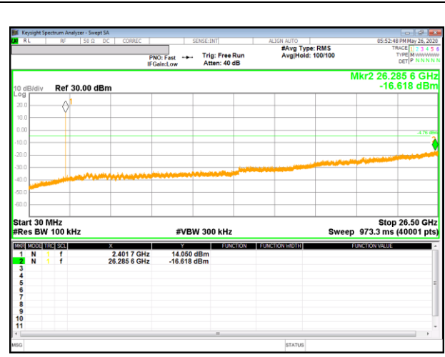
OUT-OF-BAND 0 CHANNEL
