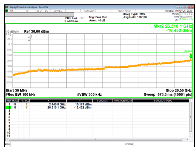
OUT-OF-BAND 39 CHANNEL
