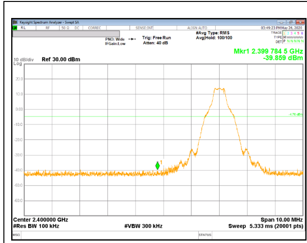
0 CHANNEL BANDEDGE
