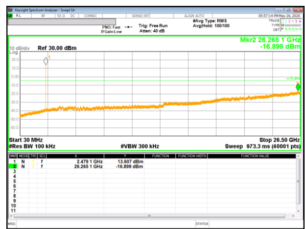
OUT-OF-BAND 77 CHANNEL
