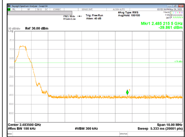
77 CHANNEL BANDEDGE
