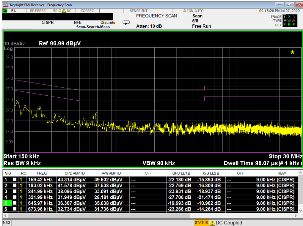
Plot 7-6. Line-Conducted Test Plot (L1)
