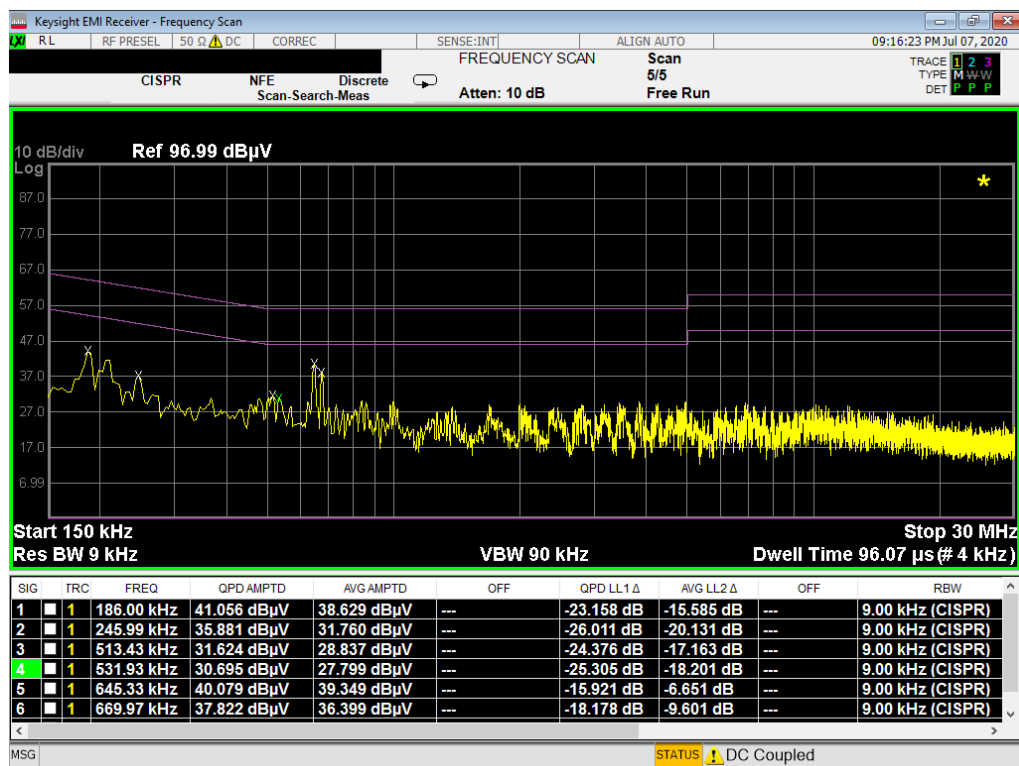
Plot 7-7. Line-Conducted Test Plot (N)
