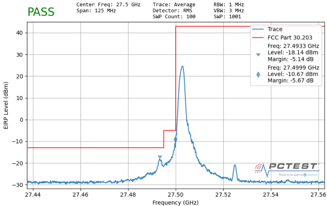
Plot 7-122. Ant1 Lower Band Edge (50MHz-1CC – \pi/2 -BPSK 1 RB)
