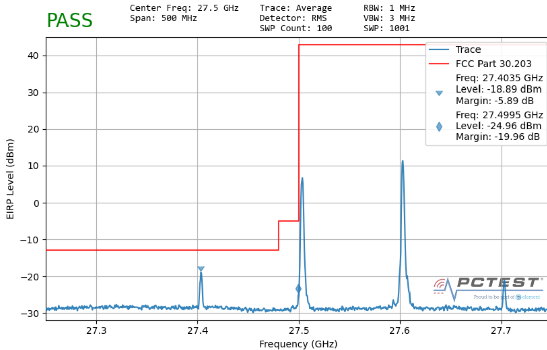
Plot 7-127. Ant1 Lower Band Edge (100MHz-2CC – QPSK 1 RB)
