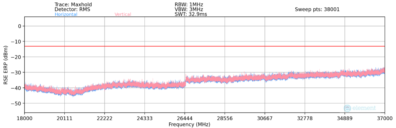
Plot 7-100. Ant1 - n260 Radiated Spurious Plot (1CC QPSK Mid Channel 2Tx – EN-DC Anchor Band 2)
