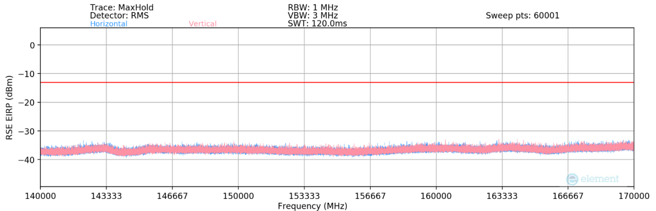
Plot 7-104. Ant1 - n260 Radiated Spurious Plot (1CC QPSK Mid Channel 2Tx – EN-DC Anchor Band 2)
