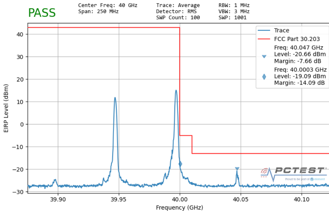
Plot 7-133. Ant1 Upper Band Edge (50MHz-2CC – QPSK 1 RB)
