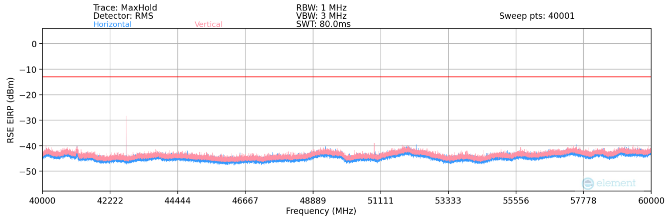
Plot 7-101. Ant1 - n260 Radiated Spurious Plot (1CC QPSK Mid Channel 2Tx – EN-DC Anchor Band 2)
