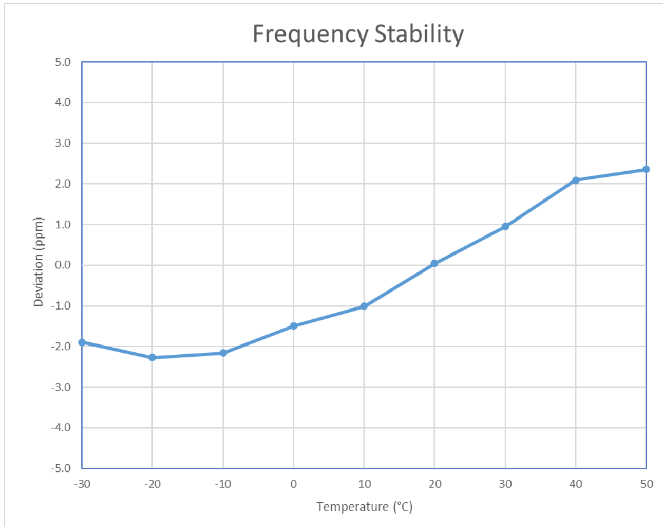
Figure 7-3. Frequency Stability Graph (n260)
