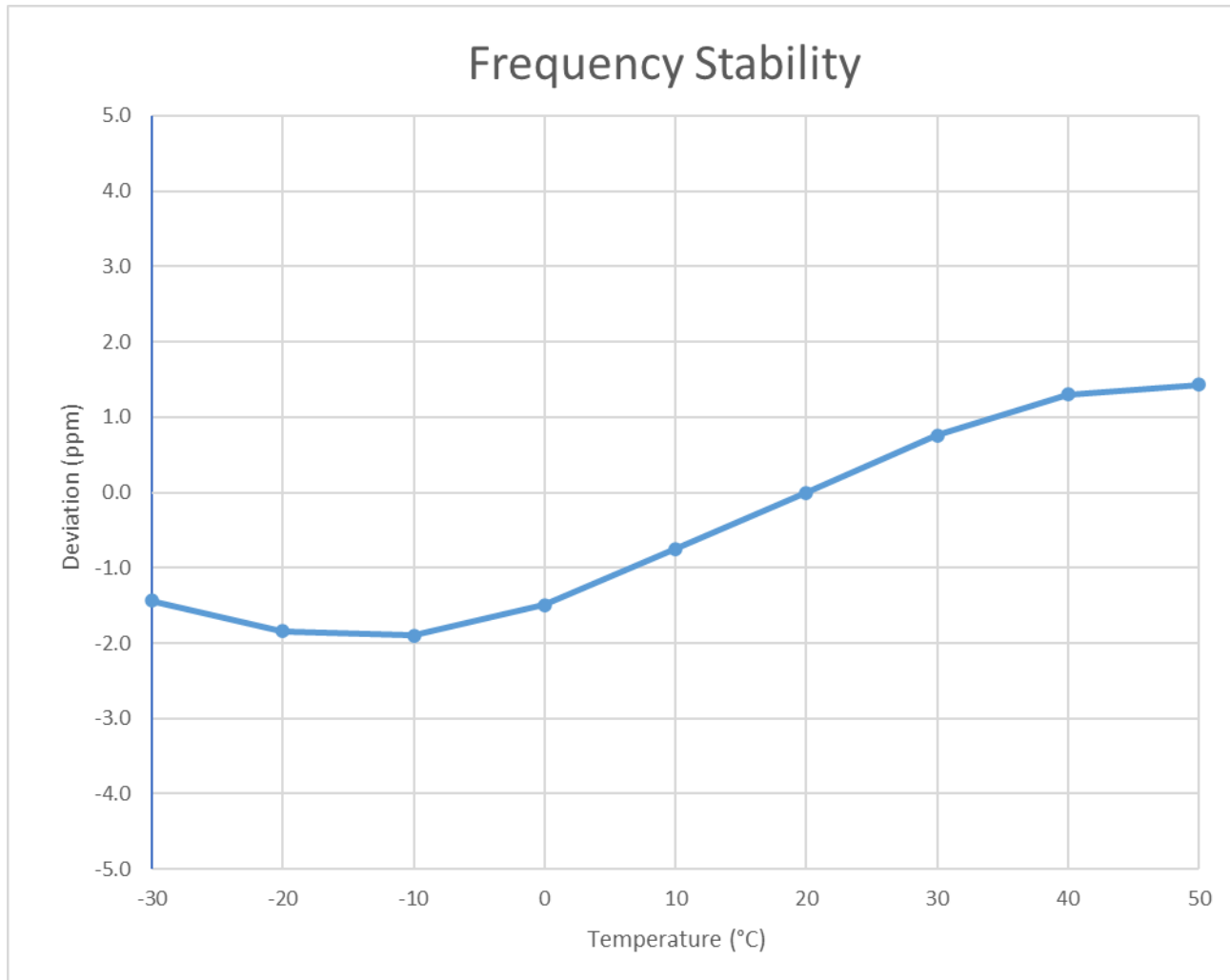
Figure 7-1. Frequency Stability Graph (n258)
