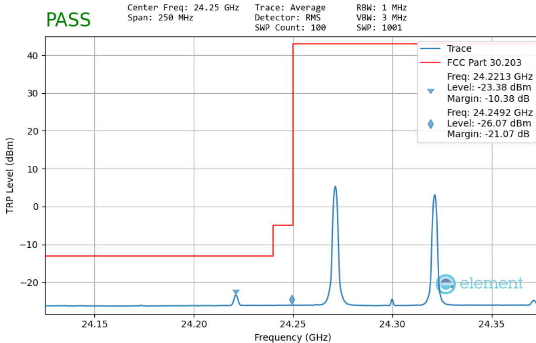
Plot 7-107. Ant1 Lower Band Edge – TRP (50MHz-2CC – QPSK 1 RB)
