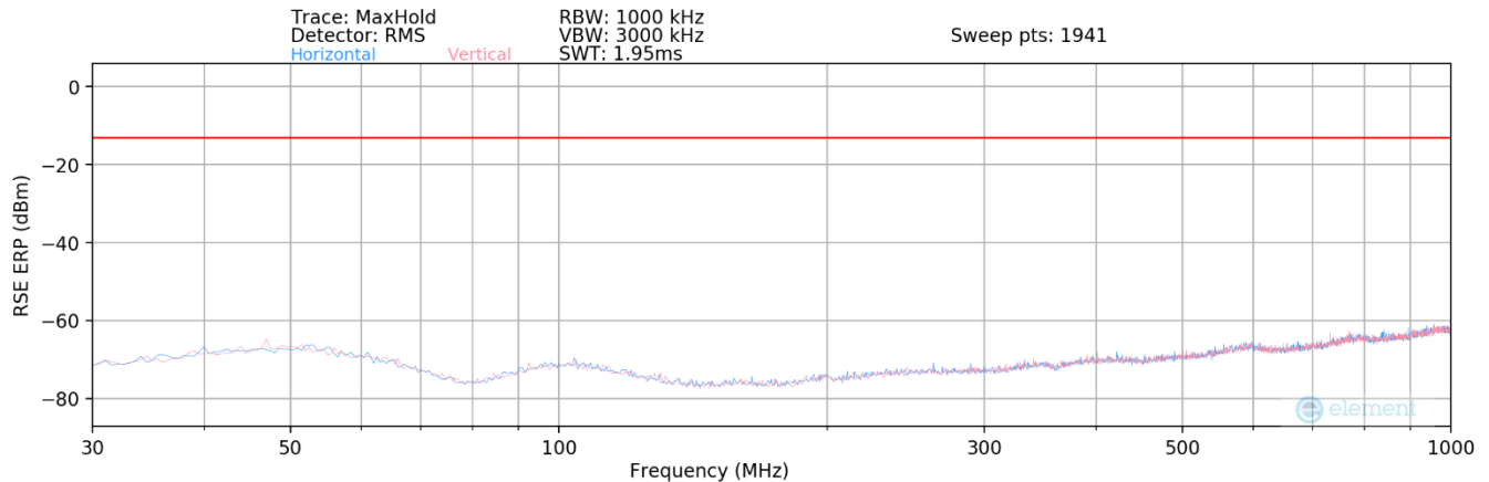
Plot 7-98. Ant1 - n260 Radiated Spurious Plot (1CC QPSK Mid Channel 2Tx – EN-DC Anchor Band 2)
