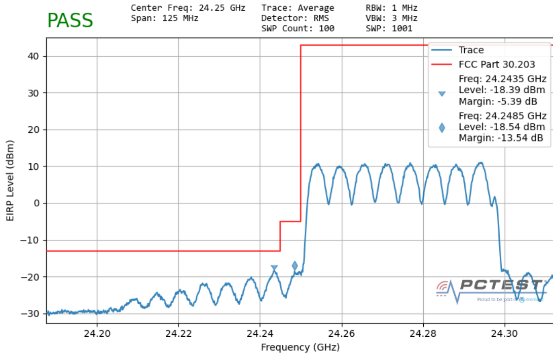
Plot 7-106. Ant1 Lower Band Edge (50MHz-1CC – QPSK Full RB)
