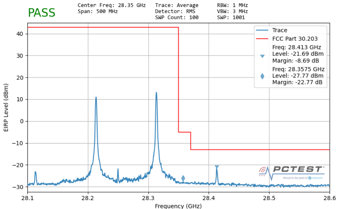
Plot 7-129. Ant1 Upper Band Edge (100MHz-2CC – QPSK 1 RB)
