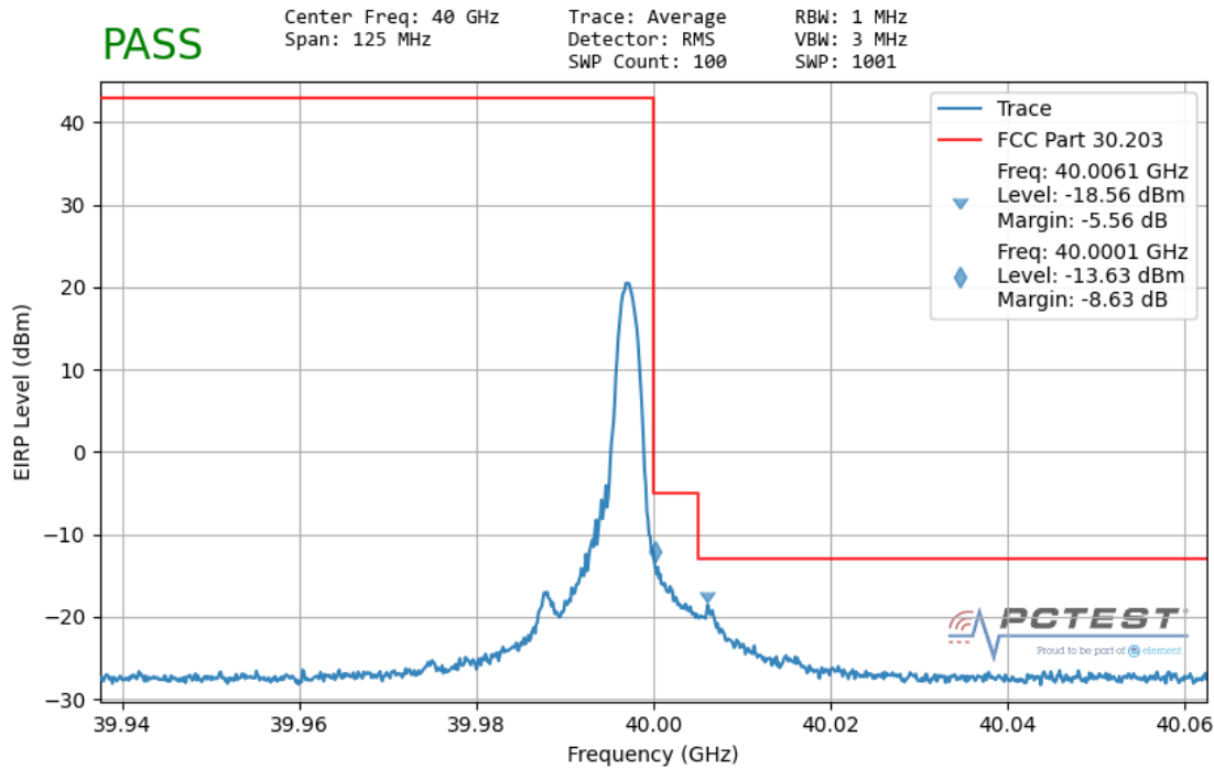
Plot 7-132. Ant1 Upper Band Edge (50MHz-1CC – \pi/2 -BPSK 1 RB)
