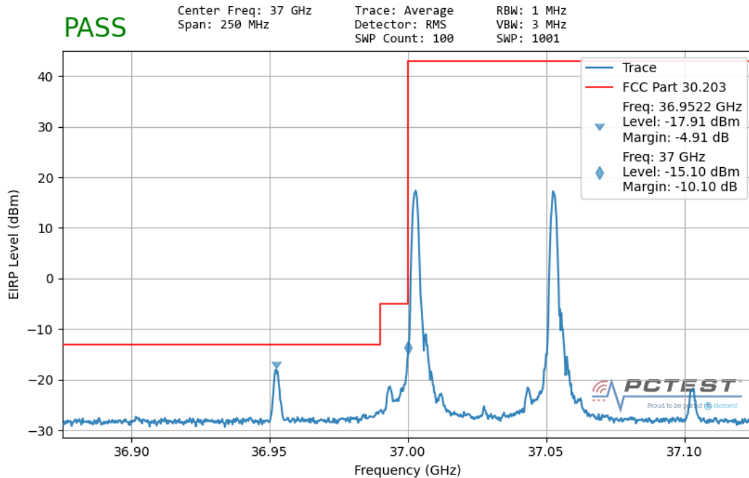
Plot 7-131. Ant1 Lower Band Edge (50MHz-2CC – QPSK 1 RB)
