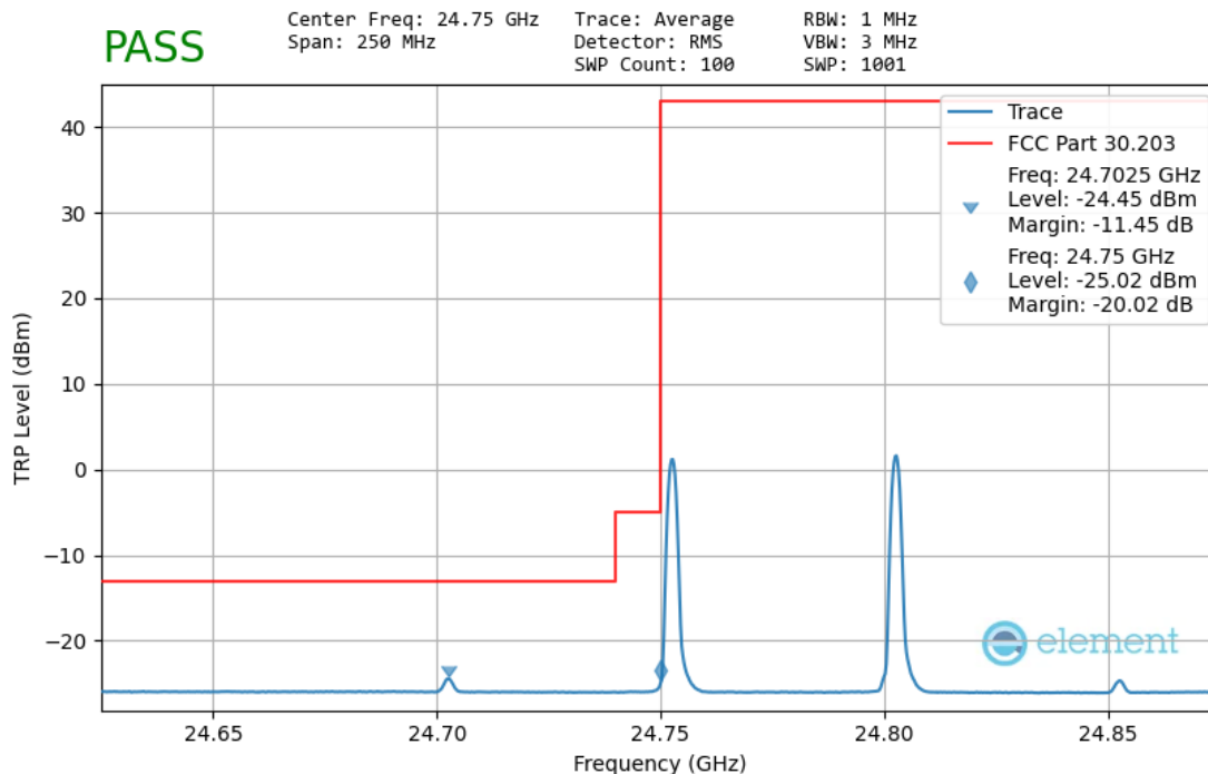
Plot 7-115. Ant1 Lower Band Edge – TRP (50MHz-2CC – QPSK 1 RB)
