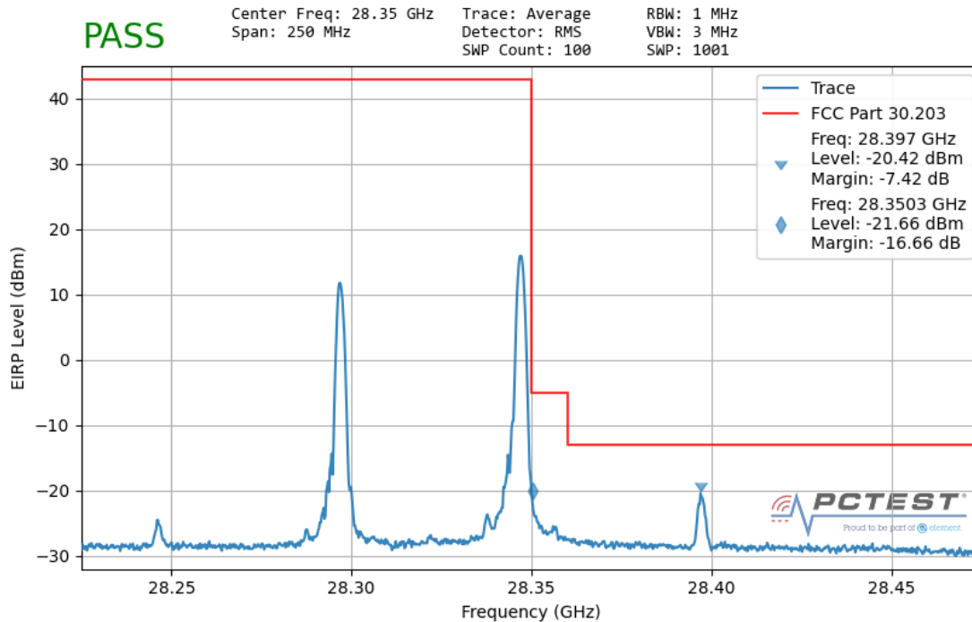
Plot 7-125. Ant1 Upper Band Edge (50MHz-2CC – QPSK 1 RB)
