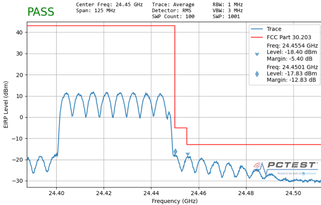
Plot 7-108. Ant1 Upper Band Edge (50MHz-1CC – QPSK Full RB)
