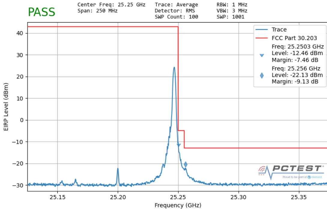
Plot 7-120. Ant1 Upper Band Edge (100MHz-1CC – QPSK 1 RB)
