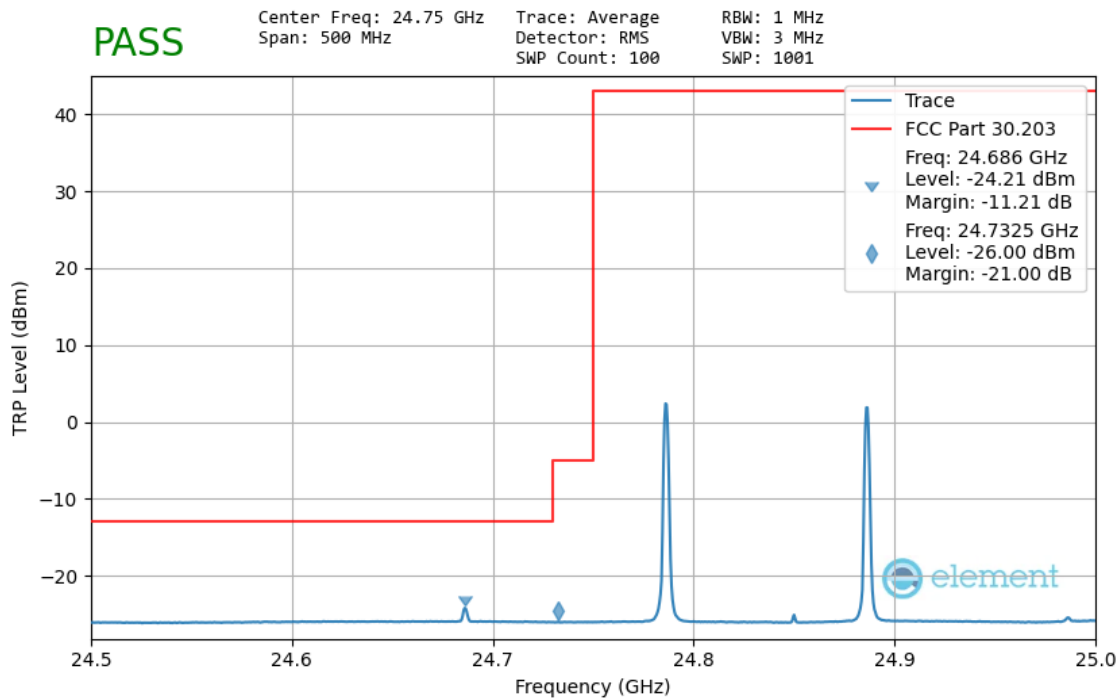
Plot 7-119. Ant1 Lower Band Edge – TRP (100MHz-2CC – QPSK 1 RB)
