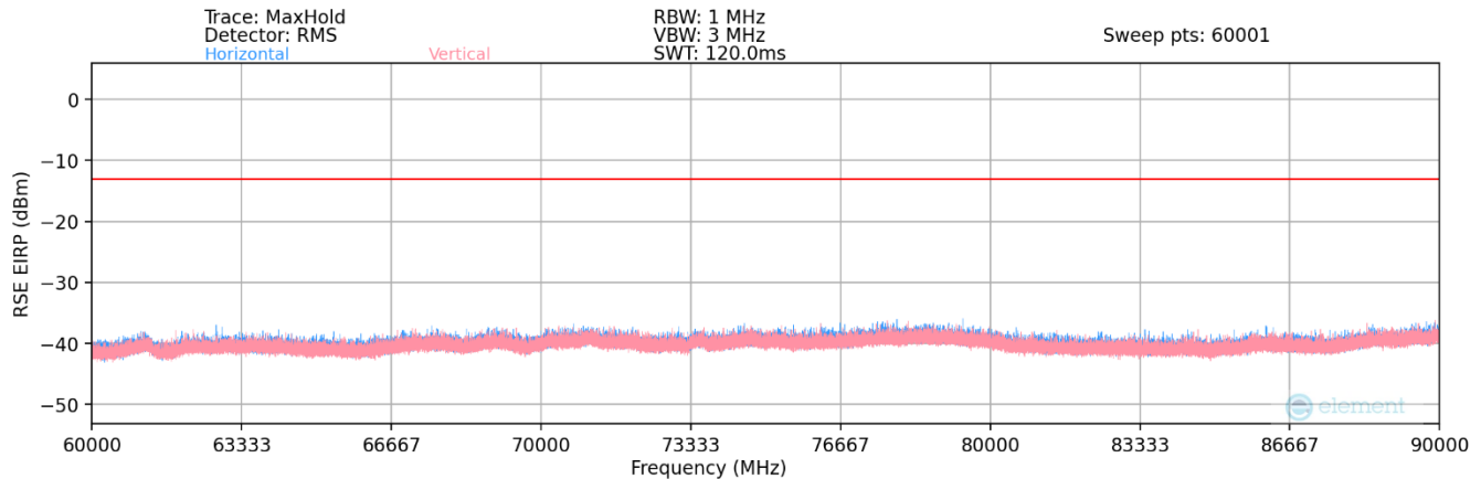
Plot 7-102. Ant1 - n260 Radiated Spurious Plot (1CC QPSK Mid Channel 2Tx – EN-DC Anchor Band 2)
