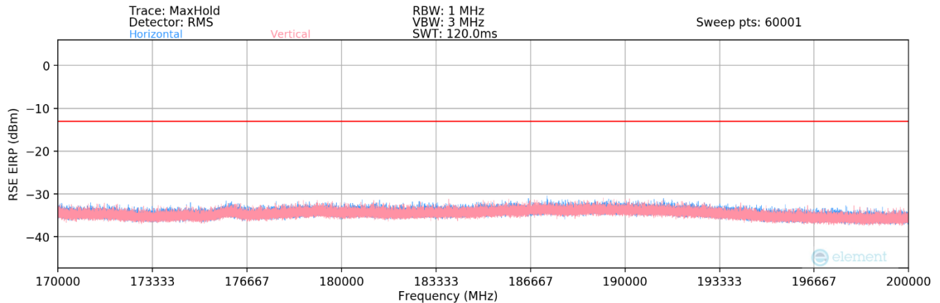
Plot 7-105. Ant1 - n260 Radiated Spurious Plot (1CC QPSK Mid Channel 2Tx – EN-DC Anchor Band 2)
