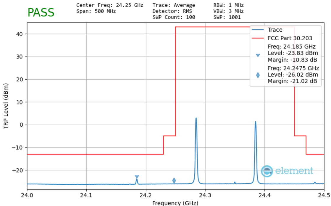
Plot 7-111. Ant1 Lower Band Edge – TRP (100MHz-2CC – QPSK 1 RB)
