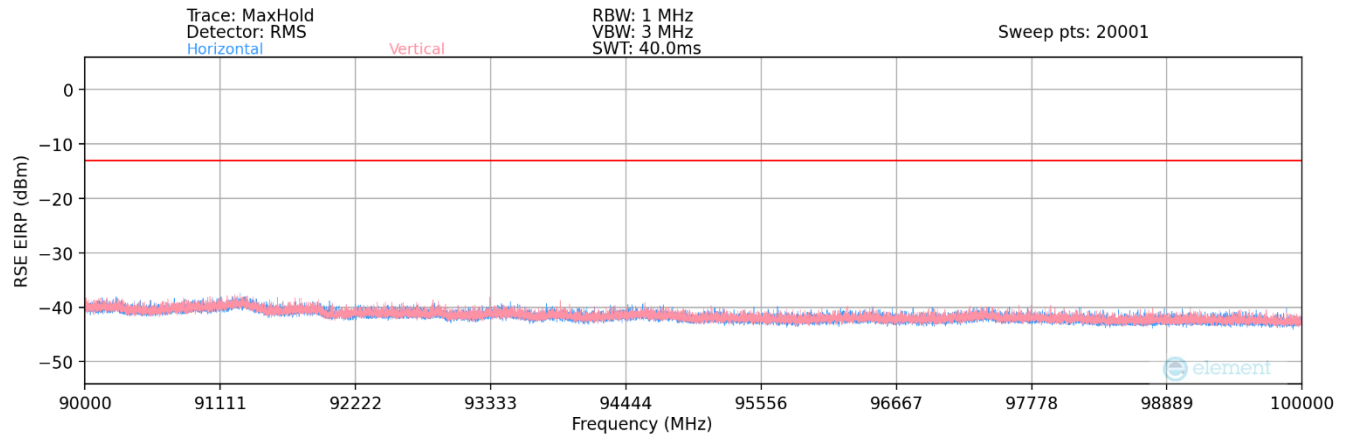
Plot 7-97. Ant1 - n261 Radiated Spurious Plot (1CC QPSK Mid Channel 2Tx - EN-DC Anchor Band 2)
