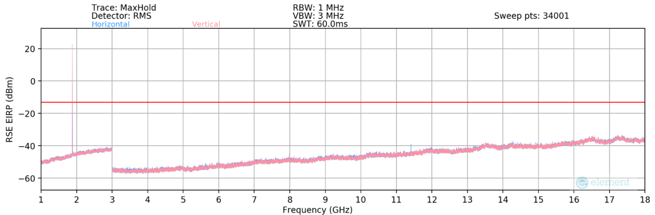
Plot 7-99. Ant1 - n260 Radiated Spurious Plot (1CC QPSK Mid Channel 2Tx – EN-DC Anchor Band 2)
