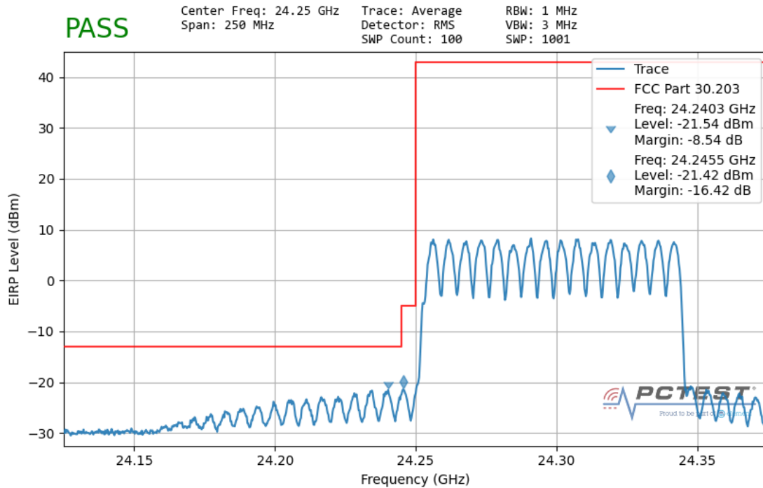
Plot 7-110. Ant1 Lower Band Edge (100MHz-1CC – QPSK Full RB)
