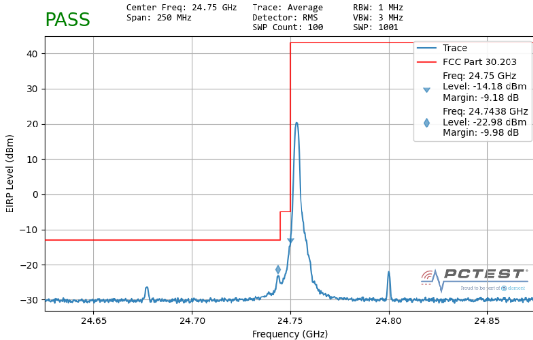
Plot 7-118. Ant1 Lower Band Edge (100MHz-1CC – QPSK 1 RB)
