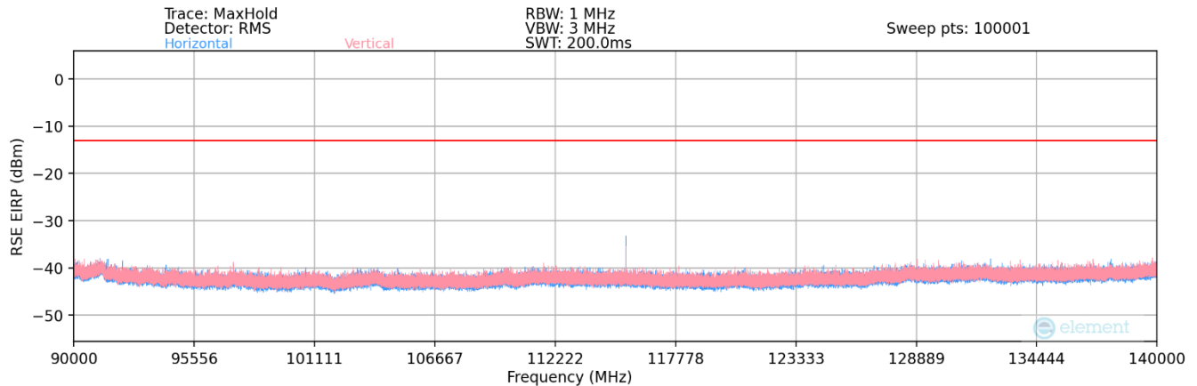
Plot 7-103. Ant1 - n260 Radiated Spurious Plot (1CC QPSK Mid Channel 2Tx – EN-DC Anchor Band 2)
