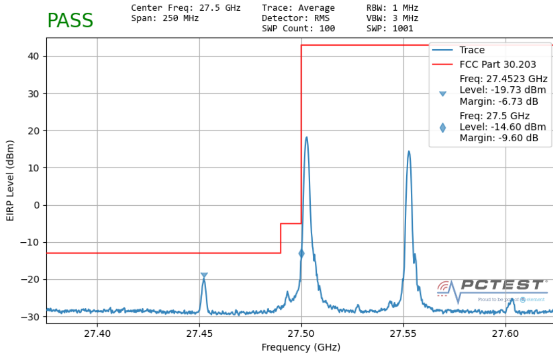
Plot 7-123. Ant1 Lower Band Edge (50MHz-2CC – QPSK 1 RB)
