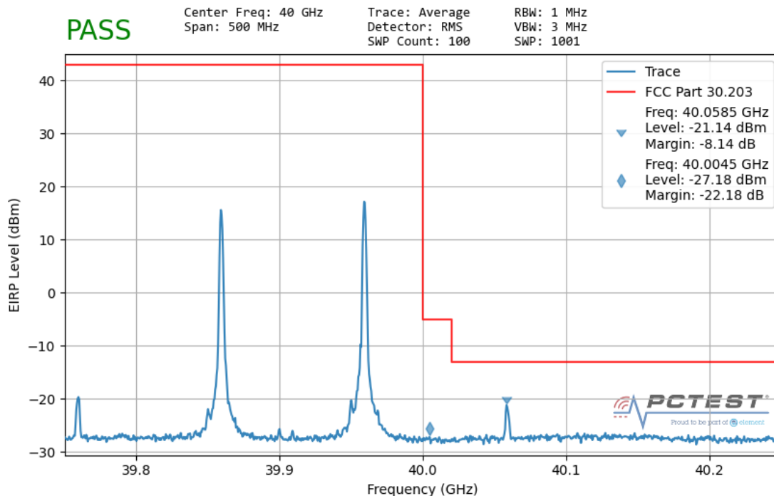
Plot 7-137. Ant1 Upper Band Edge (100MHz-2CC – QPSK 1 RB)
