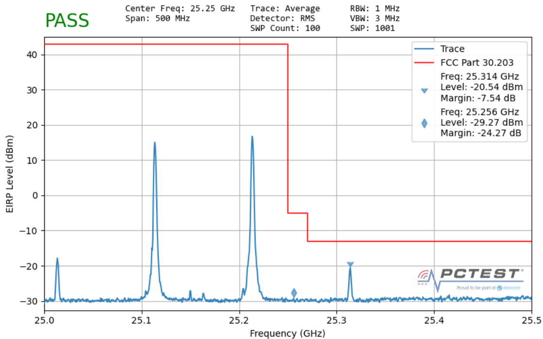
Plot 7-121. Ant1 Upper Band Edge (100MHz-2CC – QPSK 1 RB)
