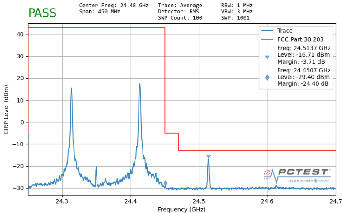
Plot 7-113. Ant1 Upper Band Edge (100MHz-2CC – QPSK 1 RB)
