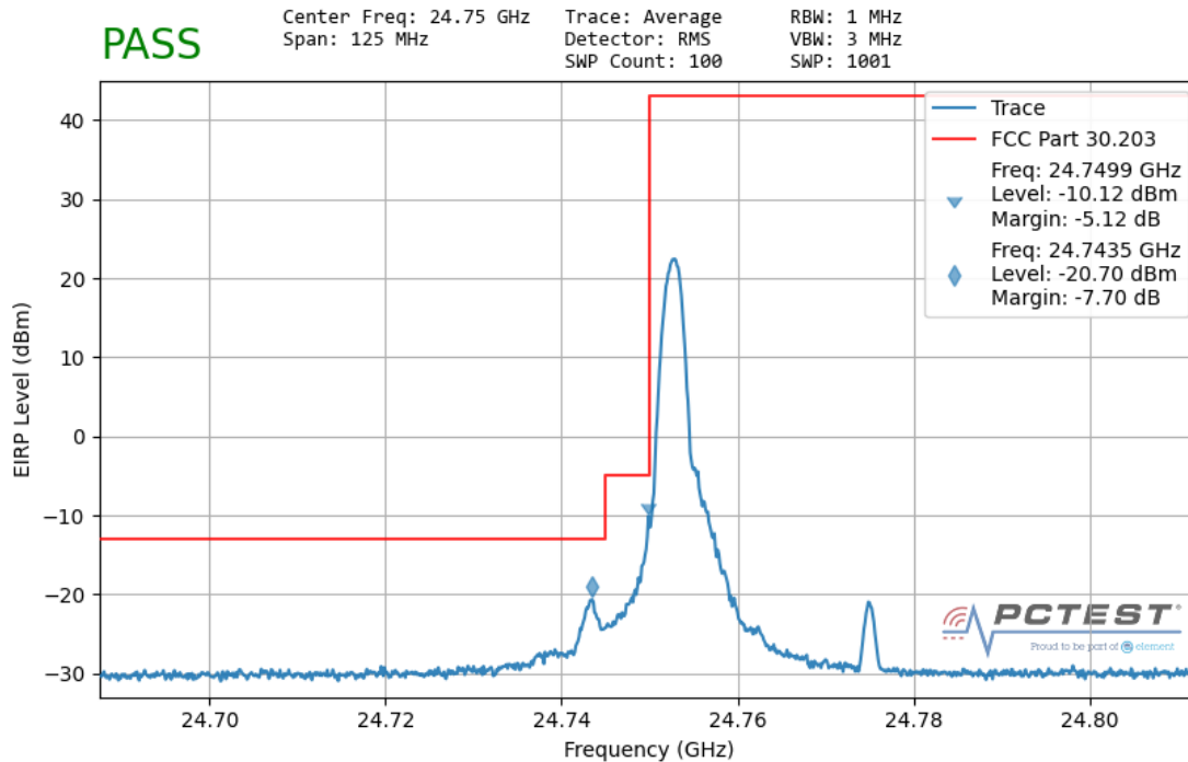
Plot 7-114. Ant1 Lower Band Edge (50MHz-1CC – \pi/2 -BPSK 1 RB)
