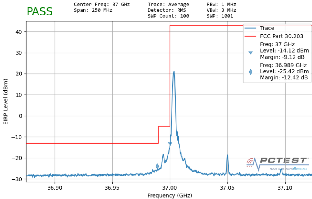
Plot 7-134. Ant1 Lower Band Edge (100MHz-1CC – \pi/2 -BPSK 1 RB)
