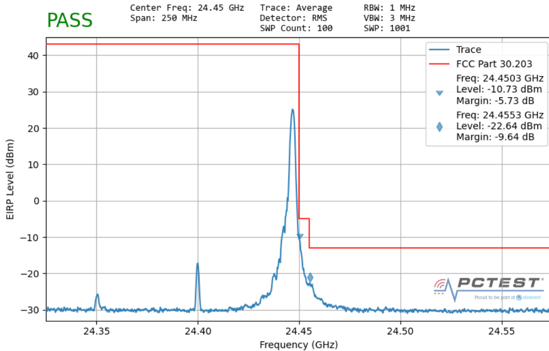
Plot 7-112. Ant1 Upper Band Edge (100MHz-1CC – \pi/2 -BPSK 1 RB)
