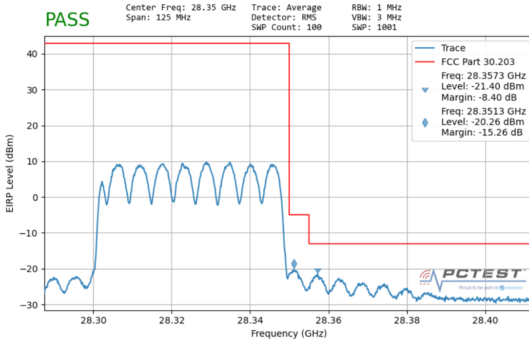
Plot 7-124. Ant1 Upper Band Edge (50MHz-1CC – QPSK Full RB)
