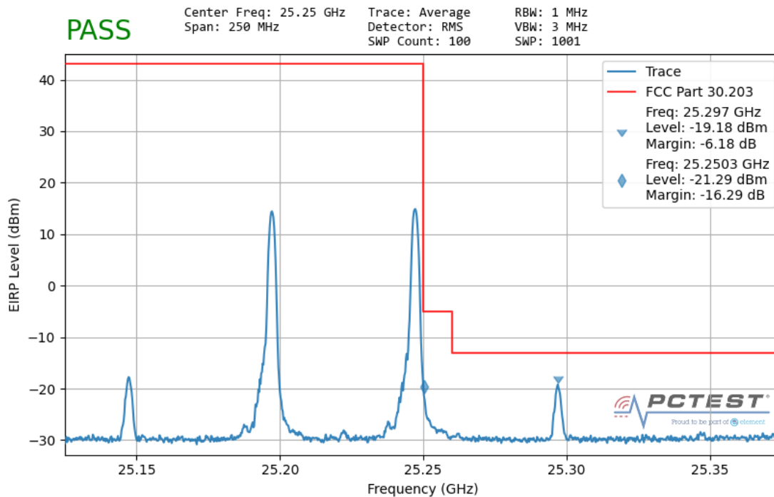
Plot 7-117. Ant1 Upper Band Edge (50MHz-2CC – QPSK 1 RB)
