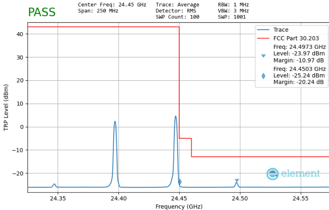
Plot 7-109. Ant1 Upper Band Edge – TRP (50MHz-2CC – QPSK 1 RB)
