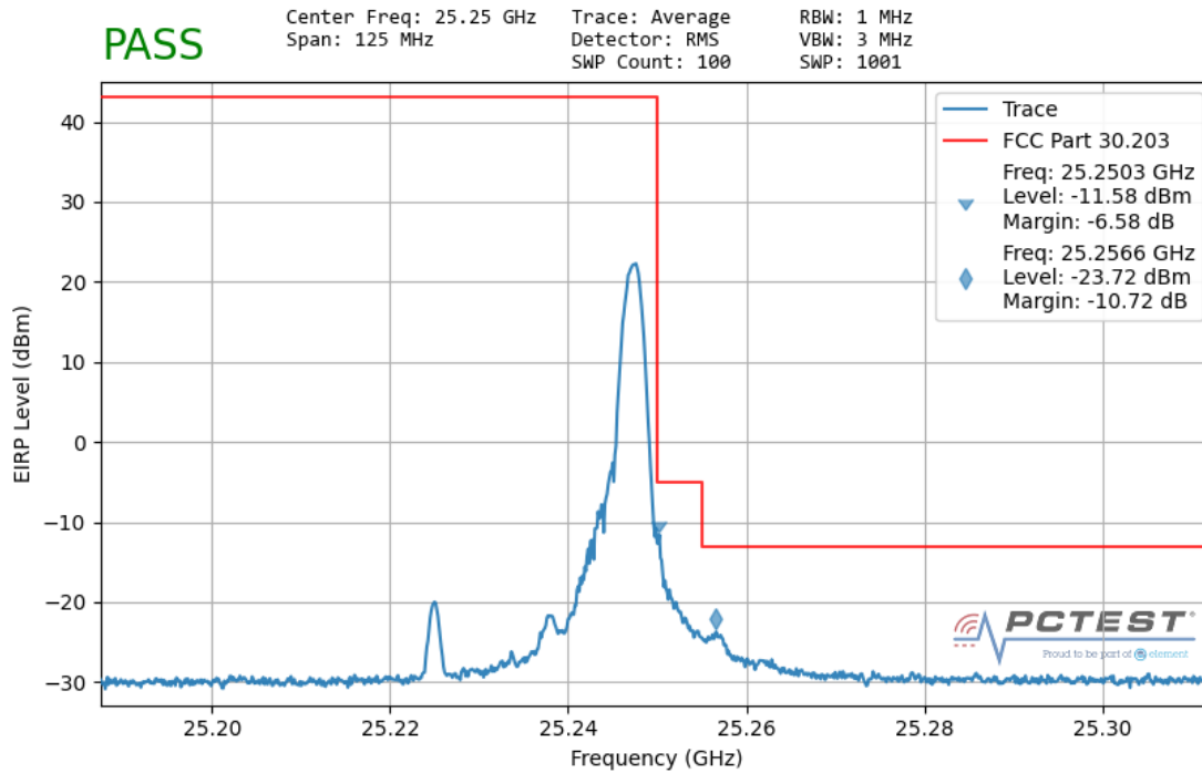
Plot 7-116. Ant1 Upper Band Edge (50MHz-1CC – \pi/2 -BPSK 1 RB)
