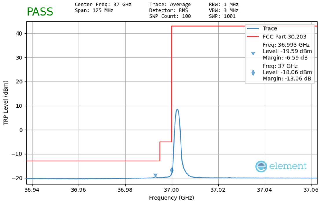
Plot 7-130. Ant1 Lower Band Edge – TRP (50MHz-1CC \pi/2 -BPSK 1 RB)
