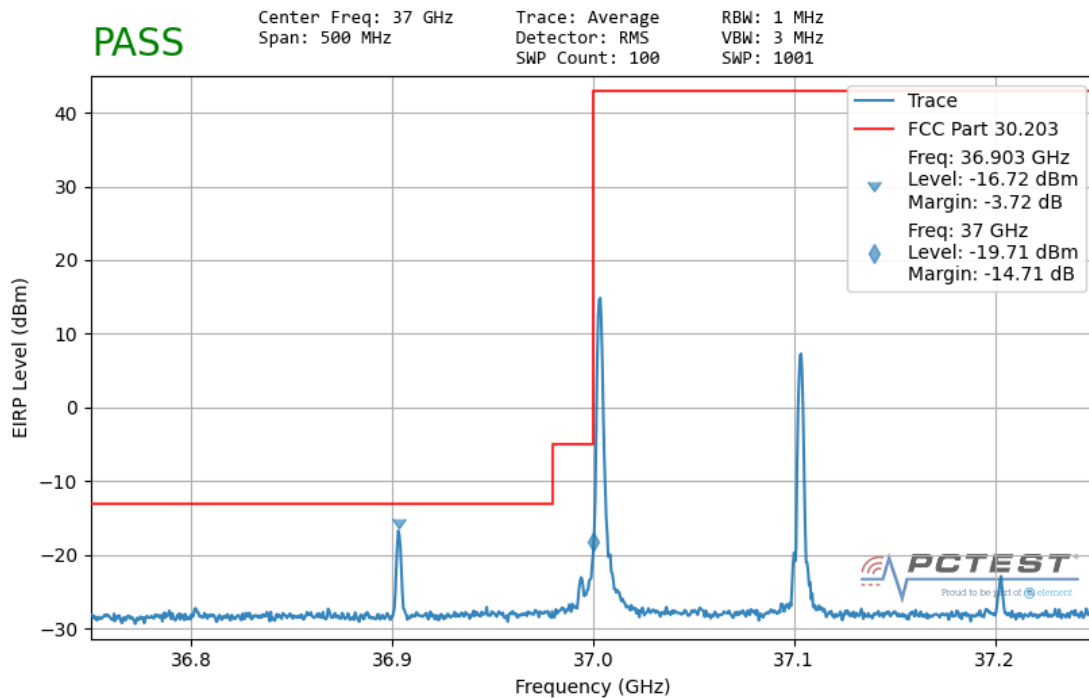
Plot 7-135. Ant1 Lower Band Edge (100MHz-2CC – QPSK 1 RB)
